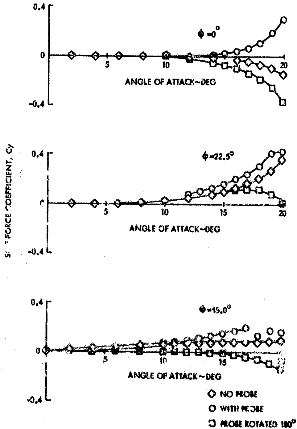
FIG. 3 SIDE FORCE COEFFICIENT VERSUS ANGLE OF ATTACK AT A MACH NUMBER OF 0.5 AND A REYNOLDS NUMBER OF 3.33 \times 10^6 PER FOOT
