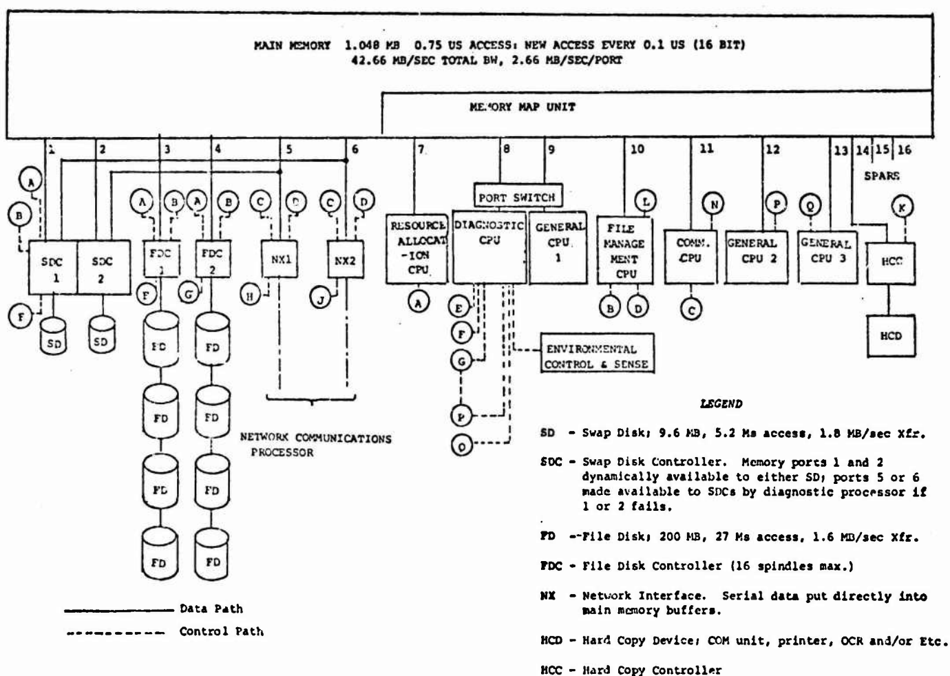
Figure 5. Host computer system.
