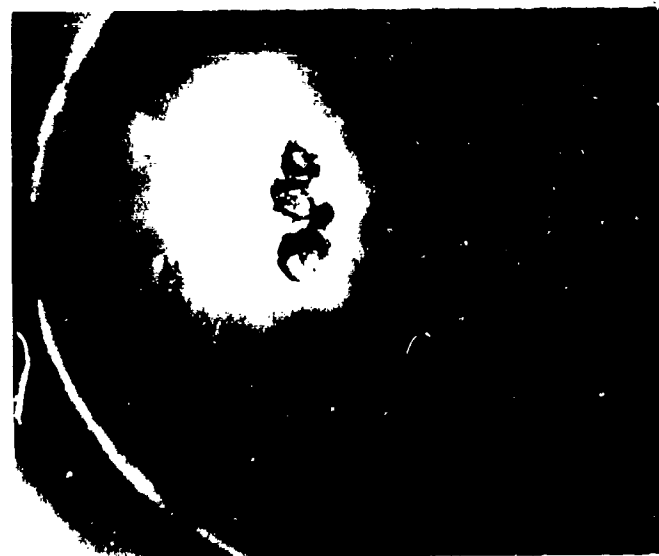
Figure 19. Spalled ball run against new 0.1 \mu\text{m} AA finish silicon nitride flat washer using DTE Medium Heavy Lube (Test #17). Note absence of visible wear band.
