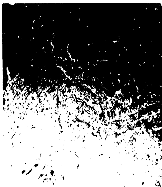
Figure 20. Surface damage in wear track on ball run against grooved silicon nitride flat washer using DTE Medium Heavy Lube (Test #19).
