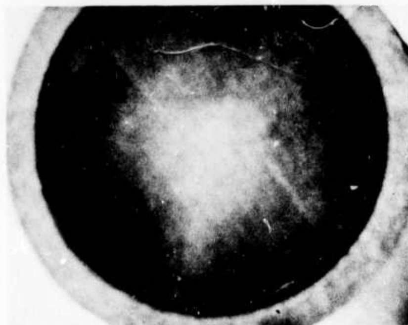
Fig. 6-16b Same After 1000°C Anneal for 10 hrs. and Cooled at 25°C/hr.
