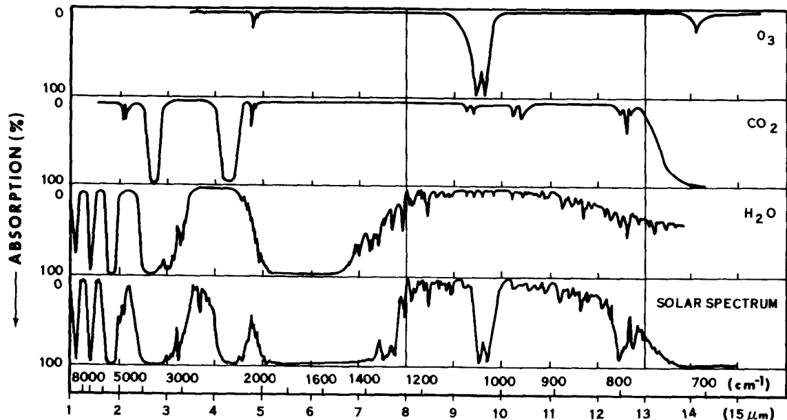
Fig 5-1. Comparison of near-infrared solar spectrum with laboratory spectra of various atmospheric gases. [7]
