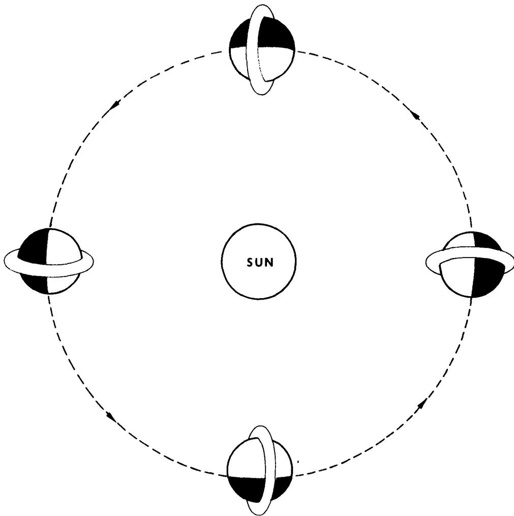
Fig 6-3. View of a sun-synchronous, local noon, near polar orbit from Polaris. Note precession of the orbital plane through 360^\circ during the year (not drawn to scale).
