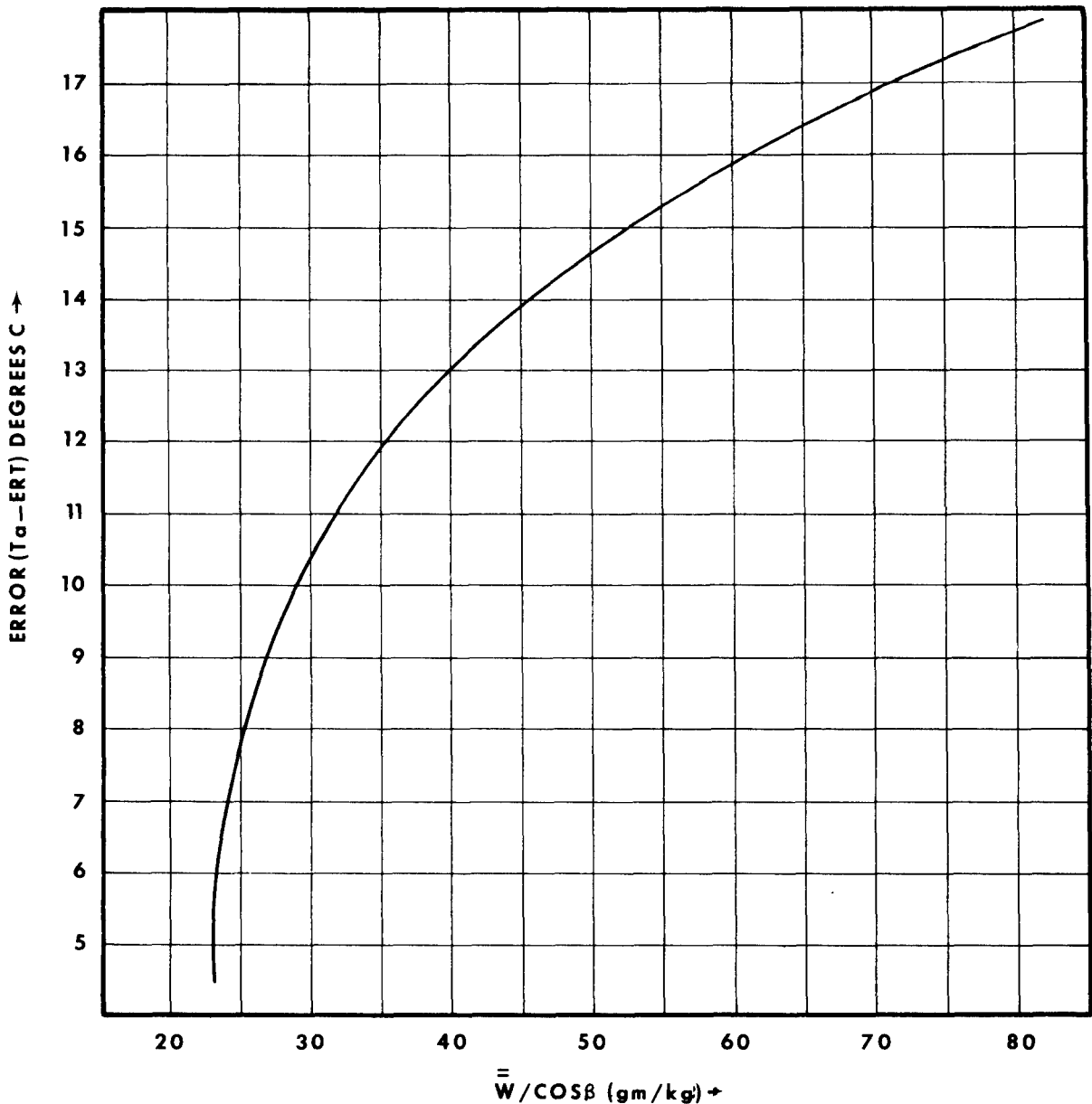
Fig 5-4. Temperature error vs moisture.
