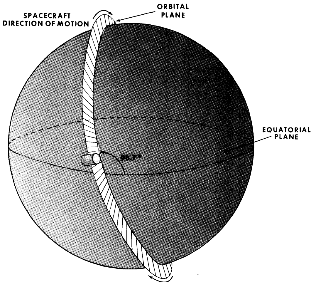
Fig 6-2. Nominal DMSP orbital inclination (not drawn to scale).
