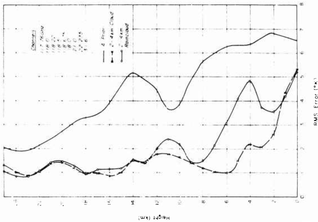
Figure 3-24 Temperature Inversion Results Using the 118 GHz Channels for Elevated 2 km Cloud and 2 km Rain Cases
