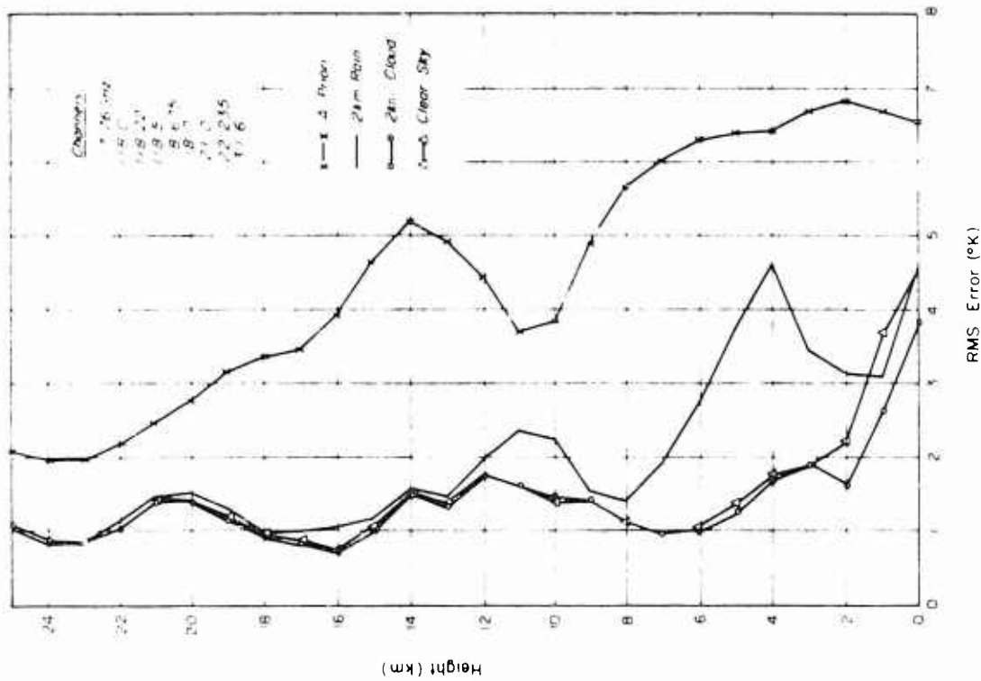
Figure 3-23 Temperature Inversion Results Using the 118 GHz Channels for Clear Sky, 2 km Cloud, and 2 km Rain Cases
