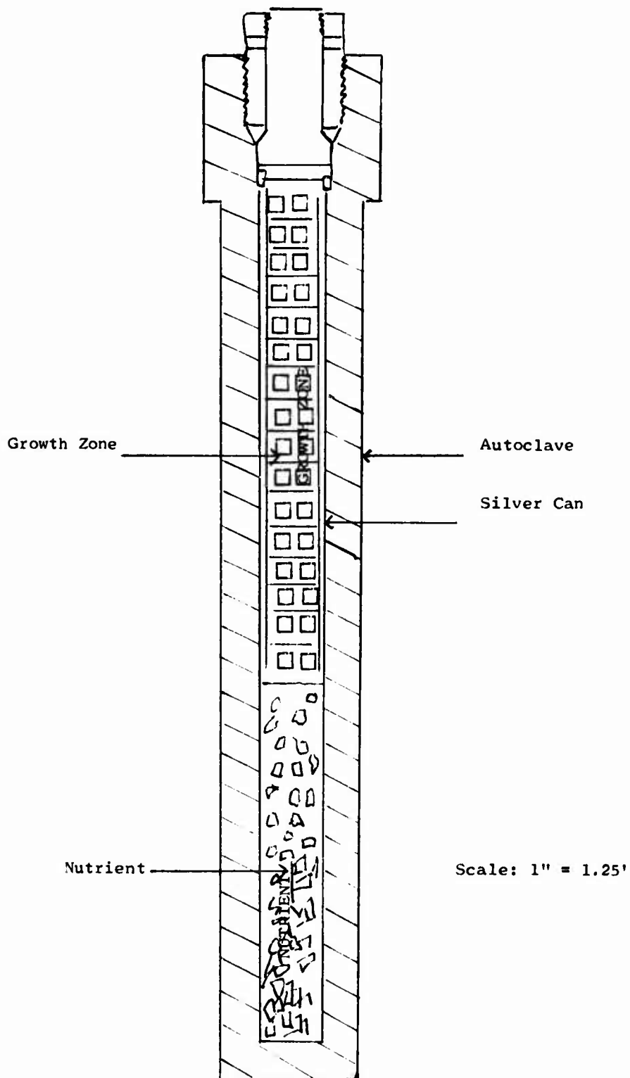
Figure 43 Nine-inch I.D. Autoclave with Silver Can in Position
