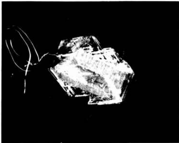
Figure 24 Growth on \{\bar{1}012\} bounded by \{\bar{1}101\} . Note rapid edgewise extension (and its preferred direction) of complementary r-face.
