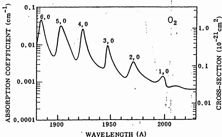
Figure C.2-2. Oxygen absorption cross-sections, Schumann-Runge bands (1, 0 to 6, 0). (Source: R-12, Figure 2)
