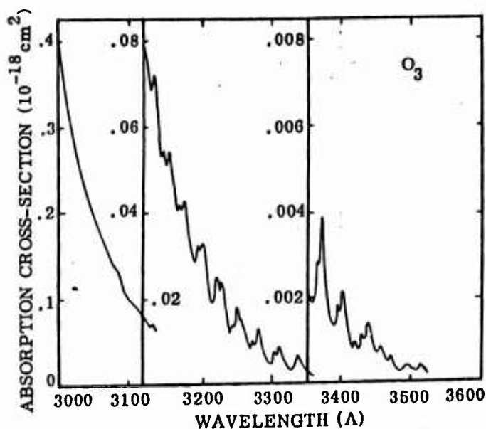
Figure B.3.a-46. Ozone cross-sections. Wavelength 3000-3600 Å. (Source: R-12, Figure 14)
