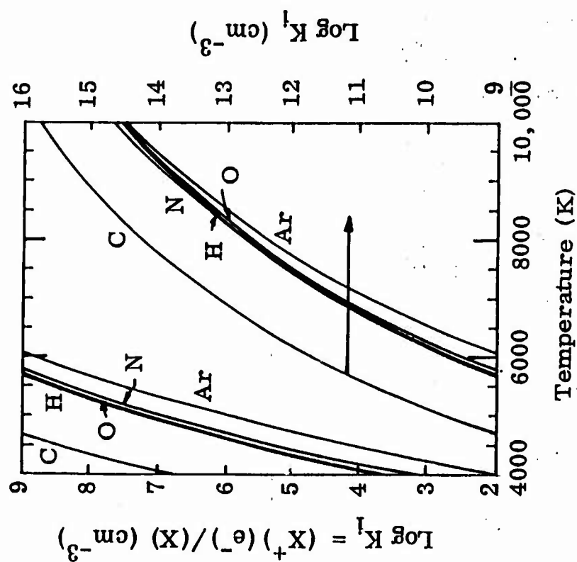
Figure B.2-1.a. Equilibrium constants for ionization of atoms. (Source: R-10, Figure 10)
