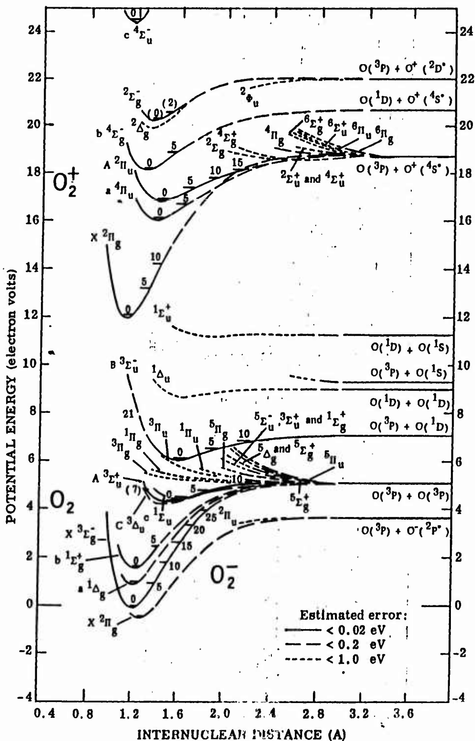
Figure B.2-9. Potential energy curves for O_2^+ , O_2 , and O_2^- . (Source: R-10, Figure 7)
