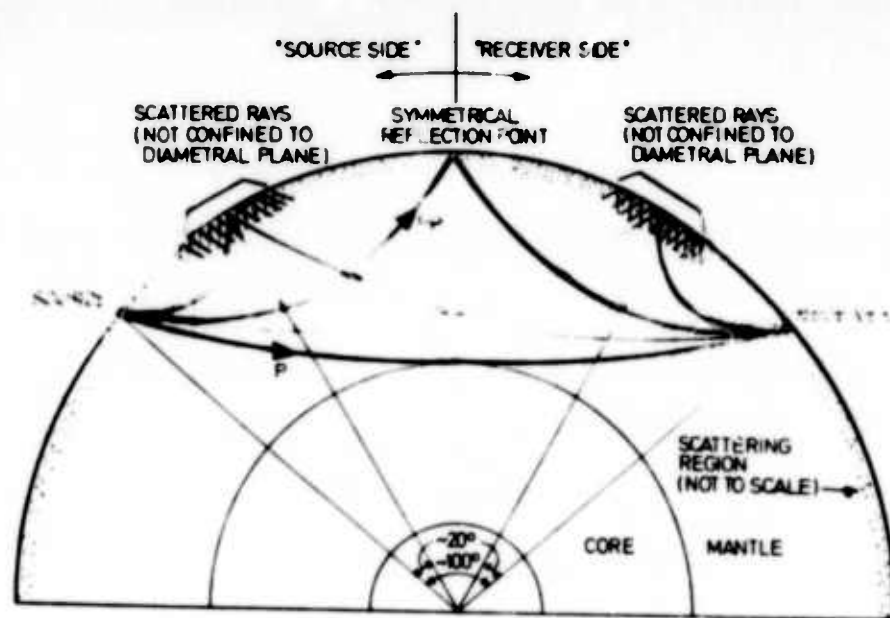
Fig. 1 Schematic diagram showing ray paths of P, PP and precursors to PP resulting from scattering by random inhomogeneities in the crust and upper mantle. The precursor paths are asymmetrical, and are not restricted to the diametral plane through source and receiver.
