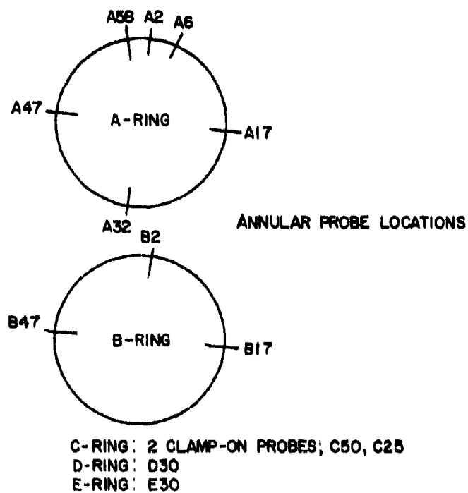
Figure 11. Electrostatic Probe Locations in Turbine Exhaust
