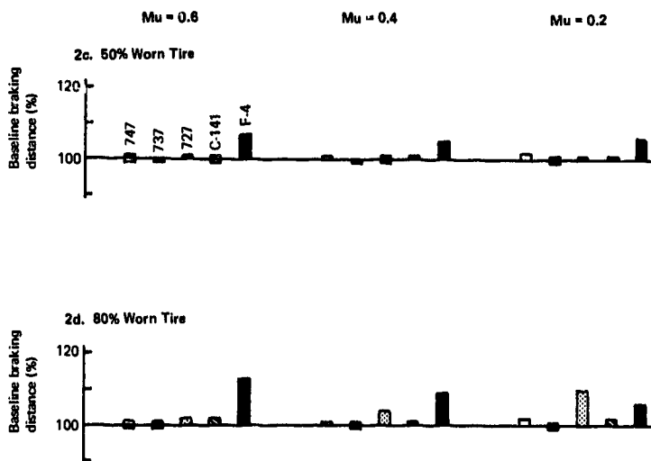
Figure 10.—Braking Distance Test Results (Sheet 11 of 15)
