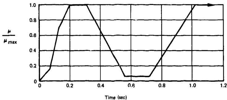
Figure B-3.—Touchdown Profile
