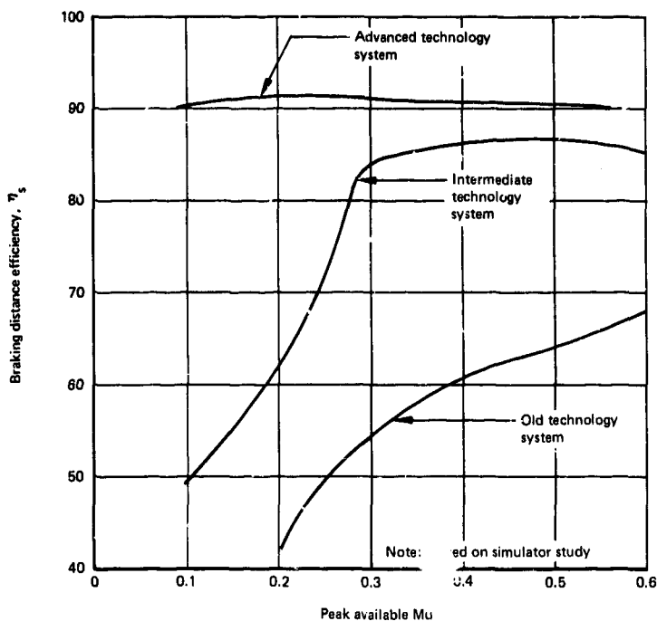
Figure 25.—Mu-Efficiency Curves
