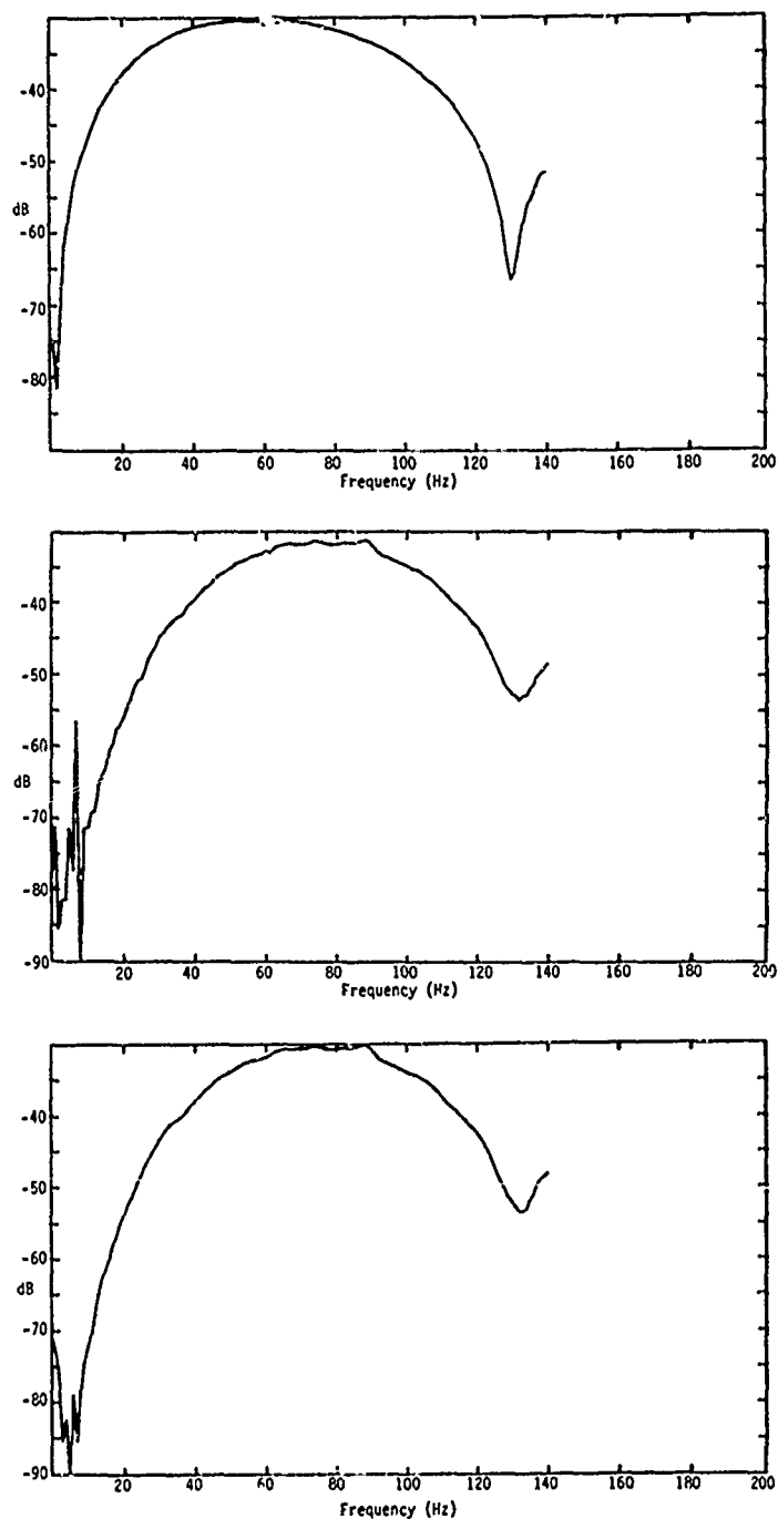
Fig. 13. Energy spectra obtained in calibration experiments using one cycle of 65-Hz signal. Top: relative spectrum, J13 current. Middle: relative spectrum, F50 response. Bottom: relative spectrum, F37 response.
