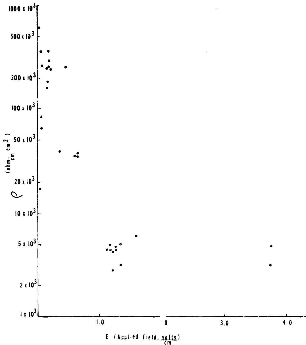
Figure 17 Resistivity vs. Applied Field
