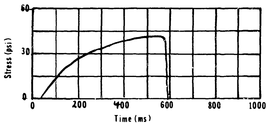
Figure 58: Stress vs. Time - Air Tests 31, 32 and 34
