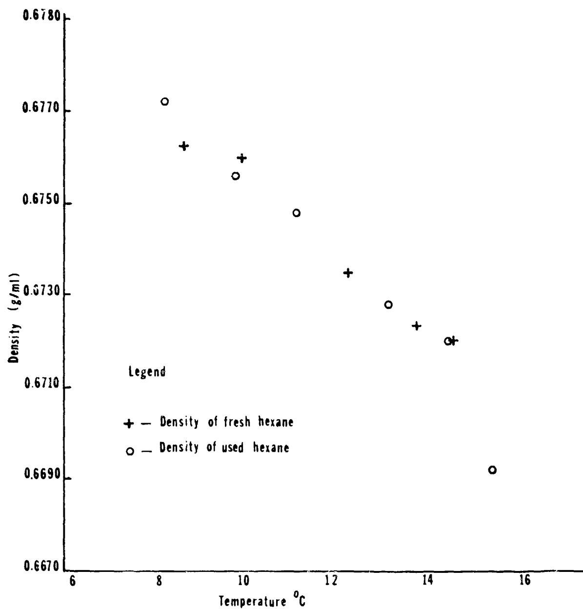
Figure 4 Hexane Density vs. Temperature
