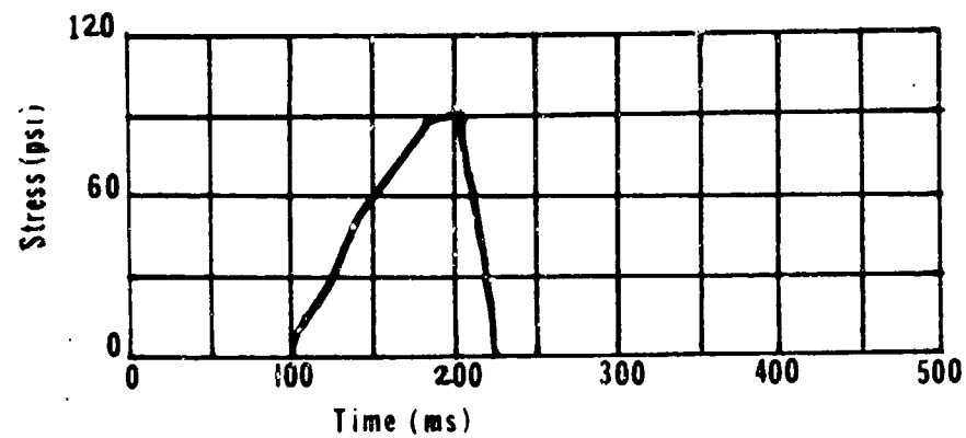
Figure 65: Stress vs. Time - Drop Weight Tests 22,23, and 24 - 24/sec
