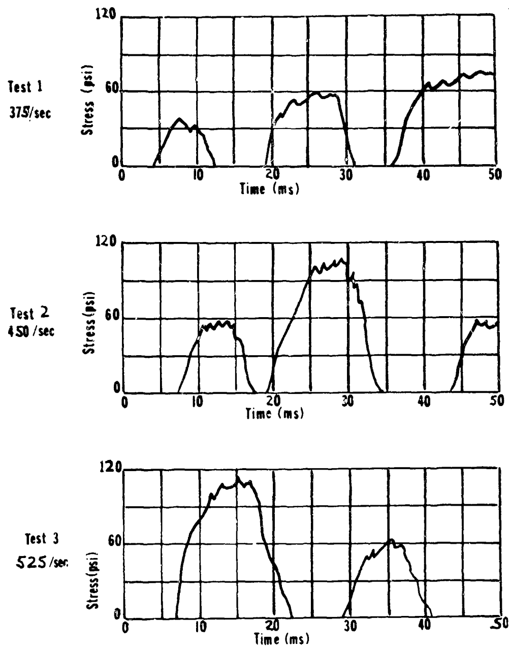
Figure 71: Stress vs. Time - Gun Tests 1,2 and 3
