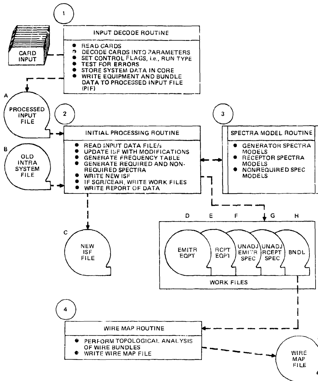
FIGURE 1 (Concluded) IDIPR SECTION OF IEMCAP TOP LEVEL FUNCTIONAL FLOW (Part 2 of 2)
