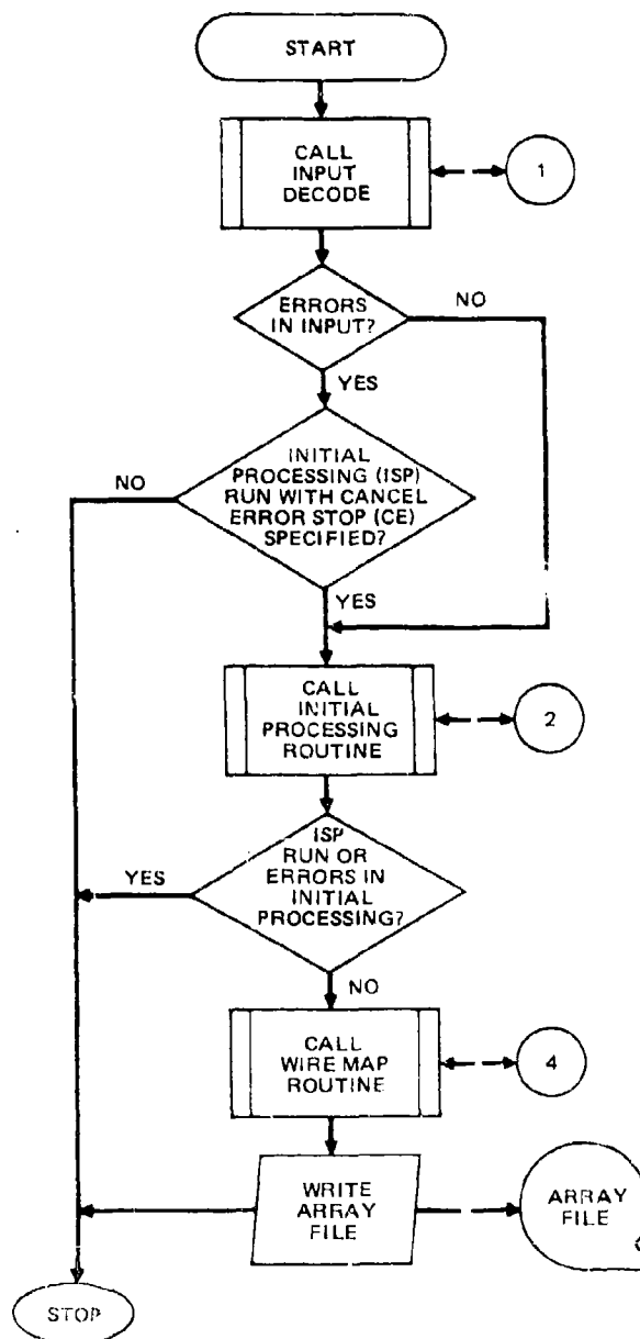
FIGURE 1 IDIPR SECTION OF IEMCAP TOP LEVEL FUNCTIONAL FLOW (Part 1 of 2)
