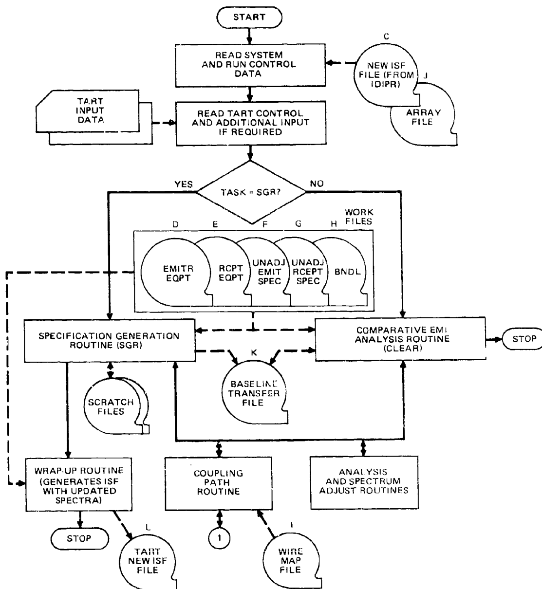
FIGURE 2 TART SECTION OF IEMCAP TOP LEVEL FUNCTIONAL FLOW (Part 1 of 2)
