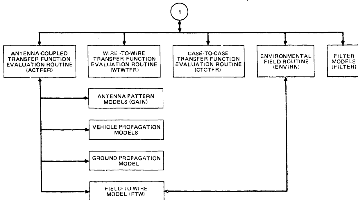
FIGURE 2 (Concluded) PART SECTION OF IEMCAP TOP LEVEL FUNCTIONAL FLOW (Part 2 of 2)
