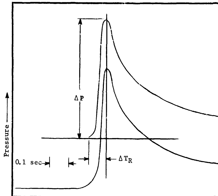
Zero-Delay Ignition Pressure Trace
