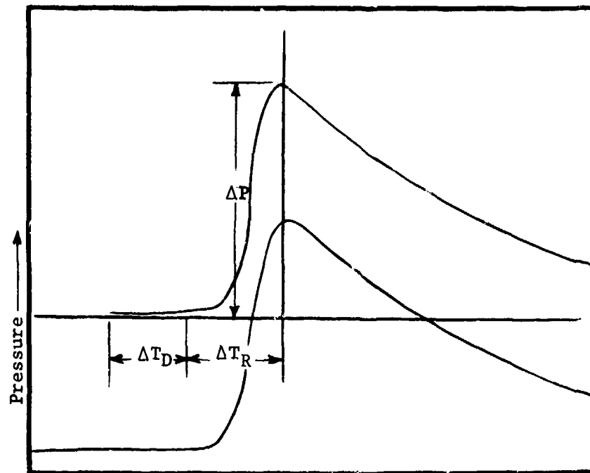
Delayed Ignition Pressure Trace
