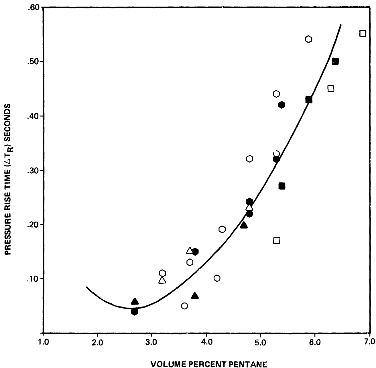
FIGURE 12. AVERAGE TIME TO PEAK OVERPRESSURE VS PERCENT PENTANE.
