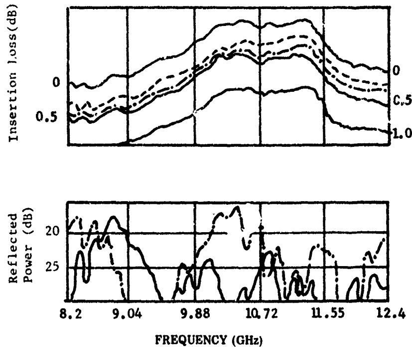
Fig. AII-3 — Insertion loss and return loss as a function of frequencies
