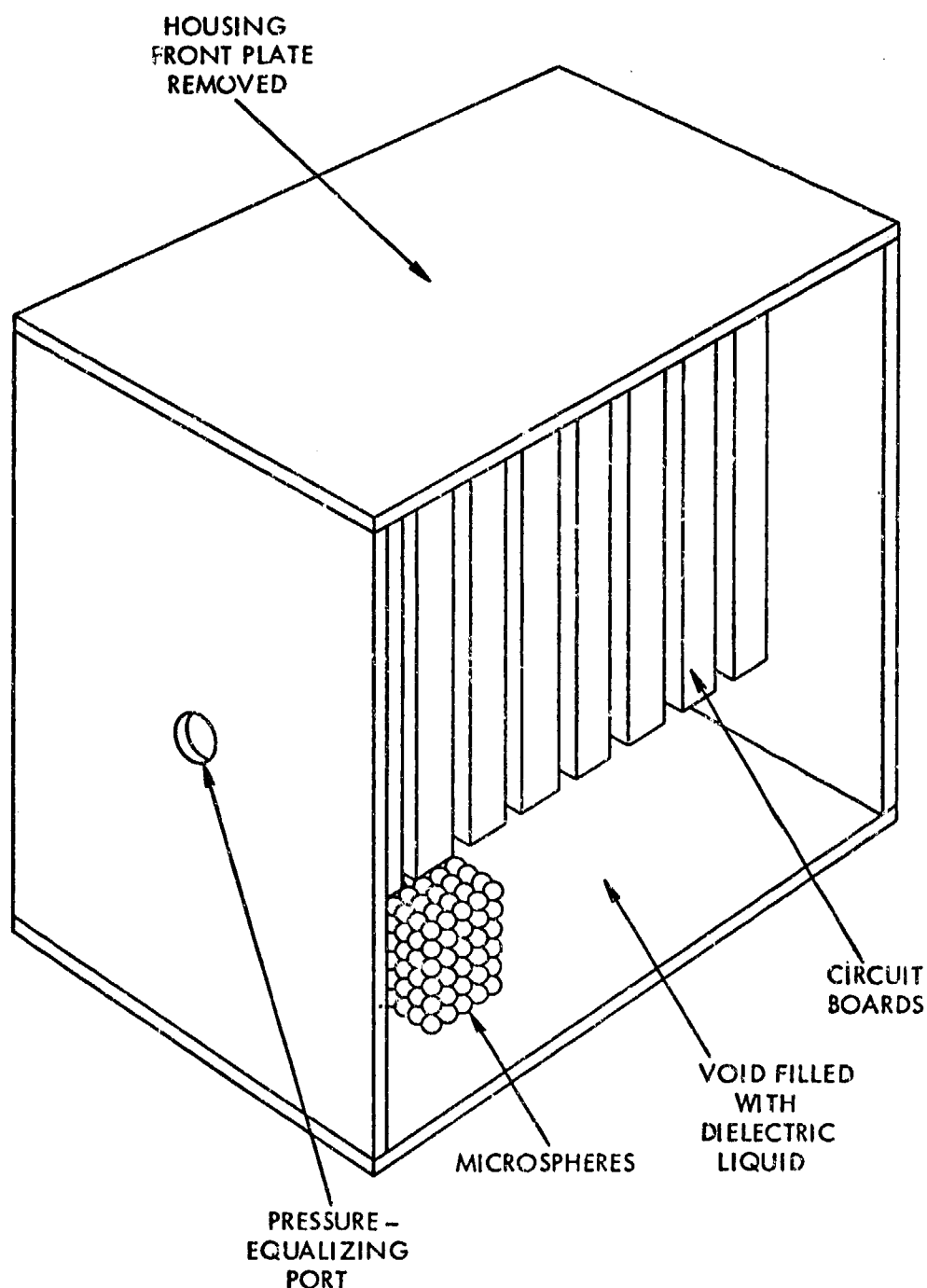
Figure 10 - System Concept
