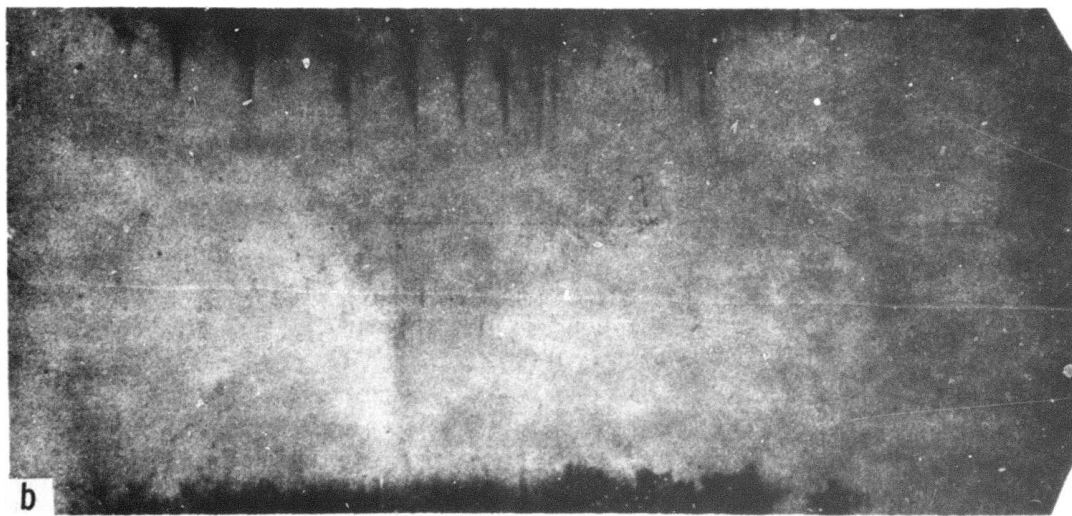
Fig. 11. X-ray topographs (recorded on x-ray film due to large size) of large slabs after heat treatment. Note perfection resulting through use of closed boat.
