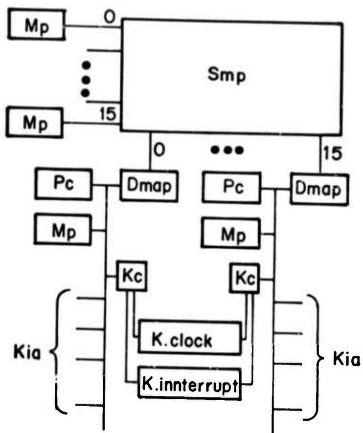
Figure 1: C.mmp Architecture
