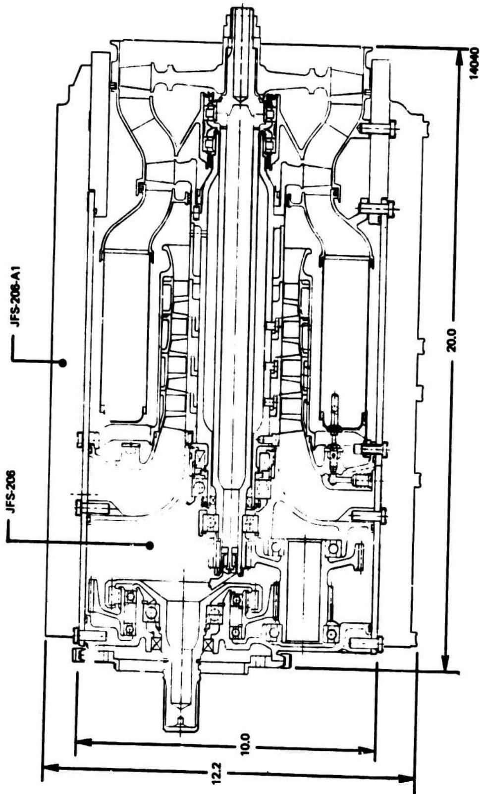
Figure 24. Comparison of JFS206 Baseline with JFS206-A1 Alternate.
