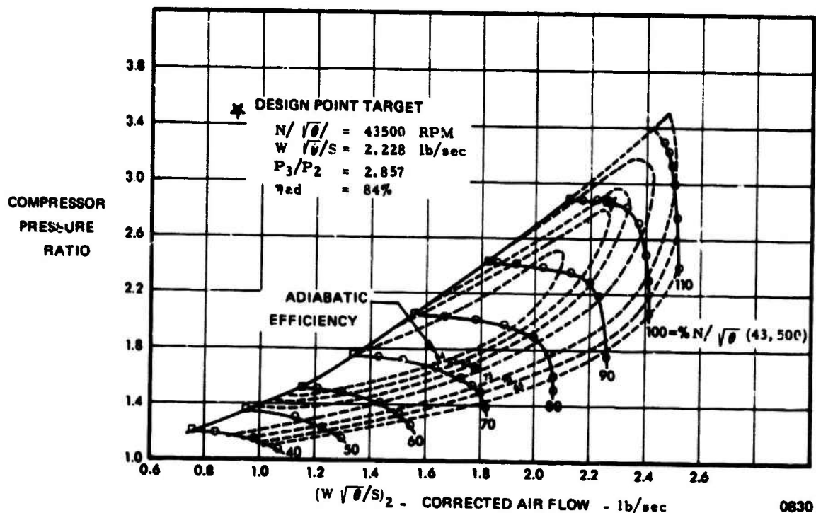
Figure 3. Compressor Performance Map Developed From Rig Testing
