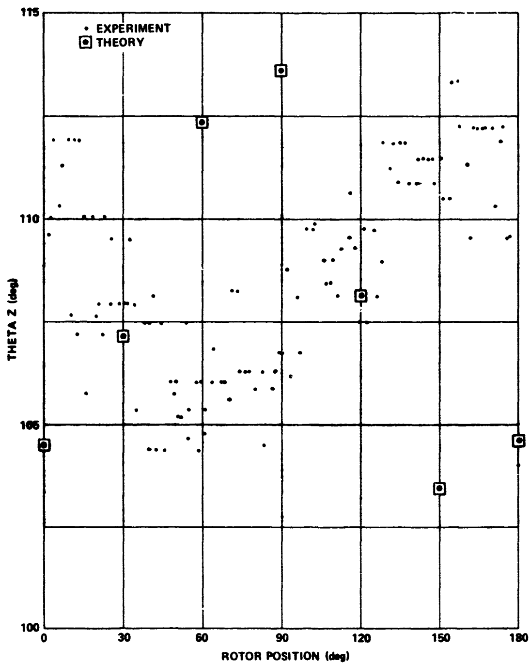
Figure 52. Folded comparison - flight record 10, sensor No. 1, and trial period 0.093500.
