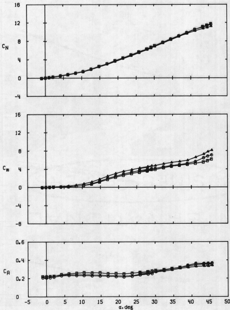
b. M_\infty = 2.00 Figure 8. Continued.
