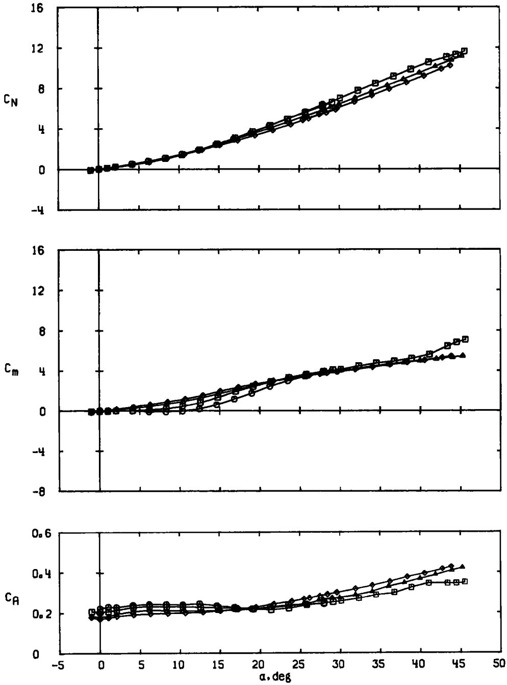
b. Configuration B*T1-5, delta fin, AR = 1.0, S_T = 7.023 \text{ in.}^2 Figure 14. Continued.
