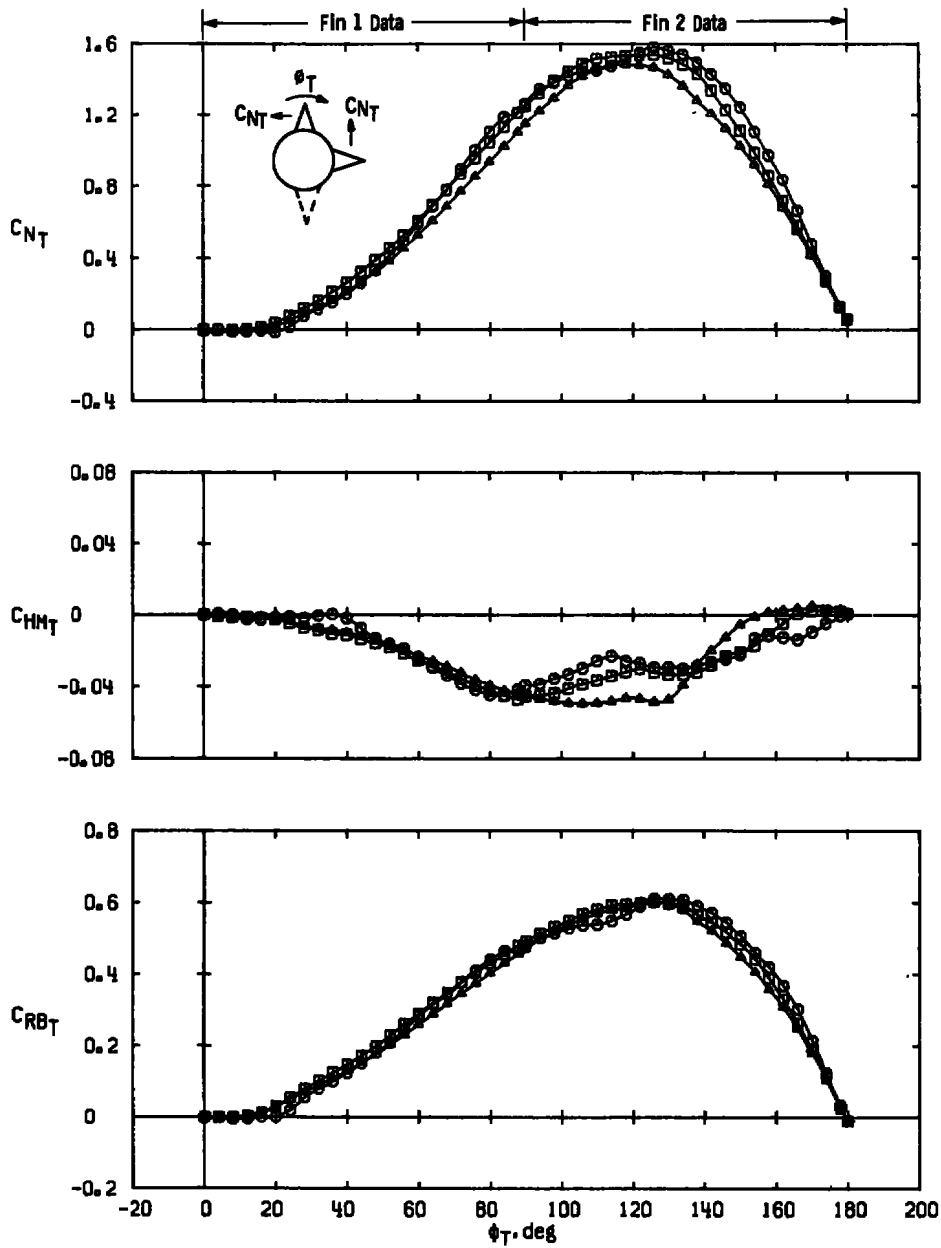
d. a \approx 43 deg Figure 27. Concluded.
