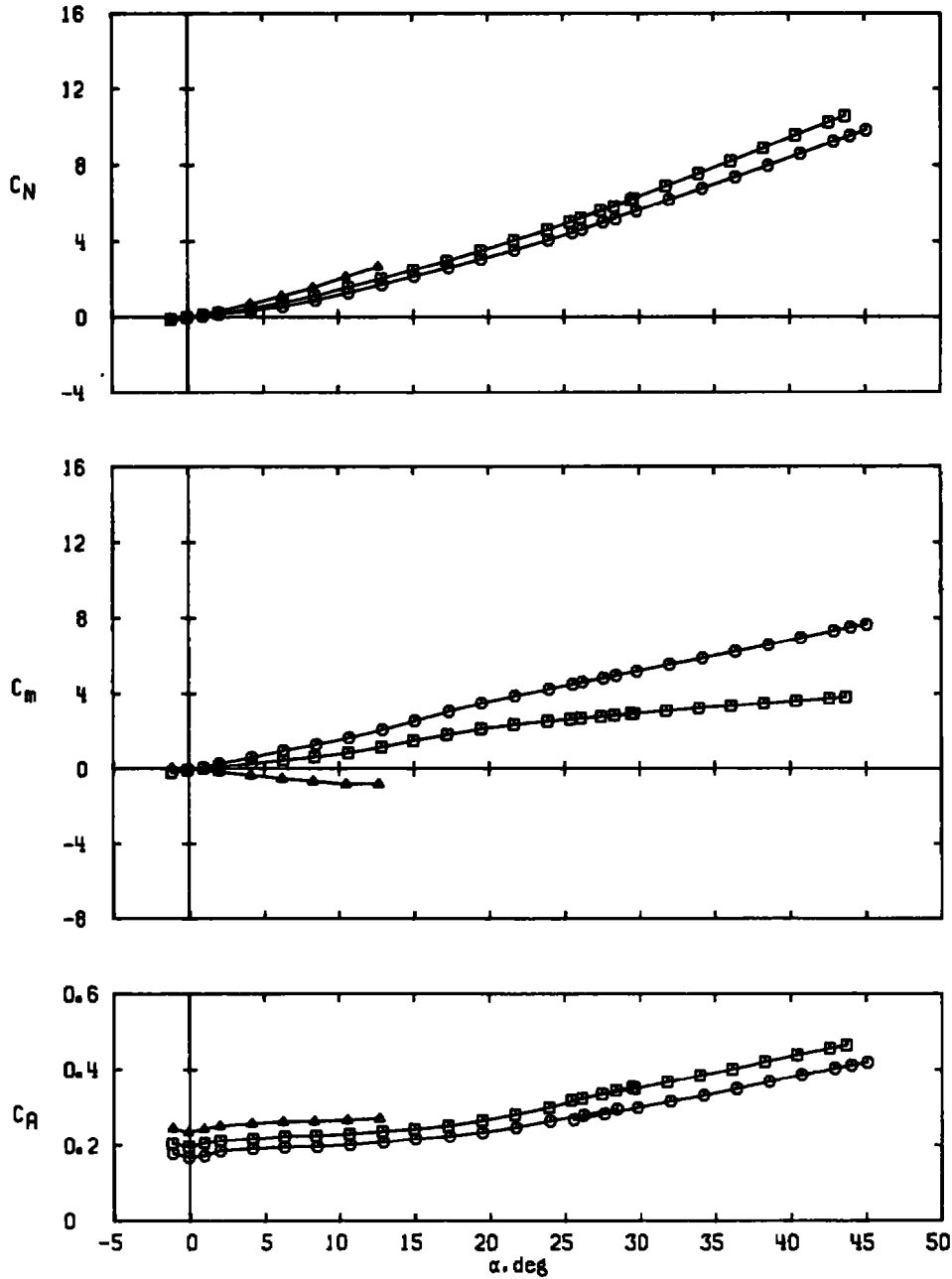
d. M_\infty = 3.01 Figure 10. Concluded.
