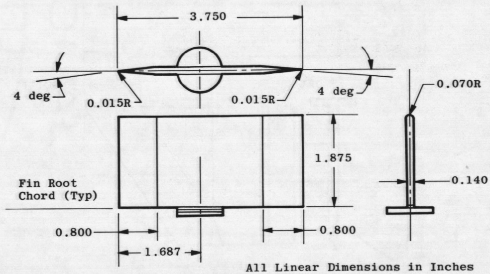
a. Fin T1-1 Figure 4. Fin details.
