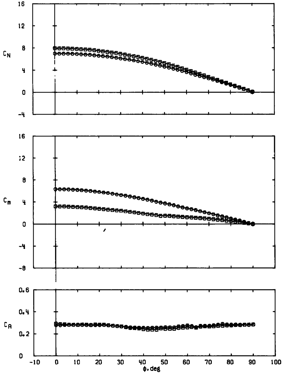
c. a \approx 32 deg Figure 19. Concluded.
