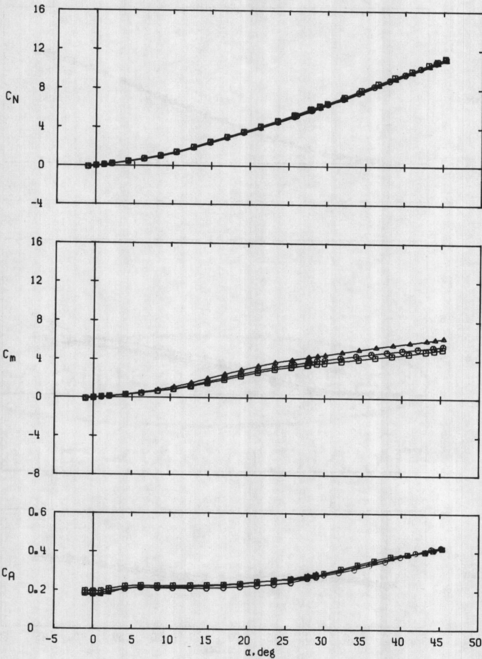
c. M_\infty = 2.50 Figure 8. Continued.
