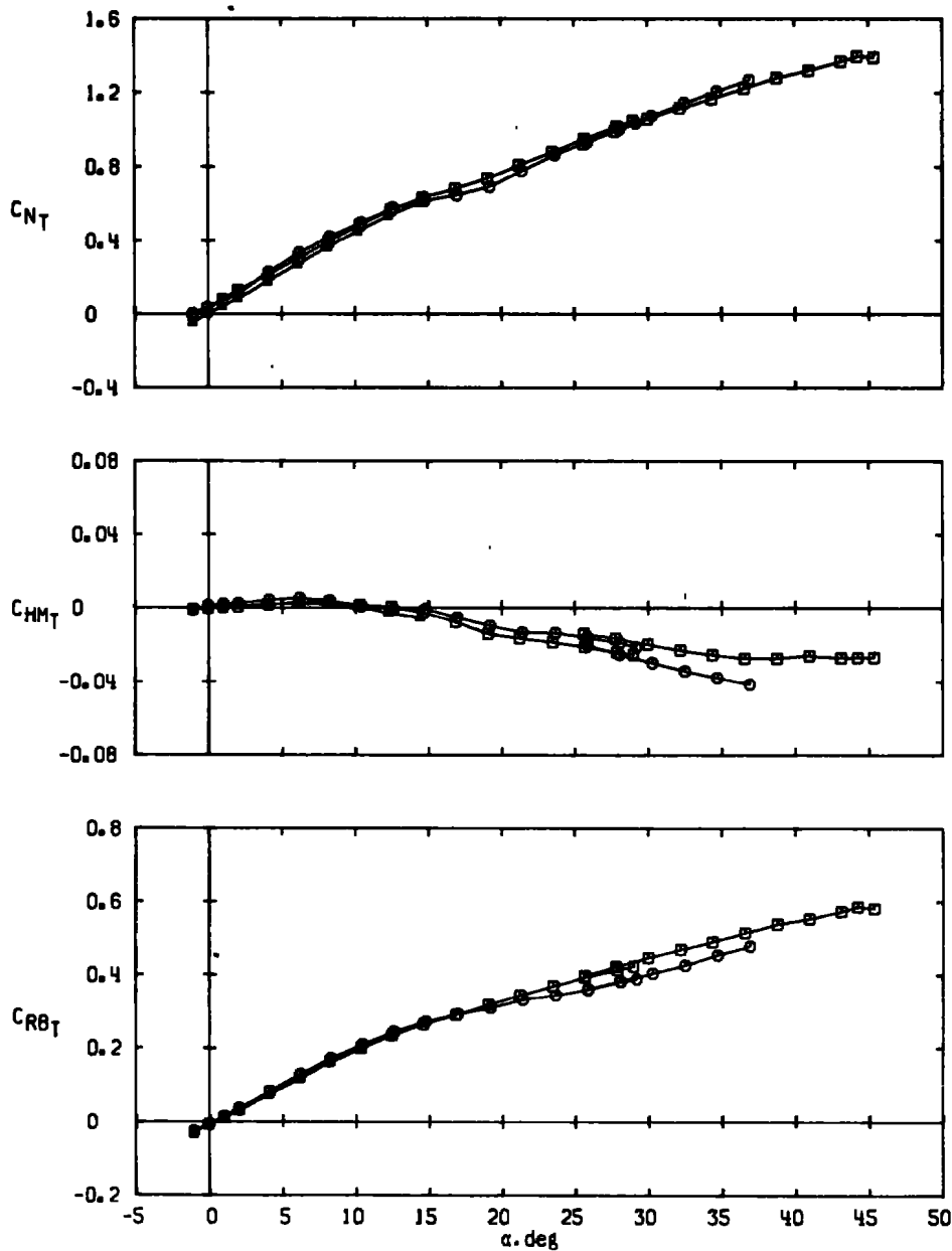
b. M_\infty = 2.00 Figure 11. Continued.
