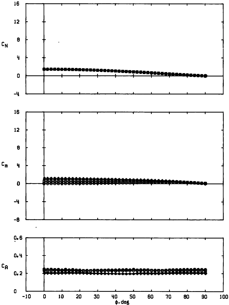
Figure 25. Variations in missile normal-force, pitching-moment, and axial-force coefficients with roll angle at different Mach numbers for a delta fin configuration (B*T1-5) of aspect ratio 1.0.
