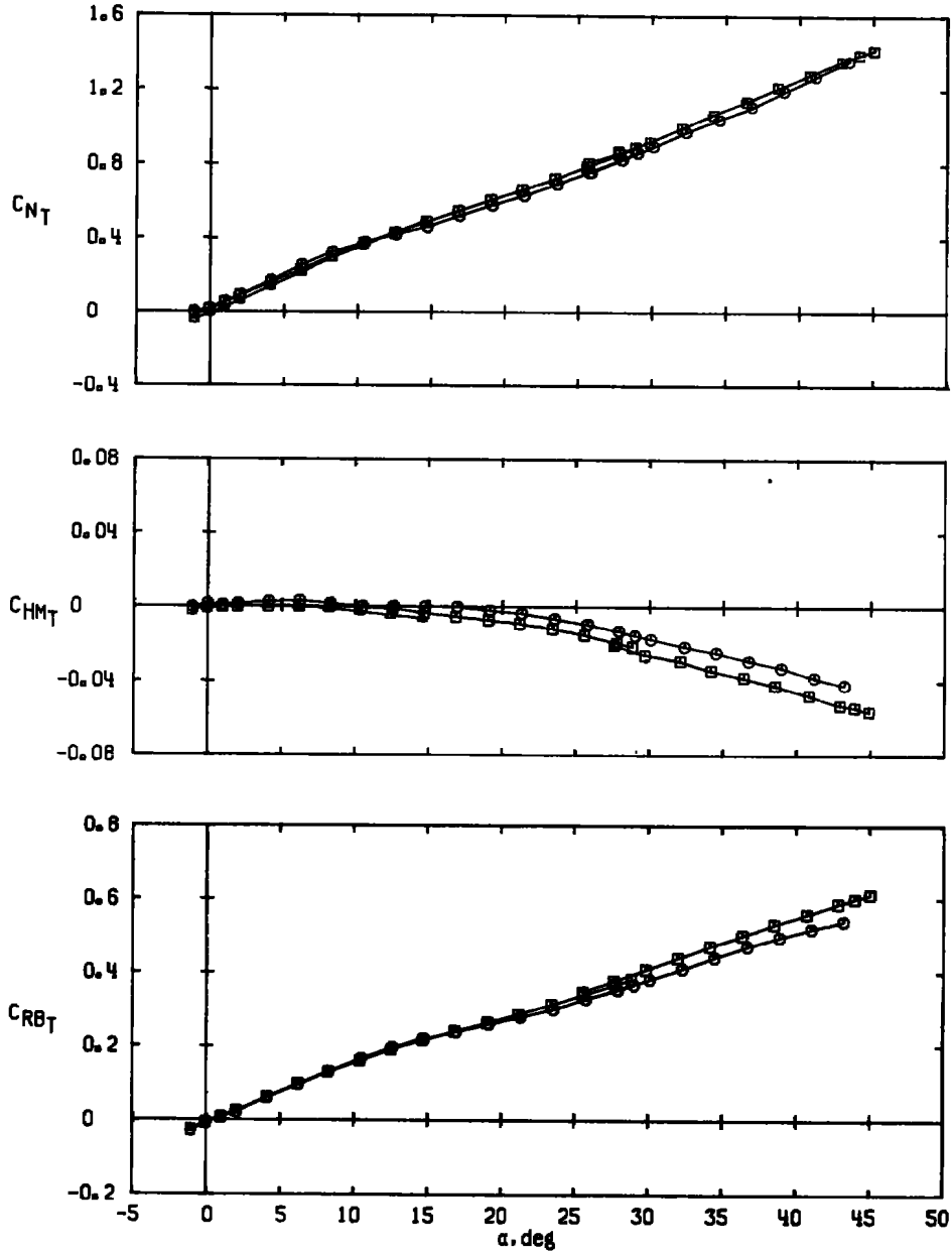
c. M_\infty = 2.50 Figure 11. Continued.
