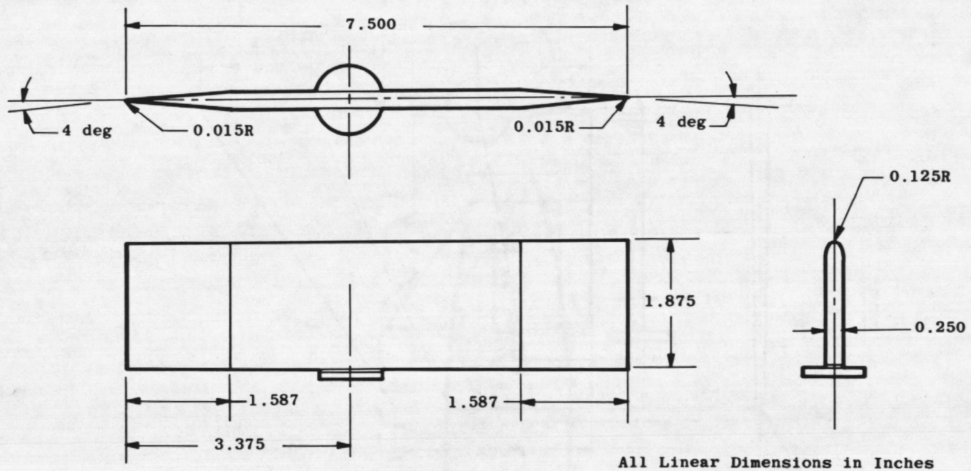
g. Fin T3-2 Figure 4. Continued.
