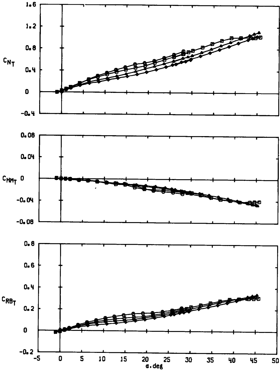
c. Configuration B*T1-4, triangular fin, S_T = 7.031 \text{ in.}^2 Figure 15. Concluded.
