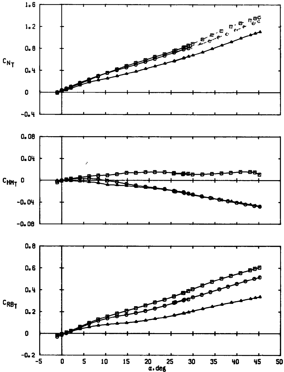
c. M_\infty = 2.50 Figure 9. Continued.
