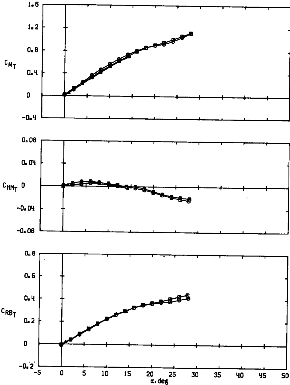
Figure 11. Effect of delta fin platform area on fin aerodynamic characteristics for aspect ratio 2.0 fins, \phi = 0 .
