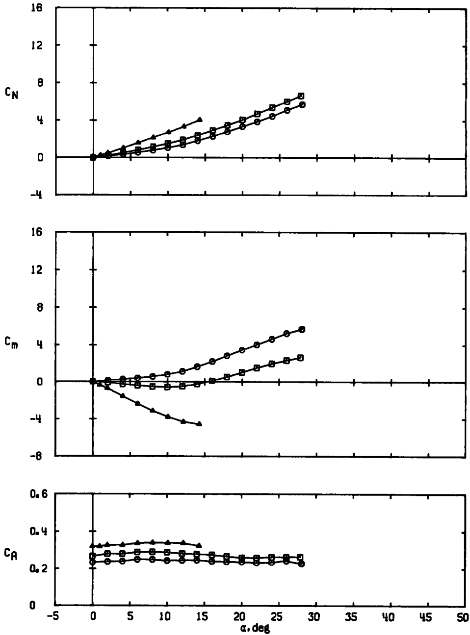
Figure 10. Effect of delta fin planform area on missile longitudinal stability and axial-force characteristics for aspect ratio 2.0 fins, \phi = 0 .
