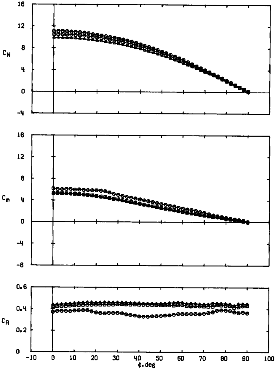
d. \alpha \approx 43 \text{ deg} Figure 25. Concluded.
