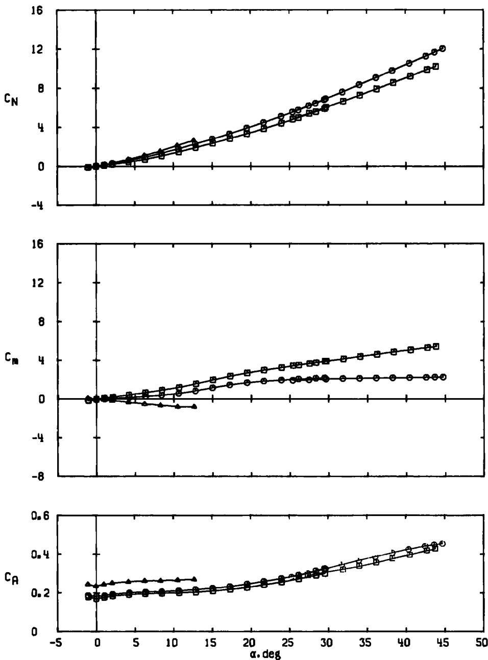
d. M_\infty = 3.01 Figure 12. Concluded.
