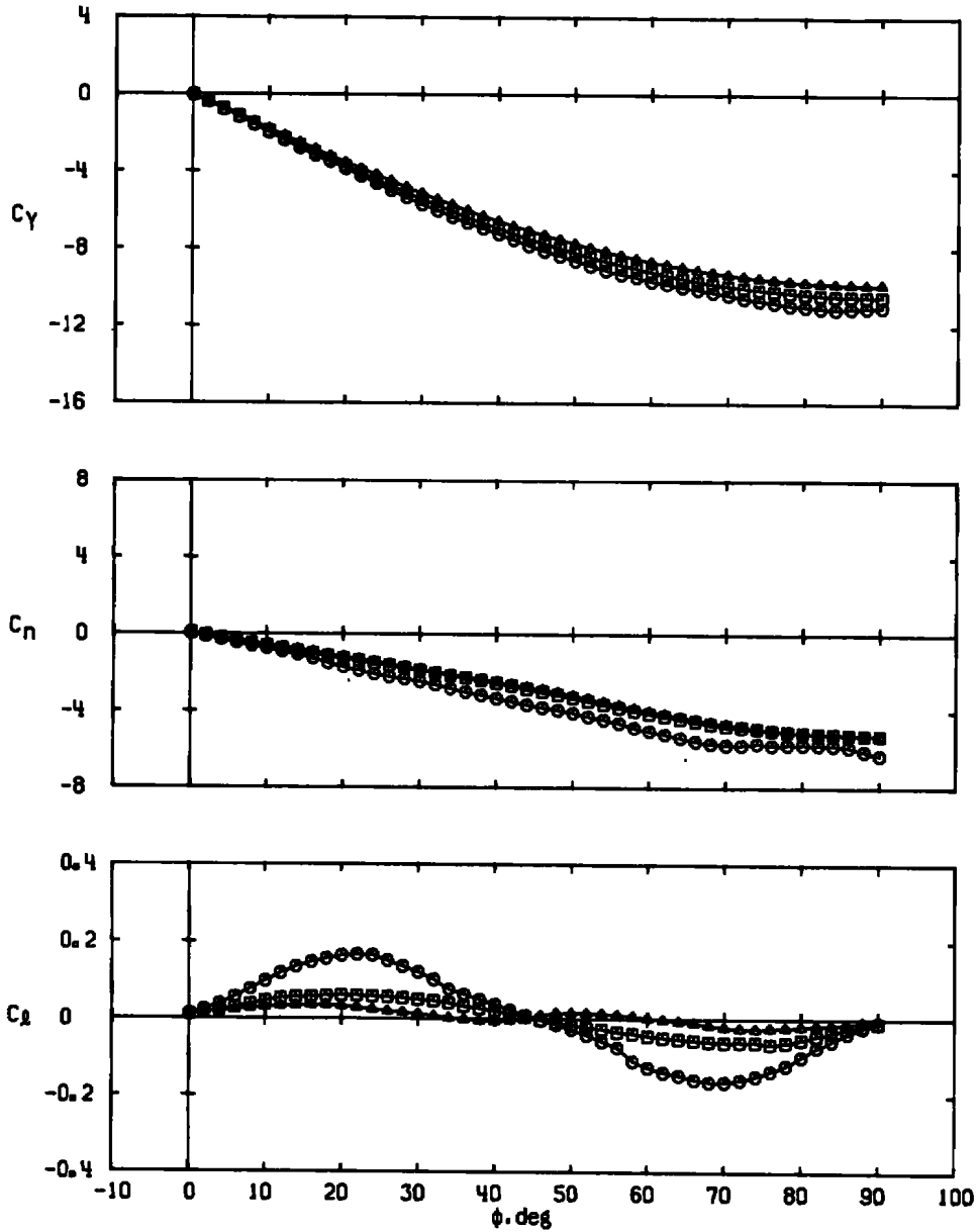
d. \alpha \approx 43 deg Figure 26. Concluded.
