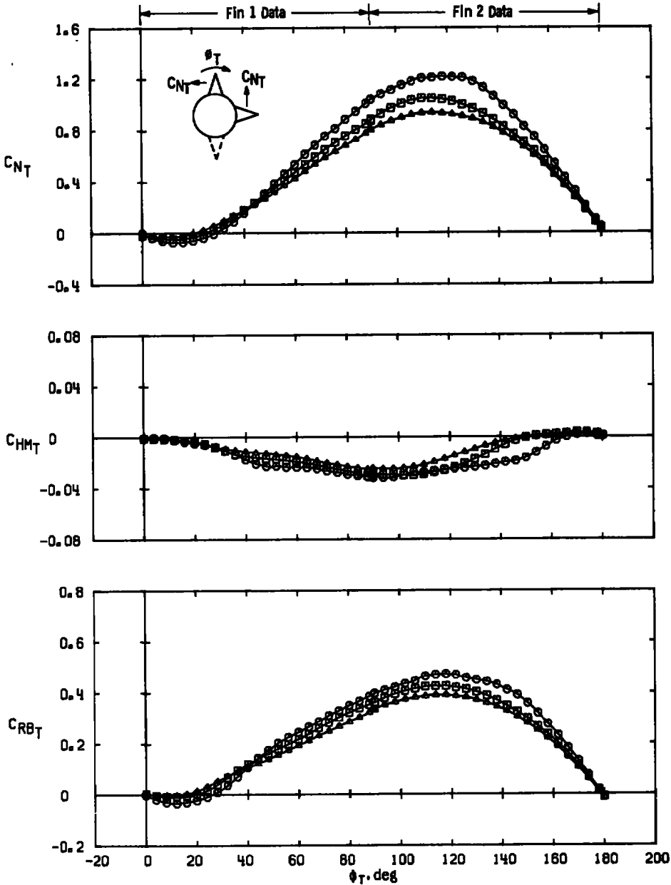
c. a \approx 32 deg Figure 27. Continued.
