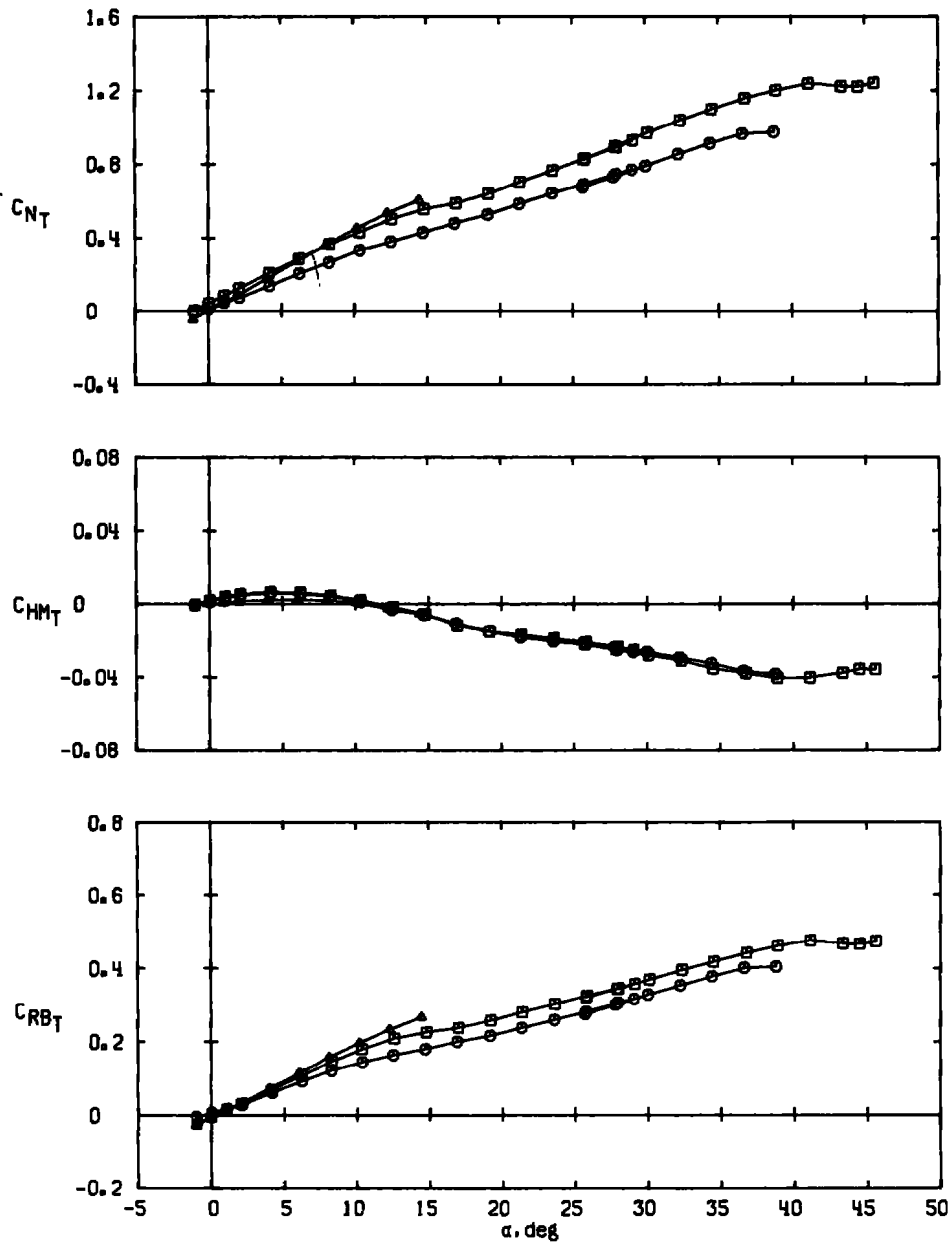
b. M_\infty = 2.00 Figure 13. Continued.
