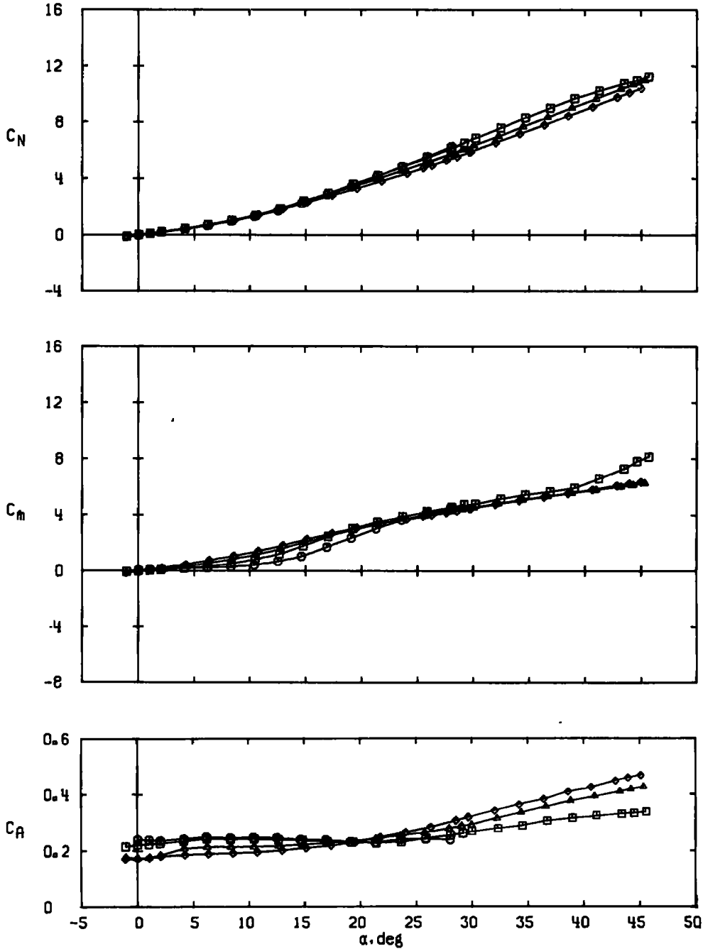
d. Configuration B*T1-4, triangular fin, AR = 1.0, S_T = 7.031 \text{ in.}^2 Figure 14. Concluded.
