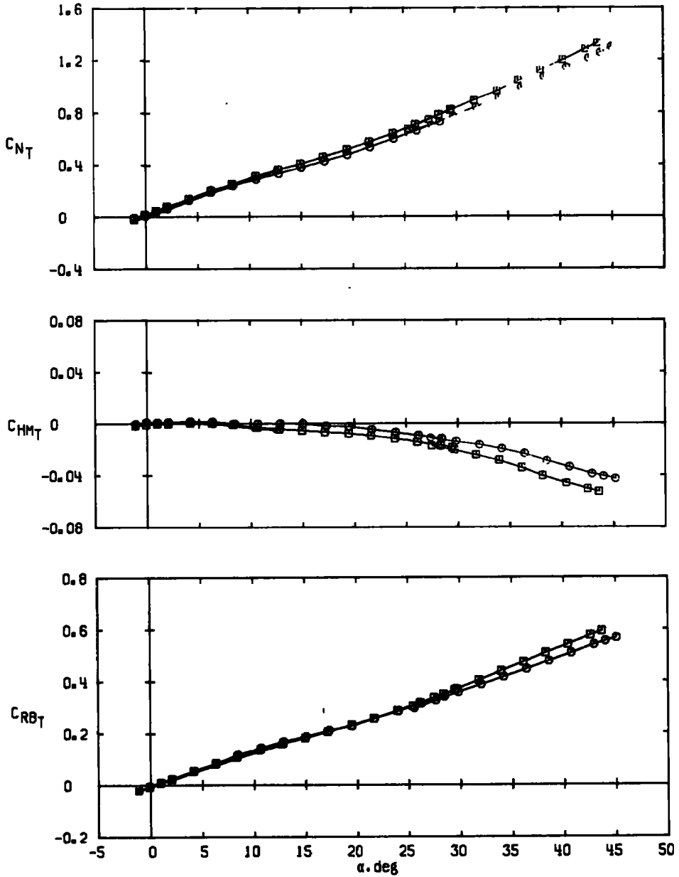
d. M_\infty = 3.01 Figure 11. Concluded.
