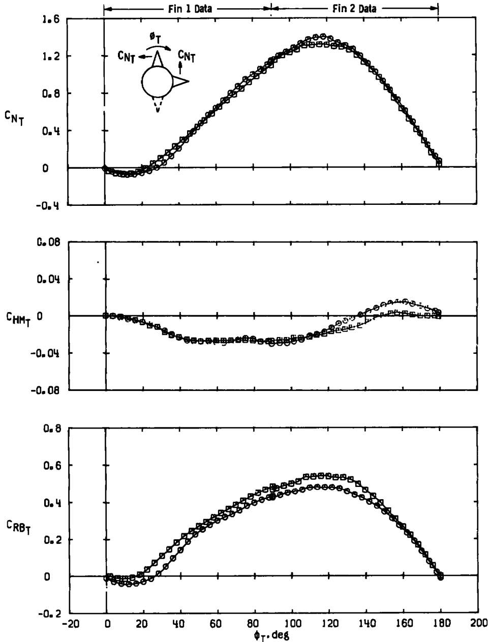
c. \alpha \approx 32 deg Figure 21. Concluded.
