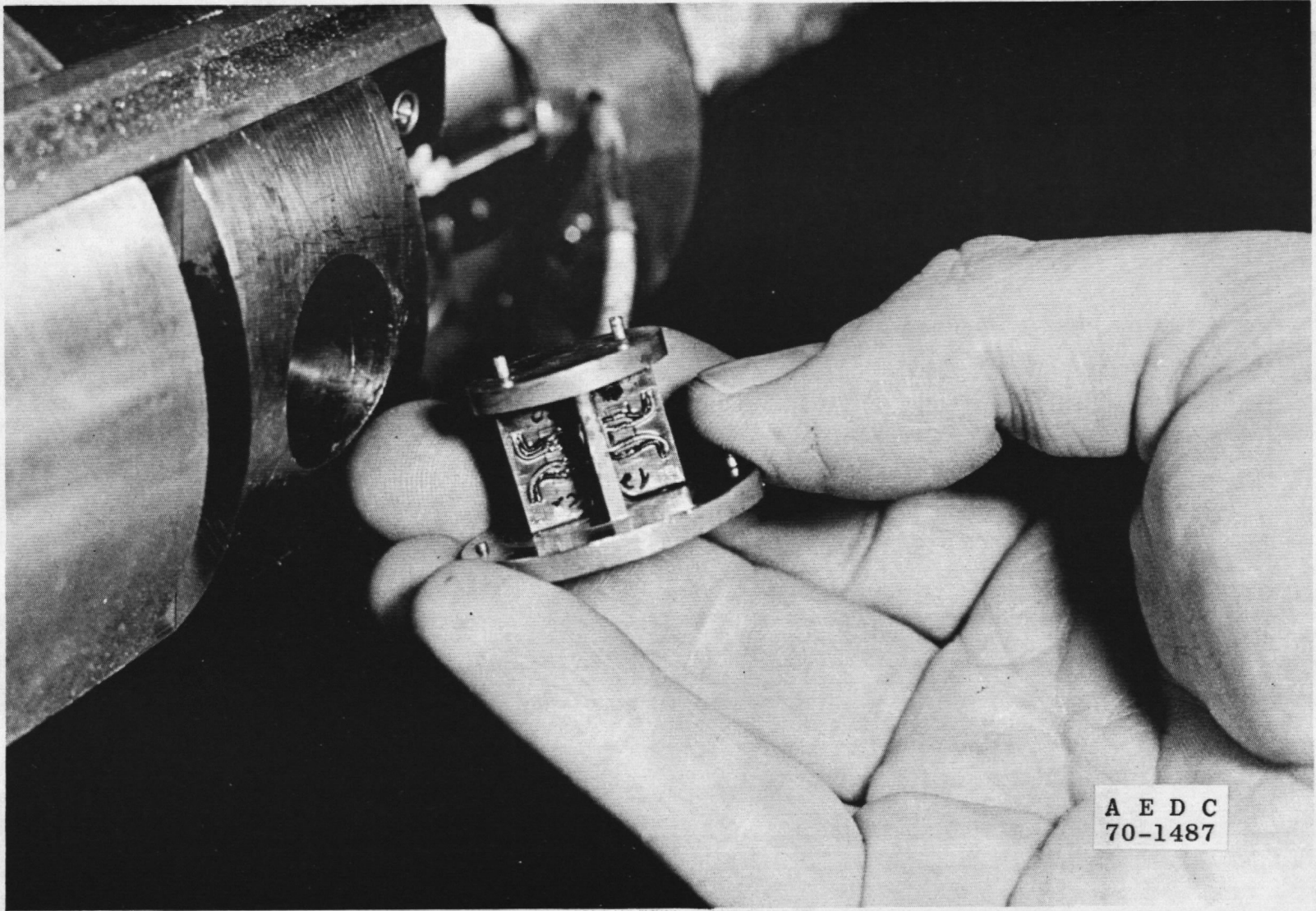
Figure 6. Photograph of fin balance.
