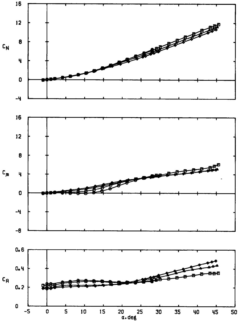
c. Configuration B*T1-1, rectangular fin, AR = 1.0, S_T = 7.031 \text{ in.}^2 Figure 14. Continued.
