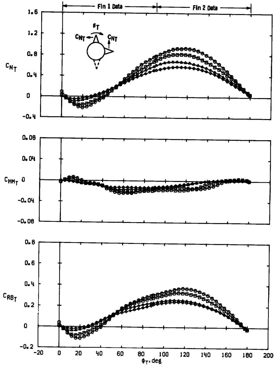
b. a \approx 21 deg Figure 27. Continued.
