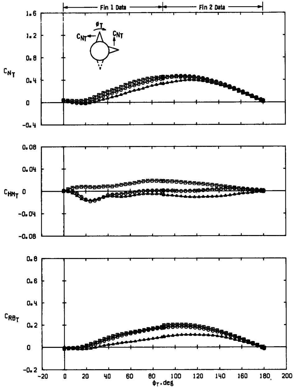
Figure 18. Variations in fin normal-force, hinge-moment, and bending-moment coefficients with fin roll position for different fin planform shapes of aspect ratio 1.0, M_\infty = 2.00 .
