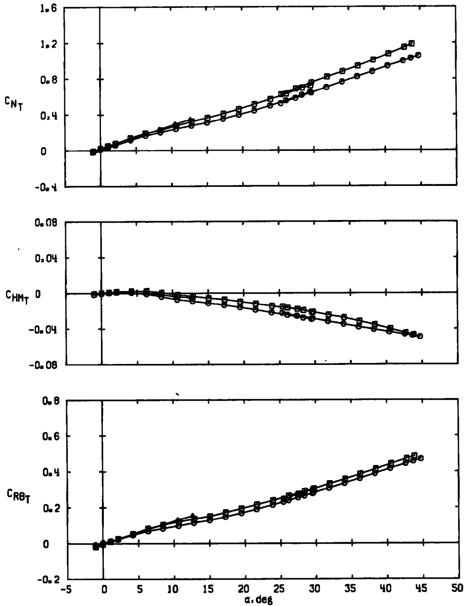
d. M_\infty = 3.01 Figure 13. Concluded.
