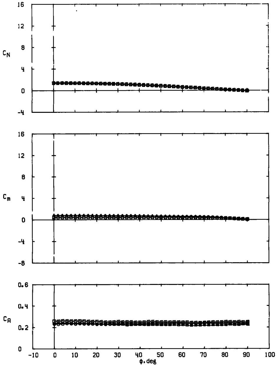
Figure 16. Variations in missile normal-force, pitching-moment, and axial-force coefficients with roll angle for different fin planform shapes of aspect ratio 1.0, M_\infty = 2.00 .
