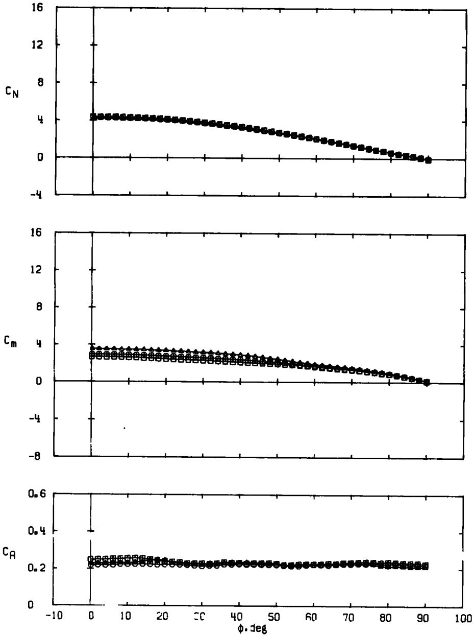
b. a \approx 21 deg Figure 16. Continued.
