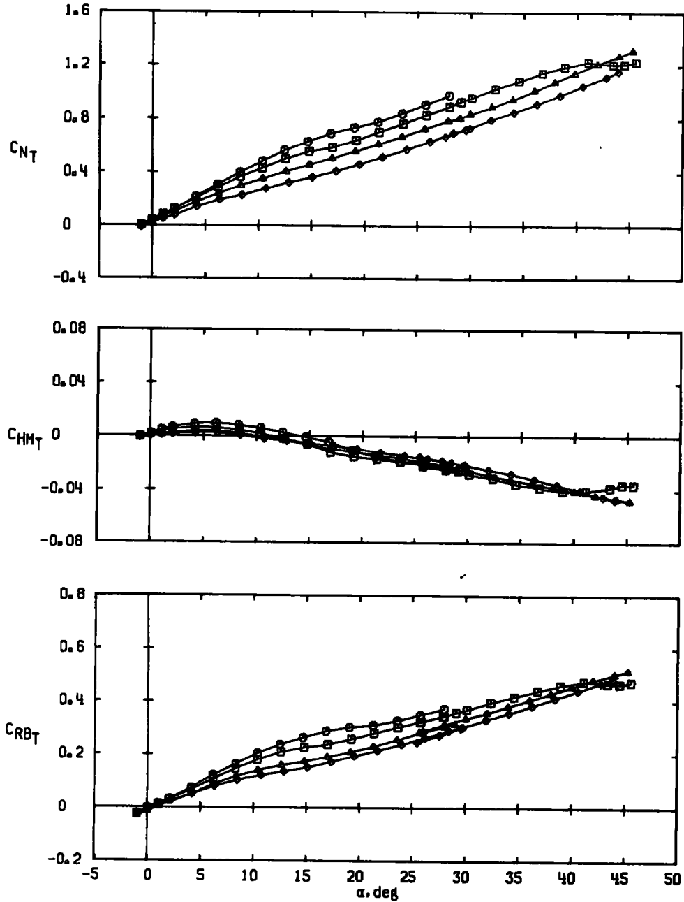
a. Configuration B*T1-5, delta fin, S_T = 7.023 \text{ in.}^2 Figure 15. Effect of Mach number on fin aerodynamic characteristics for aspect ratio 1.0 fins, \phi = 0 .
