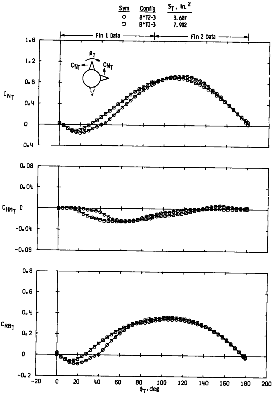
b. a \approx 21 deg Figure 21. Continued.
