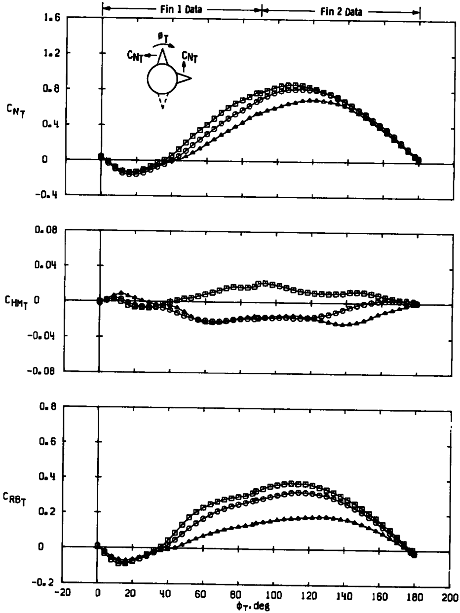
b. a \approx 21 deg Figure 18. Continued.
