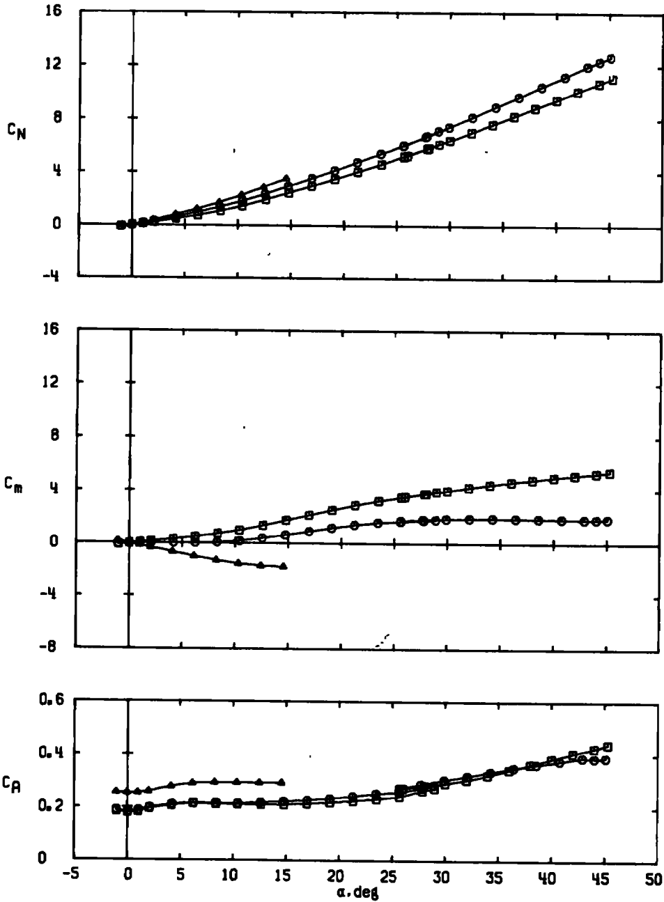
c. M_\infty = 2.50 Figure 12. Continued.
