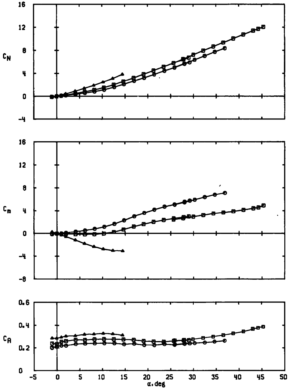
b. M_\infty = 2.00 Figure 10. Continued.
