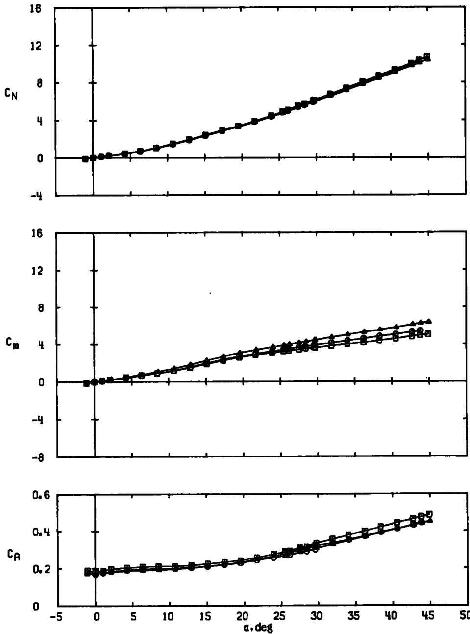
d. M_\infty = 3.01 Figure 8. Concluded.
