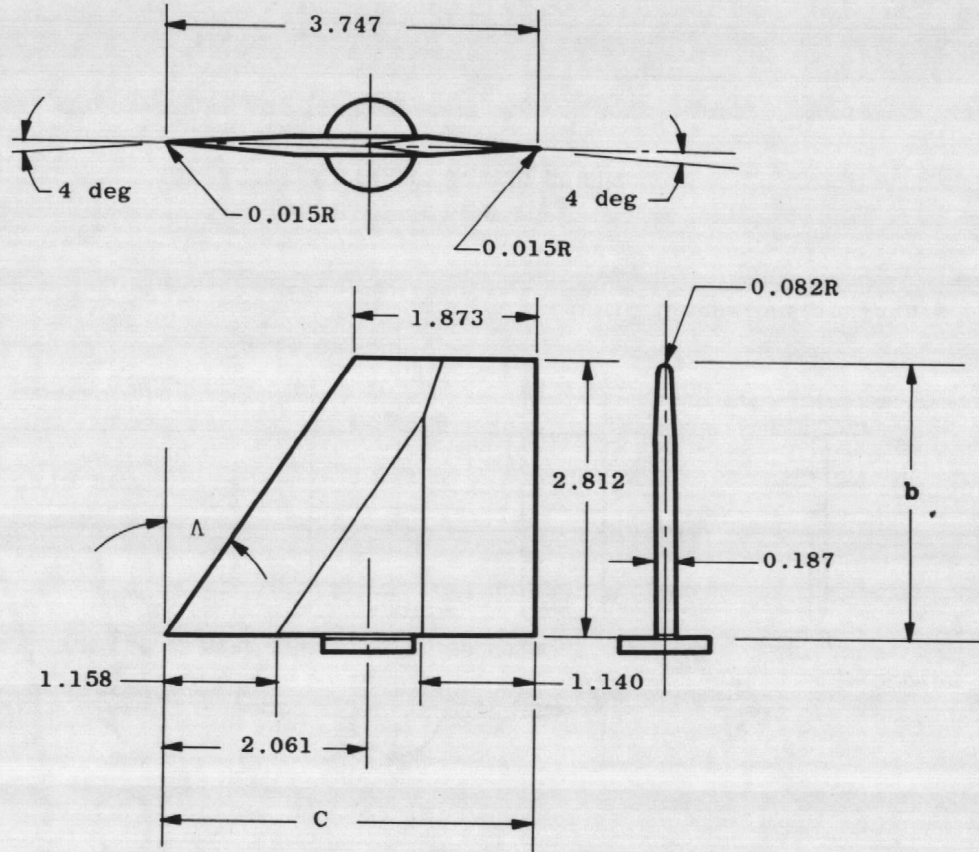
b. Fin T1-3 Figure 4. Continued.
