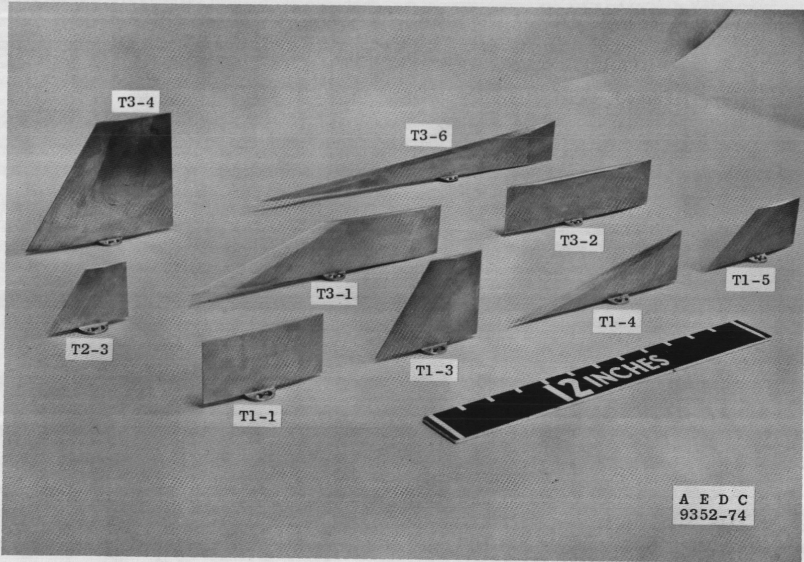
Figure 3. Photograph of fin configurations.
