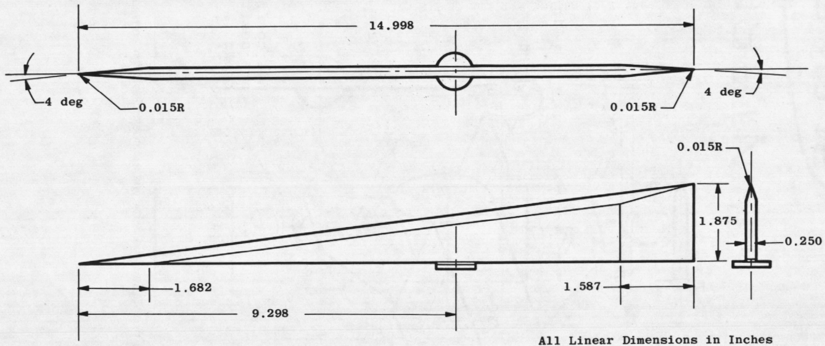
i. Fin T3-6 Figure 4. Concluded.
