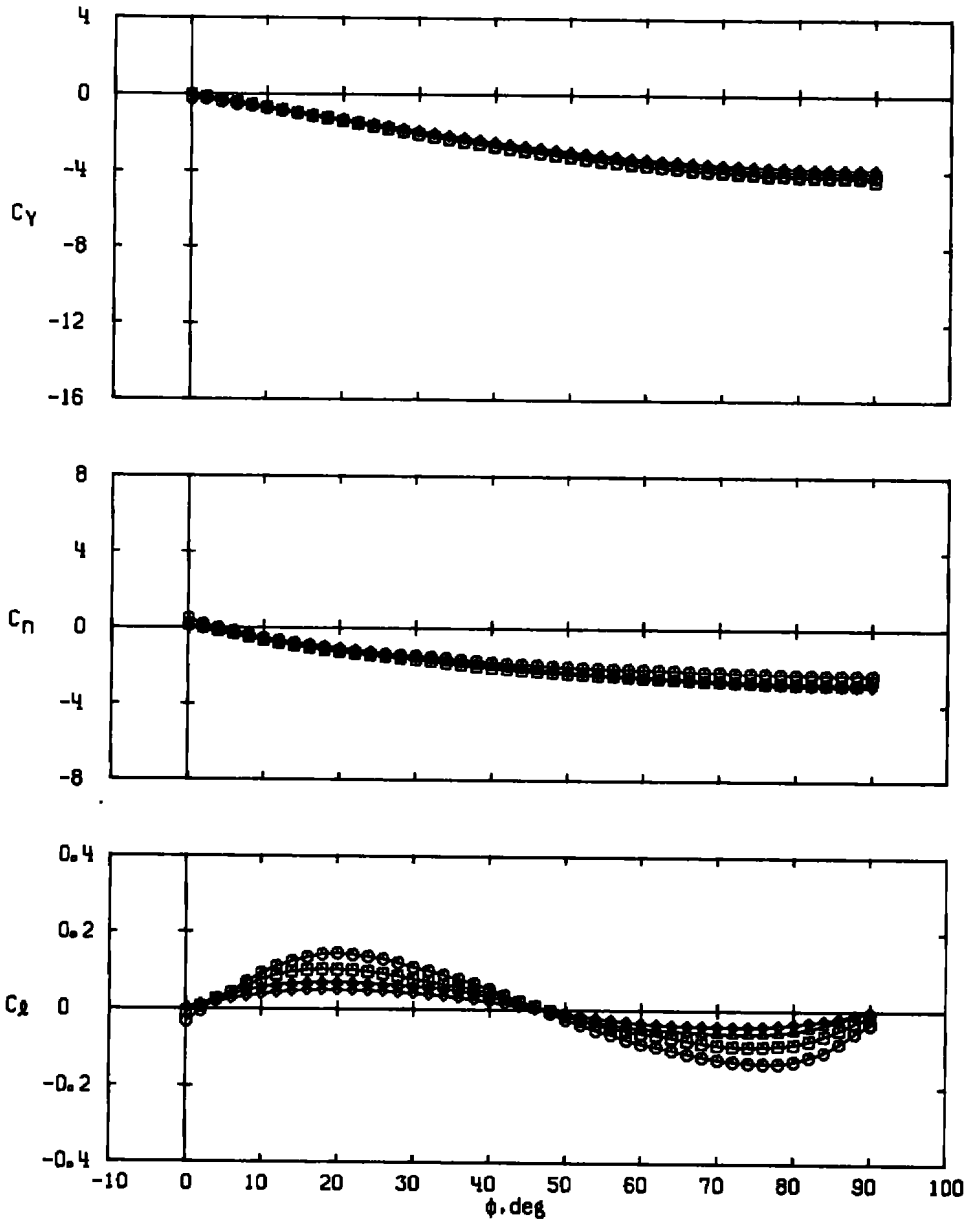
b. \alpha \approx 21 deg Figure 26. Continued.
