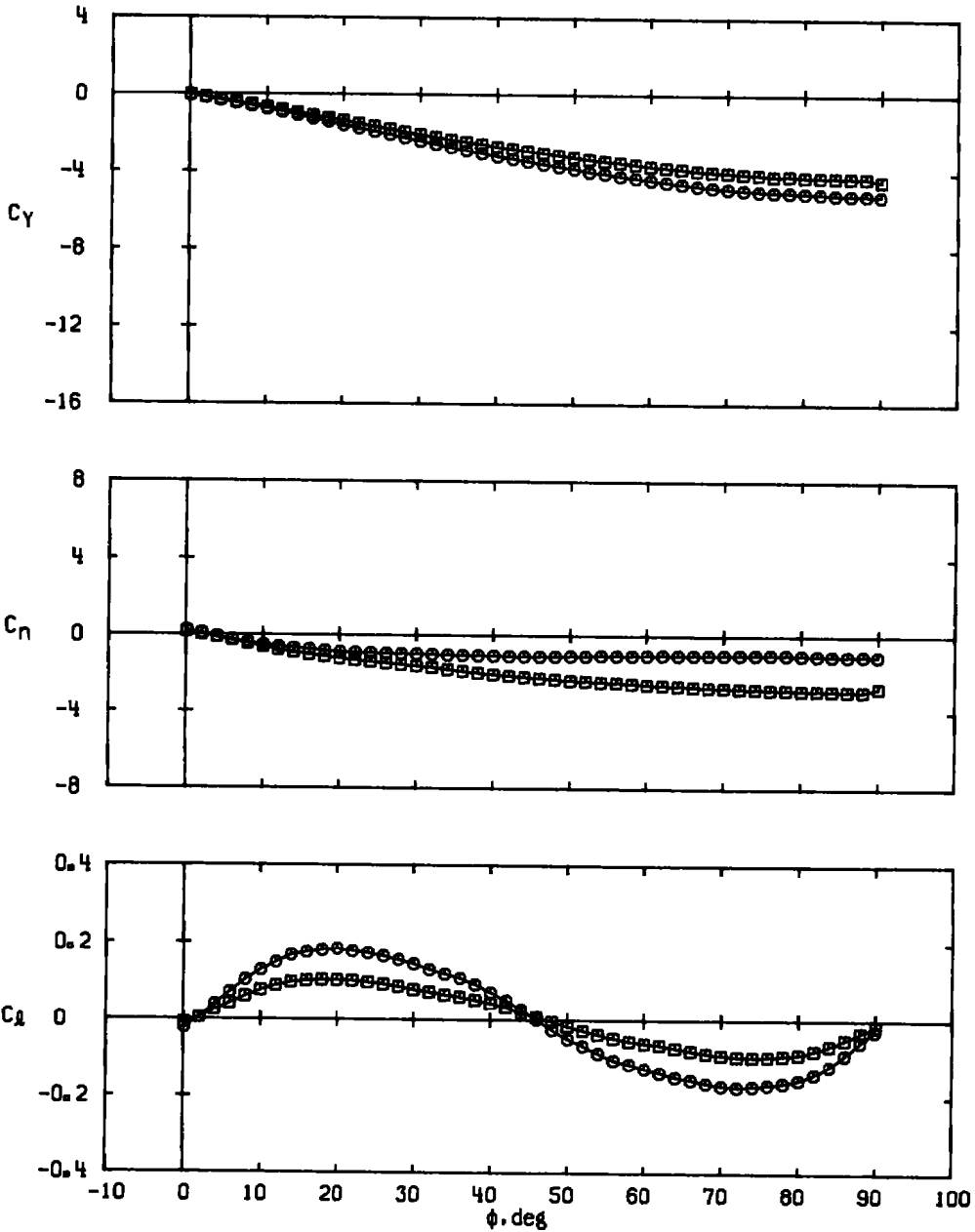
b. \alpha \approx 21 deg Figure 23. Continued.
