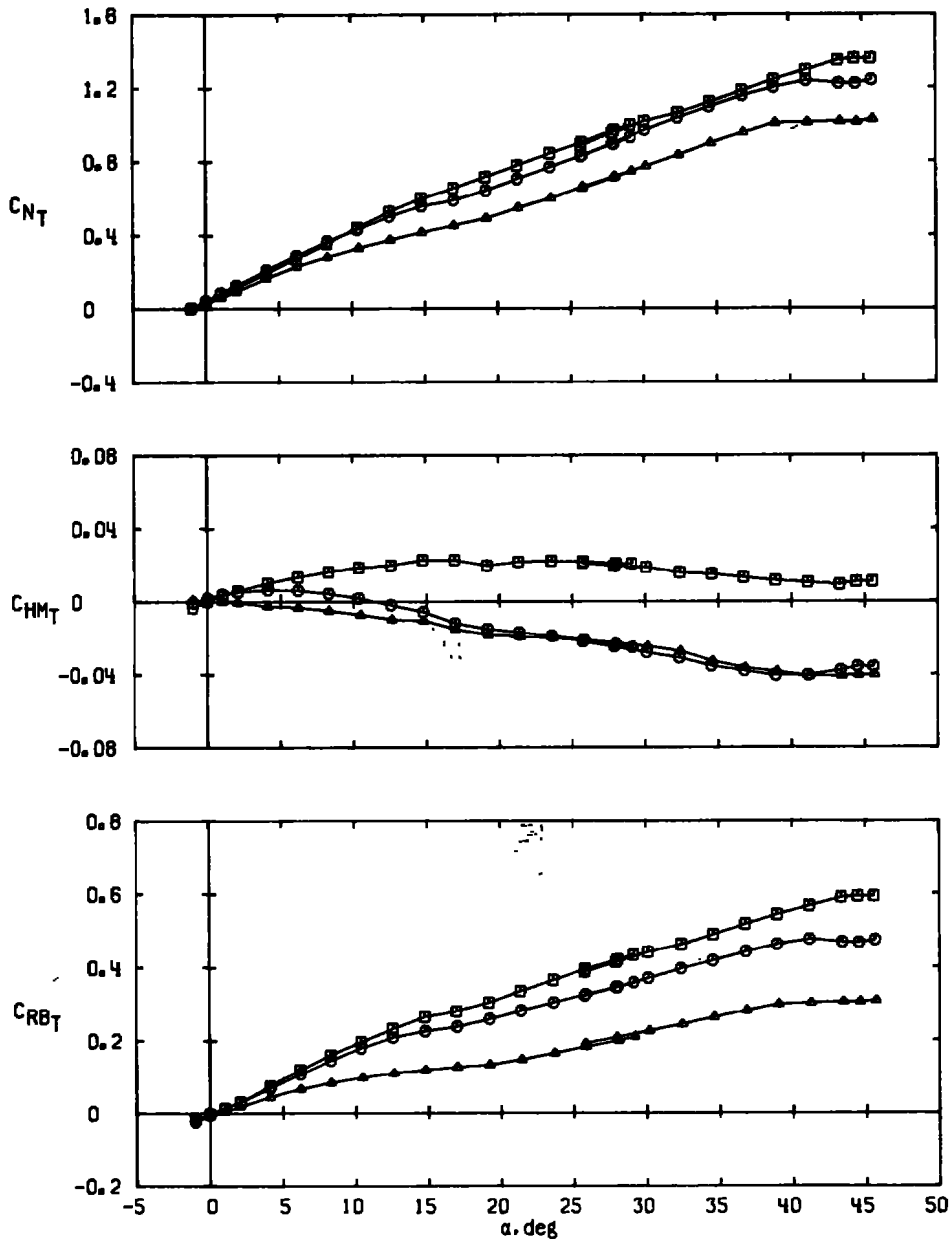
b. M_\infty = 2.00 Figure 9. Continued.
