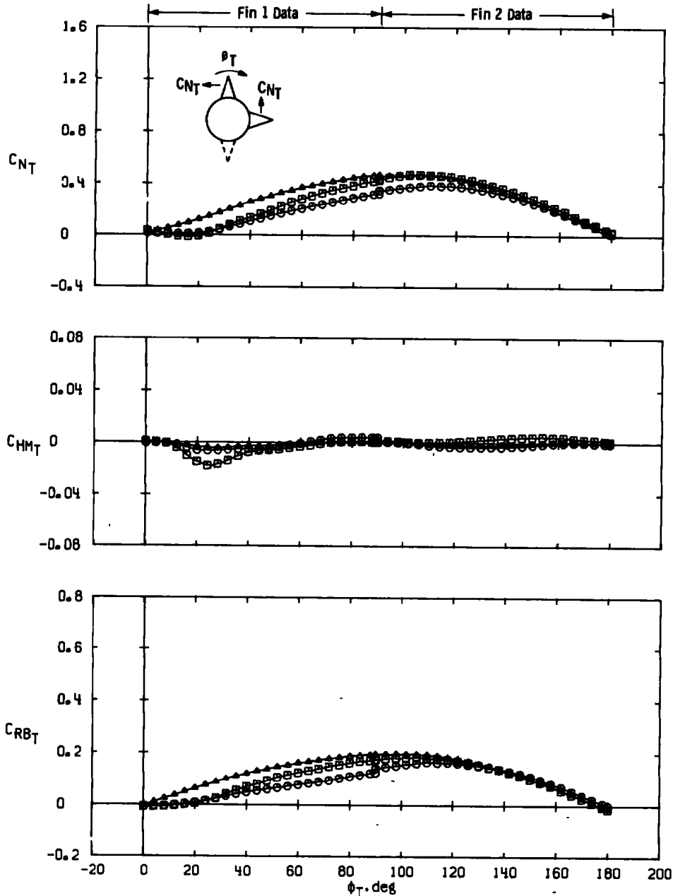
Figure 24. Variations in fin normal-force, hinge-moment, and bending-moment coefficients with fin roll position for different delta fin aspect ratios, M_\infty = 2.00 .
