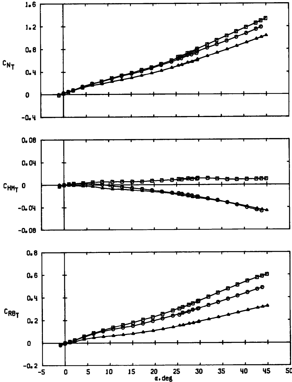
d. M_\infty = 3.01 Figure 9. Concluded.
