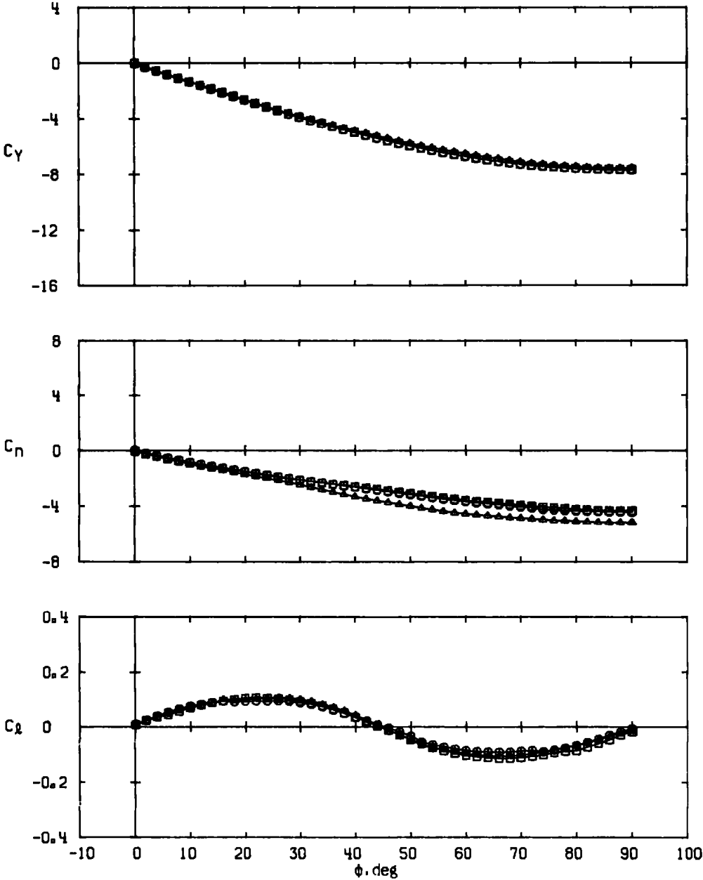
c. \alpha \approx 32 deg Figure 17. Continued.
