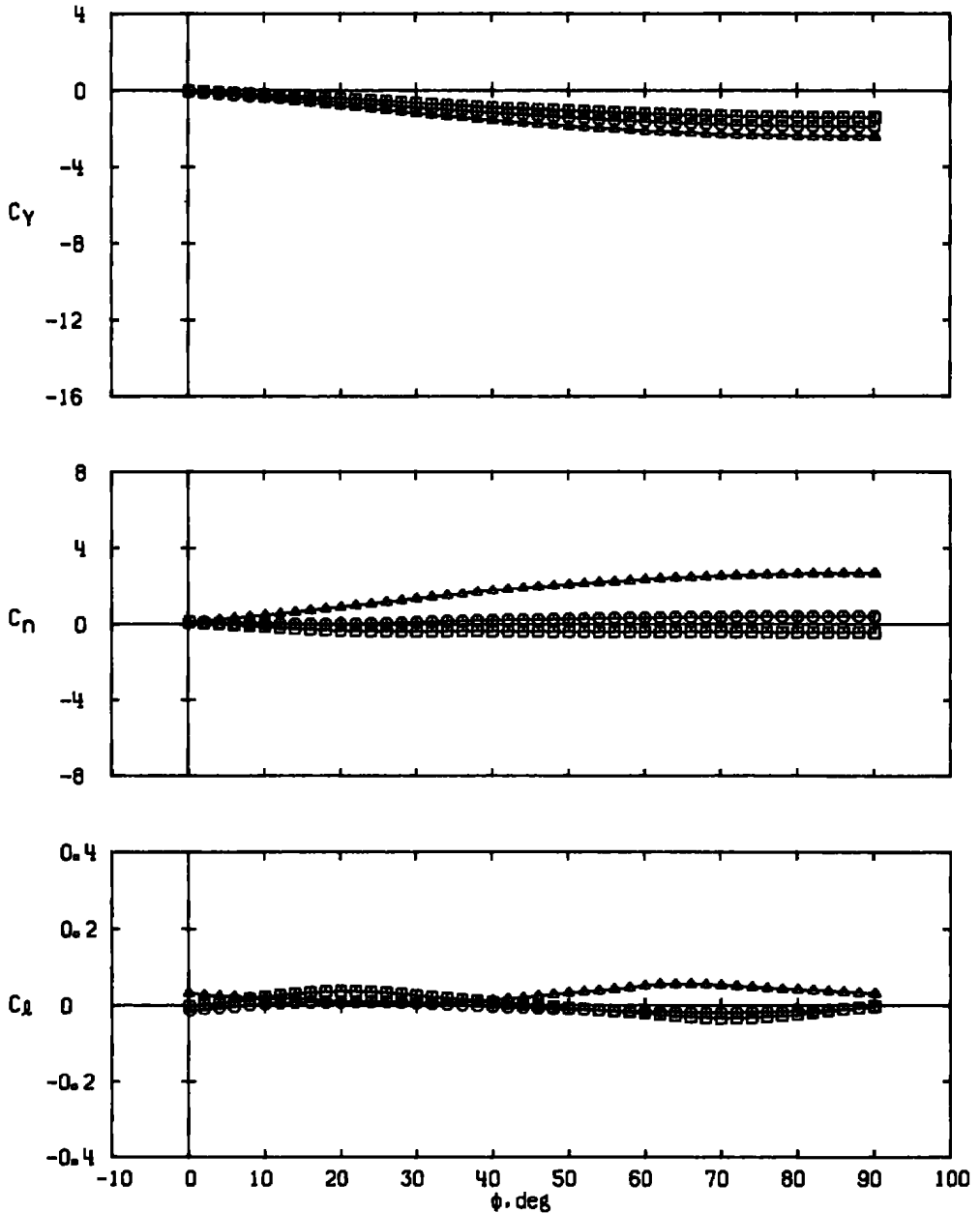
Figure 23. Variations in missile side-force, yawing-moment, and rolling-moment coefficients with roll angle for different delta fin aspect ratios, M_\infty = 2.00 .
