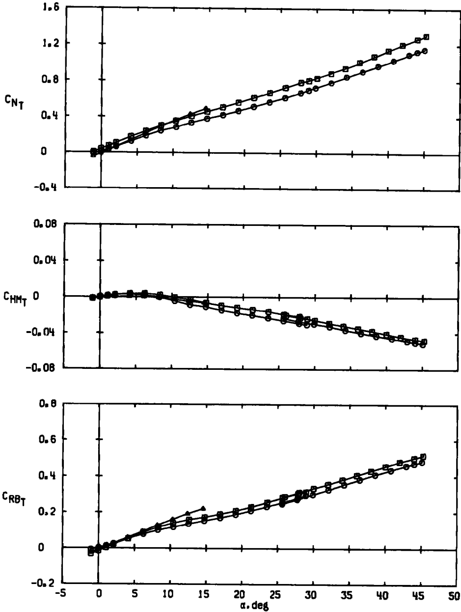
c. M_\infty = 2.50 Figure 13. Continued.
