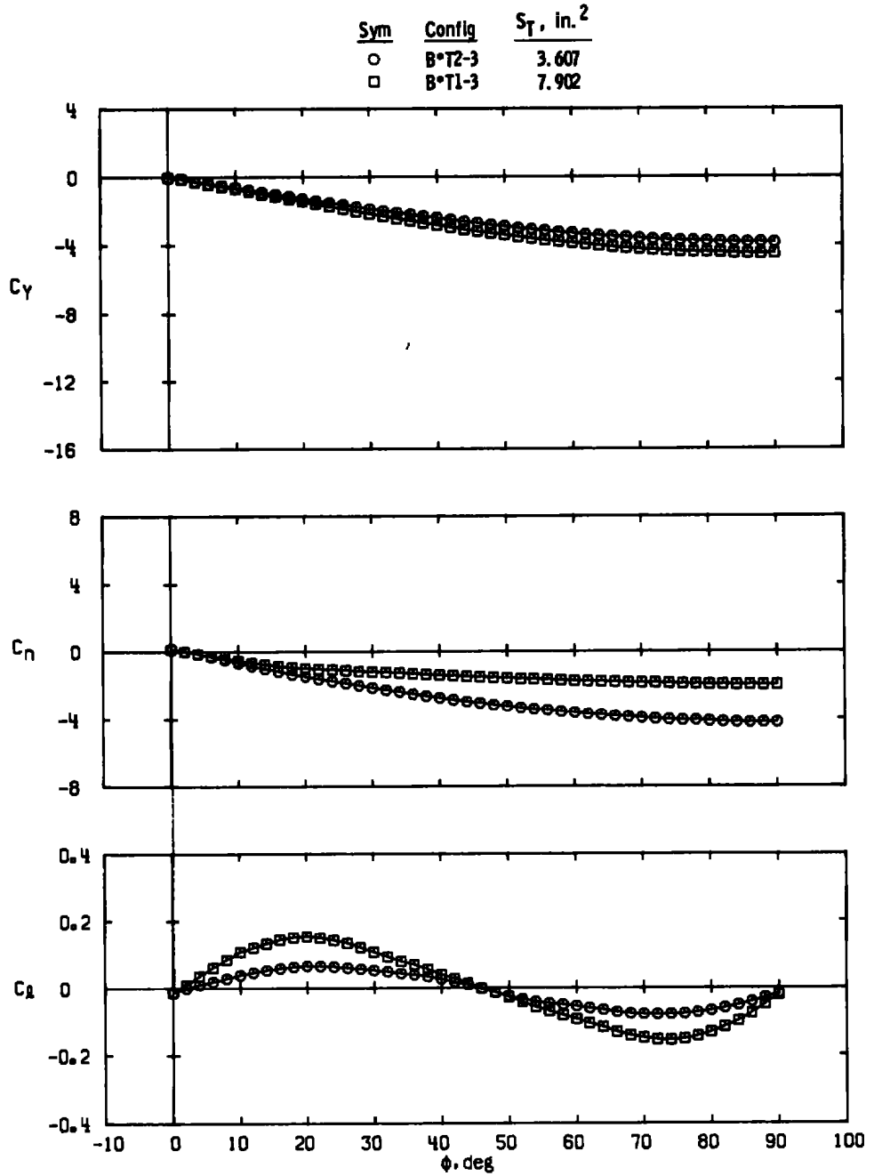
b. a \approx 21 \text{ deg} Figure 20. Continued.
