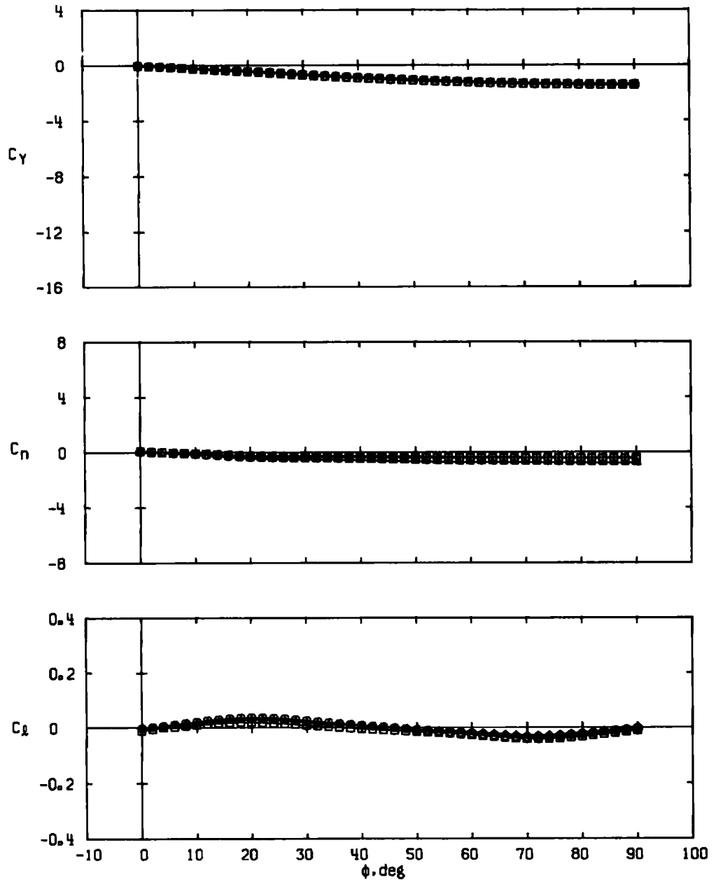
Figure 17. Variations in missile side-force, yawing-moment, and rolling-moment coefficients with roll angle for different fin planform shapes of aspect ratio 1.0, M_\infty = 2.00 .
