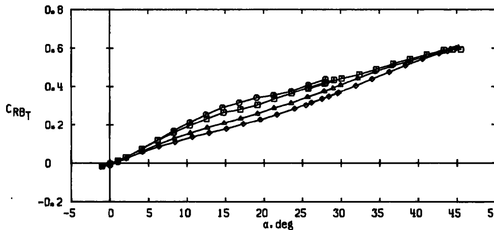
b. Configuration B*T1-1, rectangular fin, S_T = 7.031 \text{ in.}^2 Figure 15. Continued.
