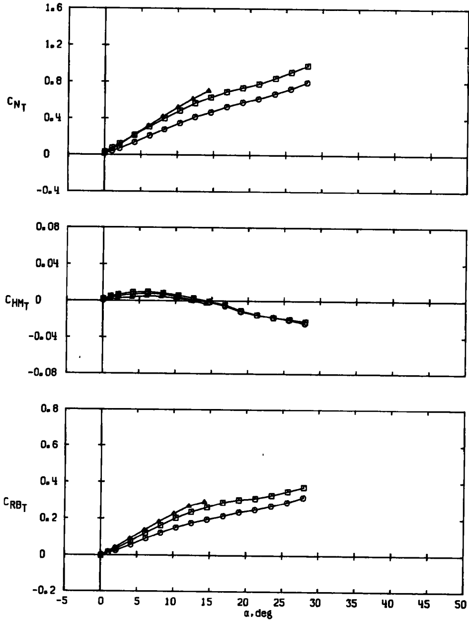
Figure 13. Effect of delta fin aspect ratio on fin aerodynamic characteristics, \phi = 0 .
