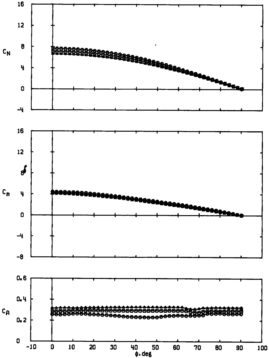
c. \alpha \approx 32 \text{ deg} Figure 25. Continued.
