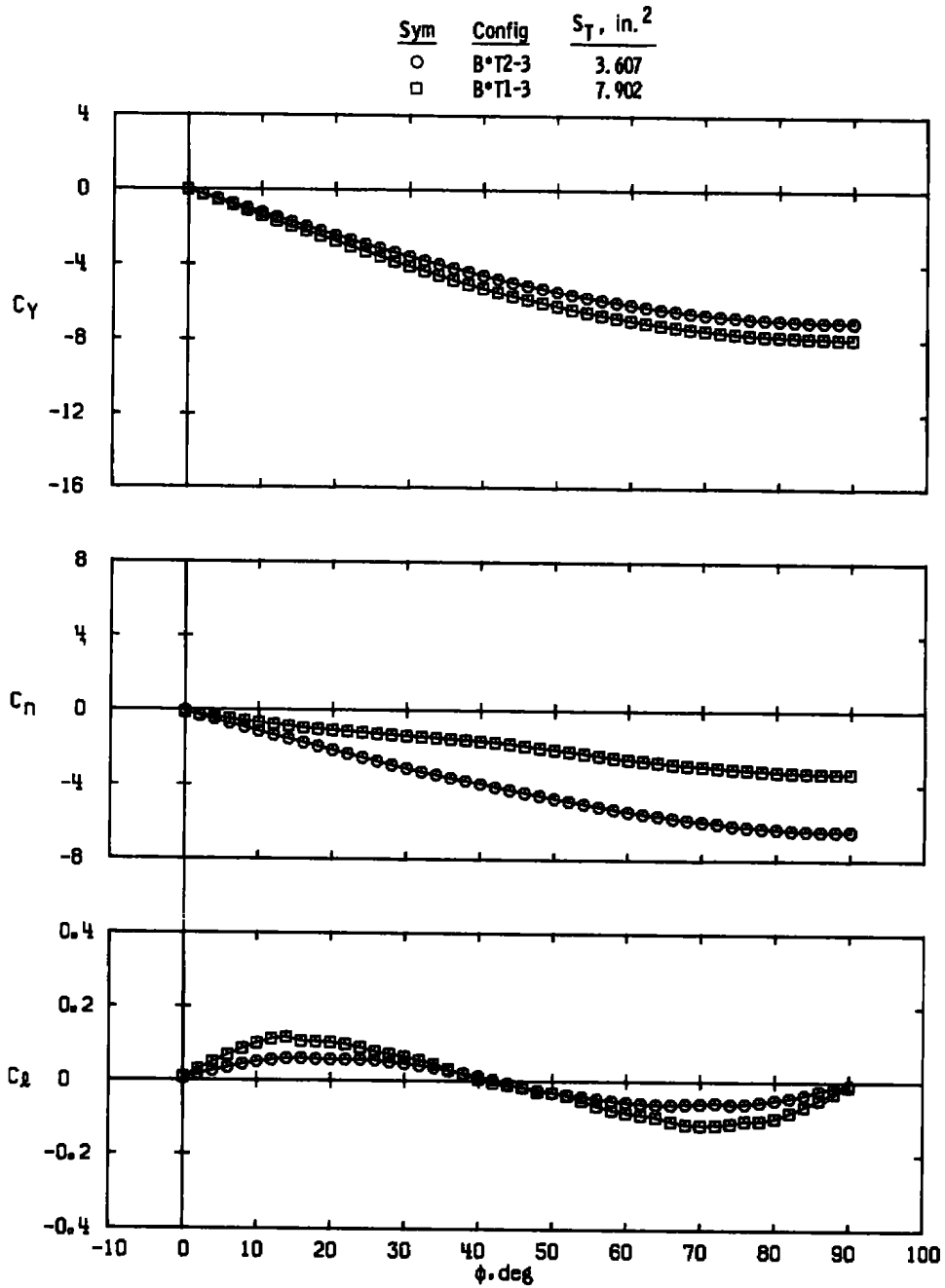
c. \alpha \approx 32 deg Figure 20. Concluded.
