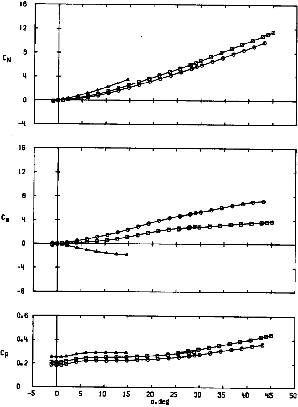
c. M_\infty = 2.50 Figure 10. Continued.
