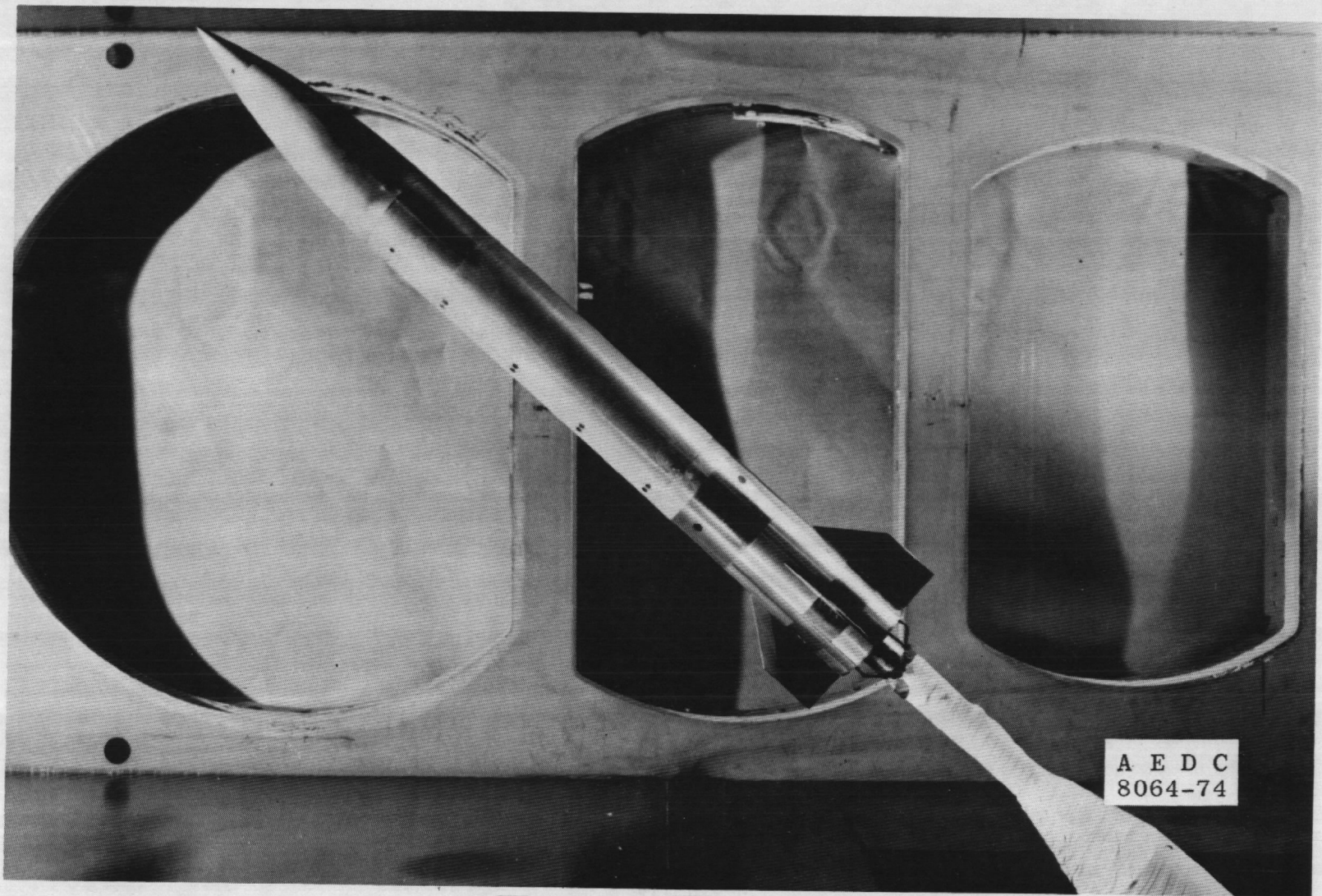
b. Configuration B*T1-5, \alpha \approx 42 deg Figure 1. Concluded.
