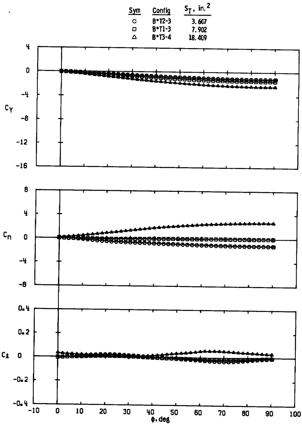
Figure 20. Variations in missile side-force, yawing-moment, and rolling-moment coefficients with roll angle for different delta fin planform areas of aspect ratio 2.0, M_\infty = 2.00 .
