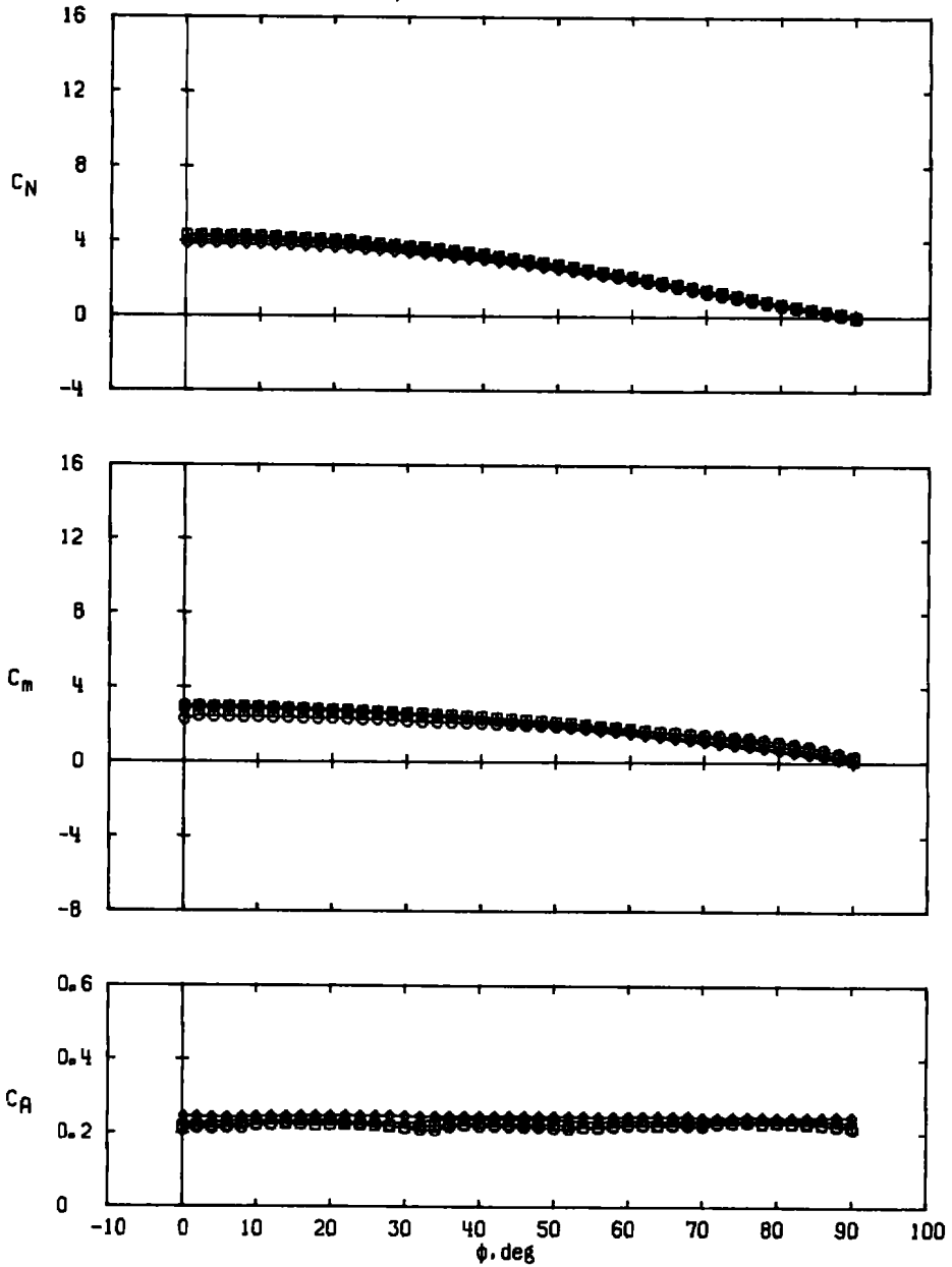
b. a \approx 21 \text{ deg} Figure 25. Continued.
