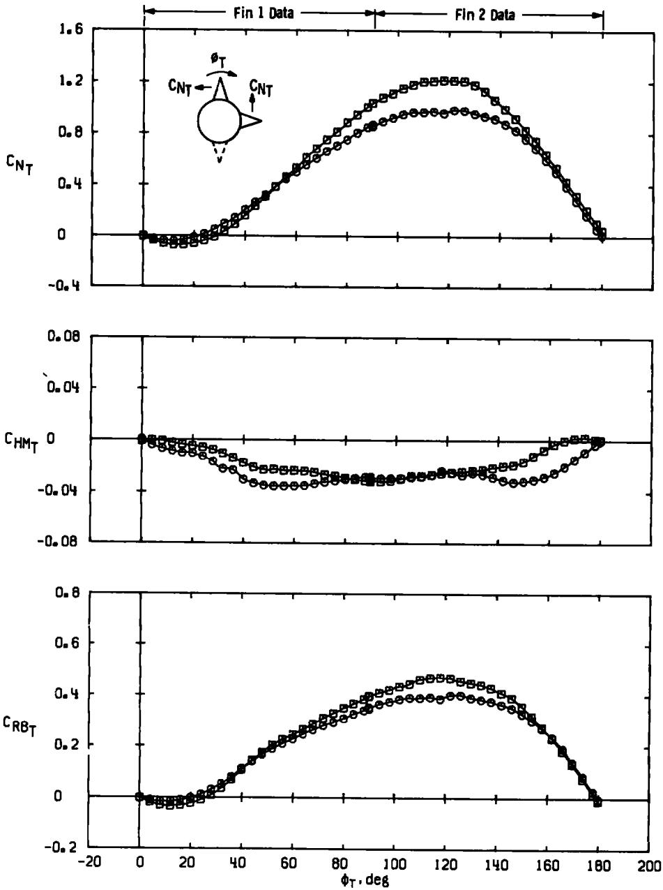
c. a \approx 32 deg Figure 24. Concluded.
