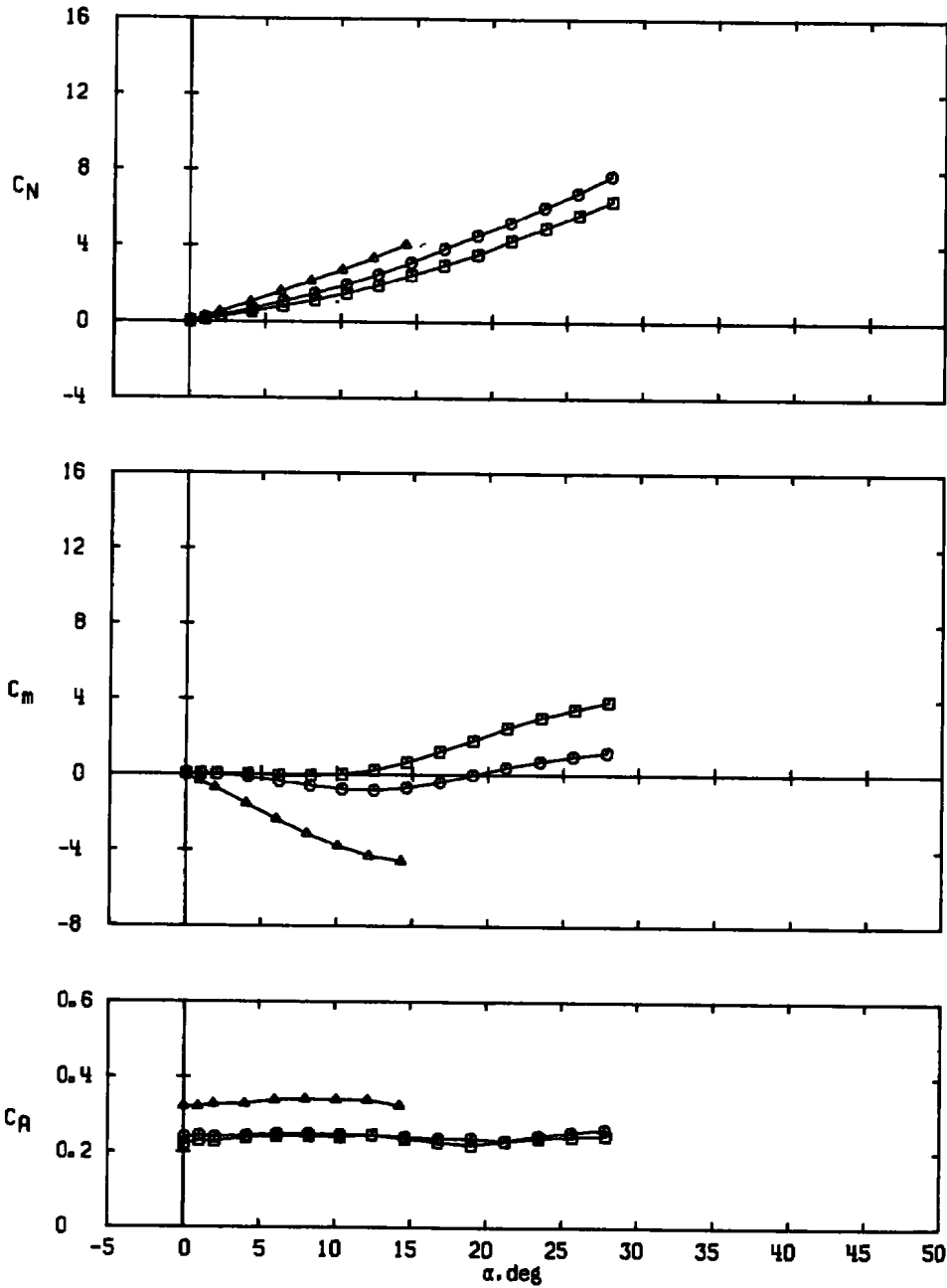
Figure 12. Effect of delta fin aspect ratio on missile longitudinal stability and axial-force characteristics, \phi = 0 .
