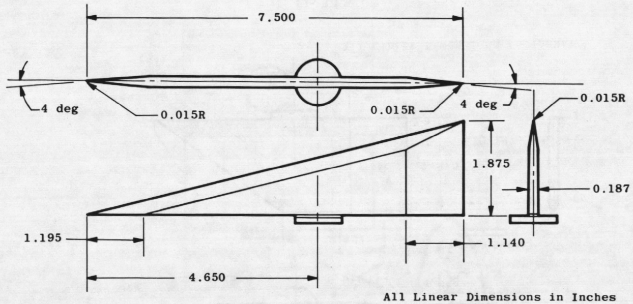
c. Fin T1-4 Figure 4. Continued.
