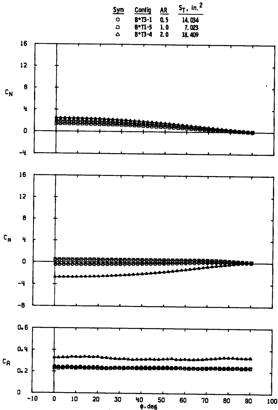
Figure 22. Variations in missile normal-force, pitching-moment, and axial-force coefficients with roll angle for different delta fin aspect ratios, M_\infty = 2.00 .
