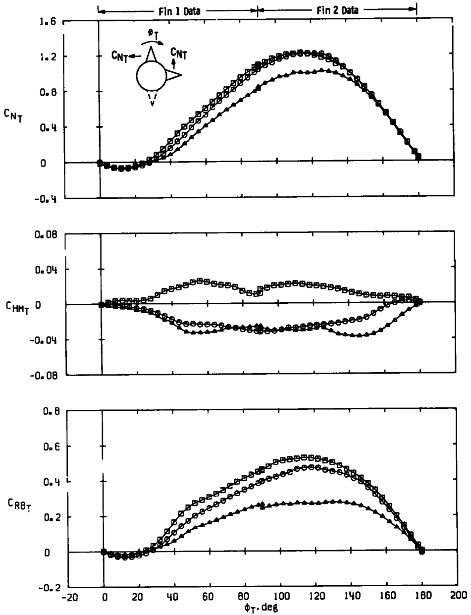
c. \alpha \approx 32 deg Figure 18. Continued.
