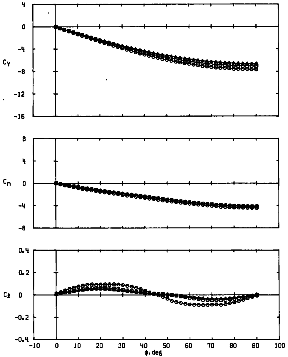
c. \alpha \approx 32 \text{ deg} Figure 26. Continued.
