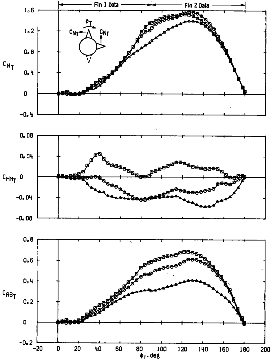
d. \alpha \approx 43 deg Figure 18. Concluded.
