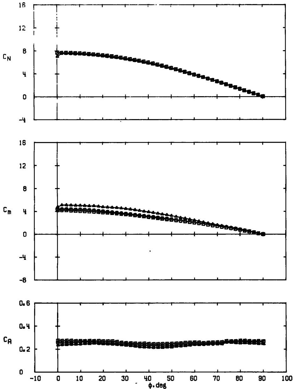
c. \alpha \approx 32 deg Figure 16. Continued.
