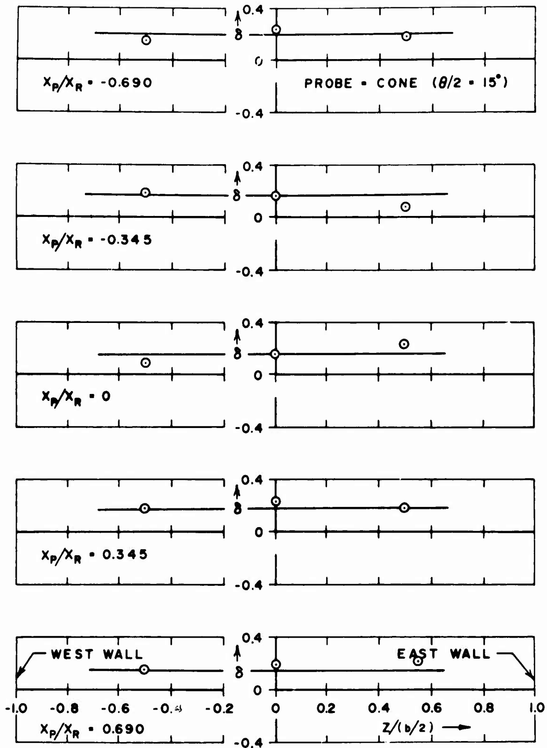
Figure 39. Flow Angularity versus Lateral Distance with Longitudinal Distance as a Parameter for p_0 = 100 psia, T_0 = 470^\circ\text{R} , M = 2.99 and Re/l = 20.6 \times 10^6 per foot
