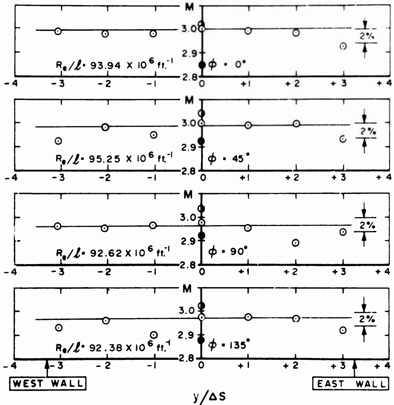
Figure 25d. Impact Mach Number versus y/\Delta s for x_p/x_r = +0.345 at p_0 = 517 psia and T_0 = 491^\circ\text{R}
