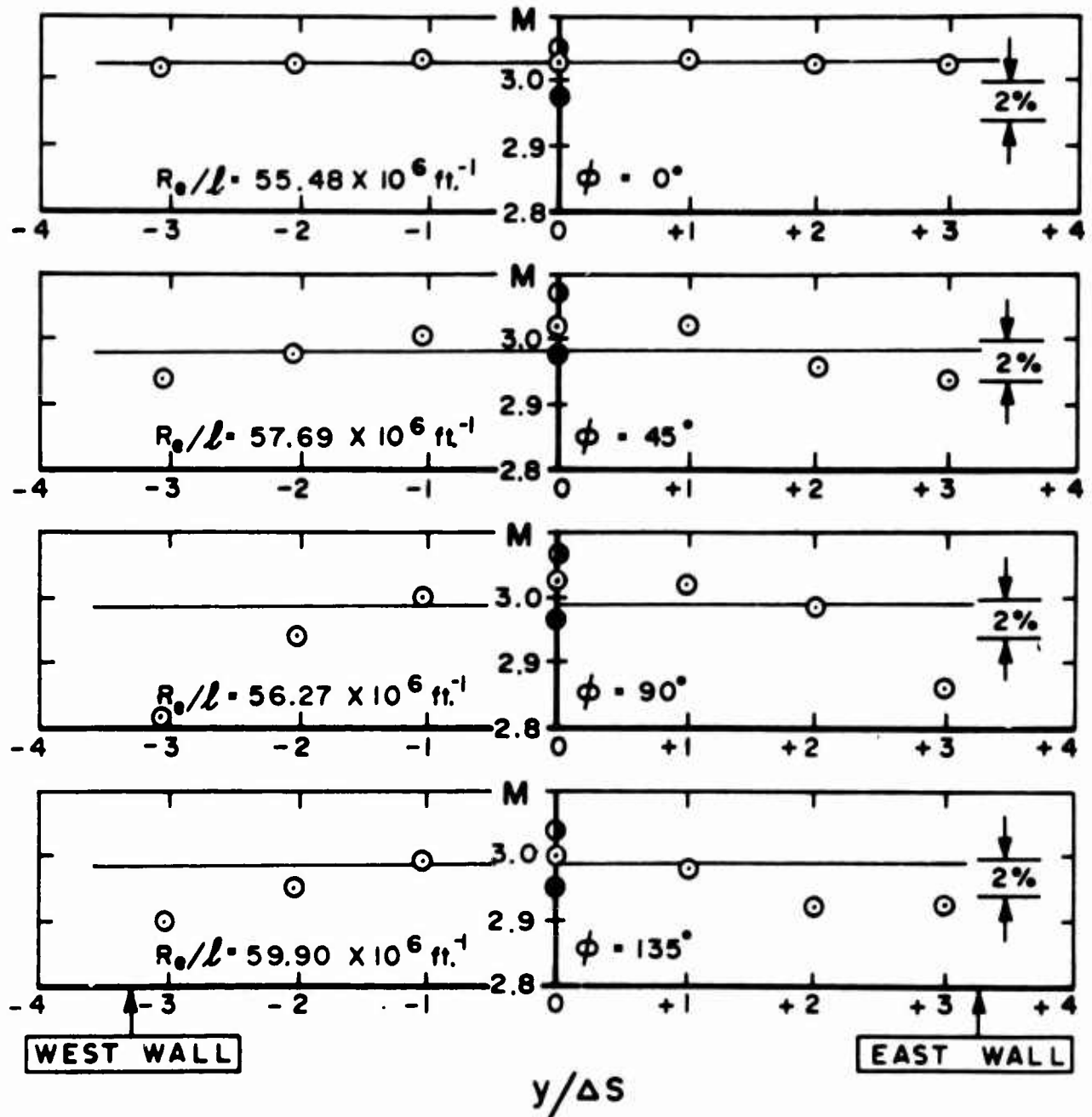
Figure 24b. Impact Mach Number versus y/\Delta s for x_p/x_r = -0.345 at p_0 = 316 \text{ psia} and T_0 = 482^\circ\text{R}
