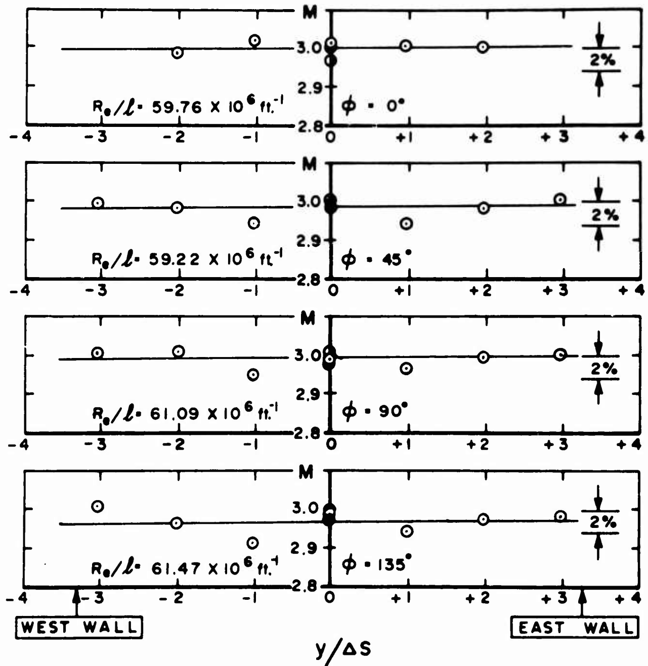
Figure 24e. Impact Mach Number versus y/\Delta s for x_p/x_r = +0.690 at p_0 = 318 \text{ psia} and T_0 = 476^\circ\text{R}
