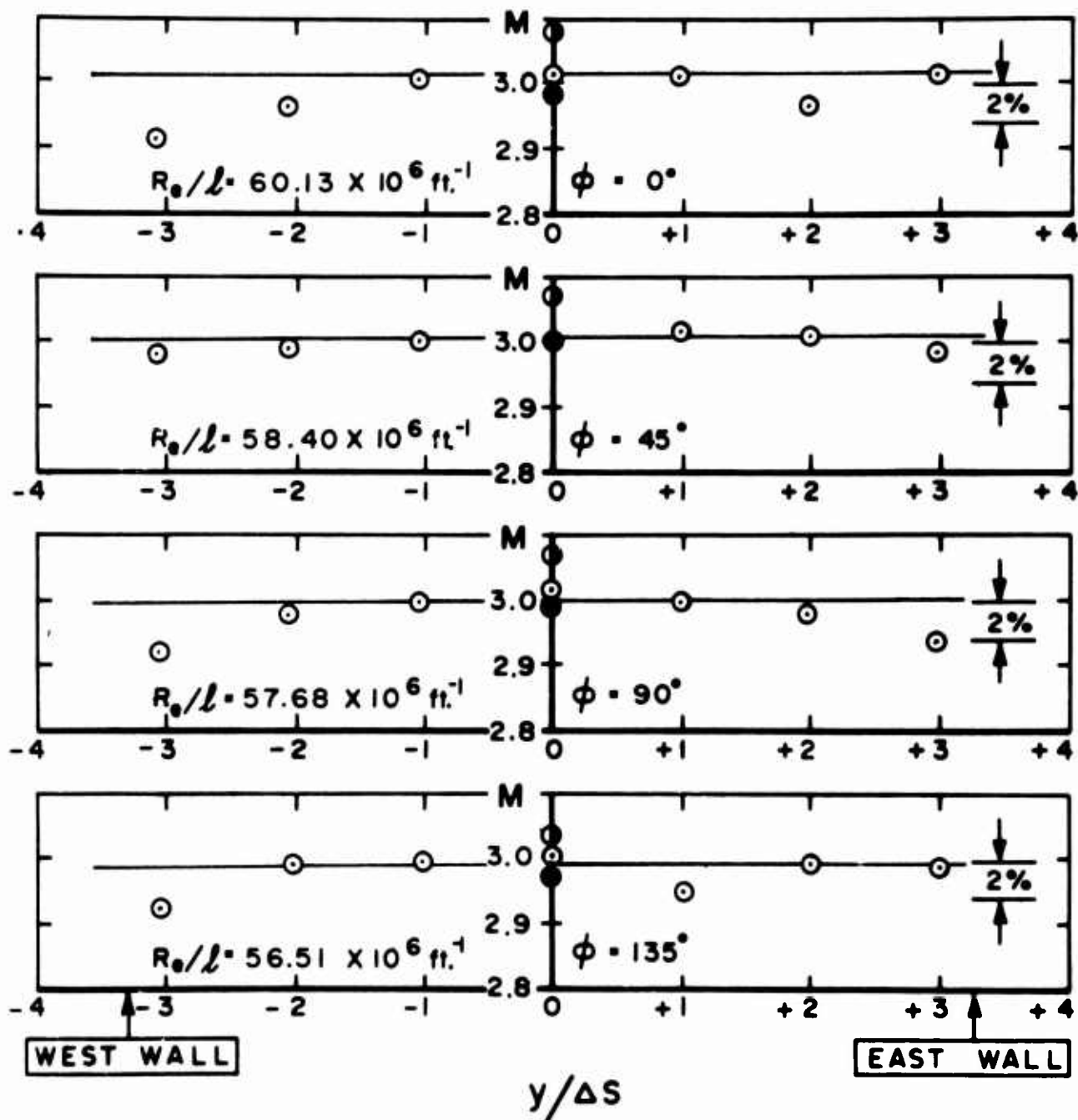
Figure 24c. Impact Mach Number versus y/\Delta s for xp/xr = 0 at p_0 = 323 \text{ psia} and T_0 = 491^\circ\text{R}
