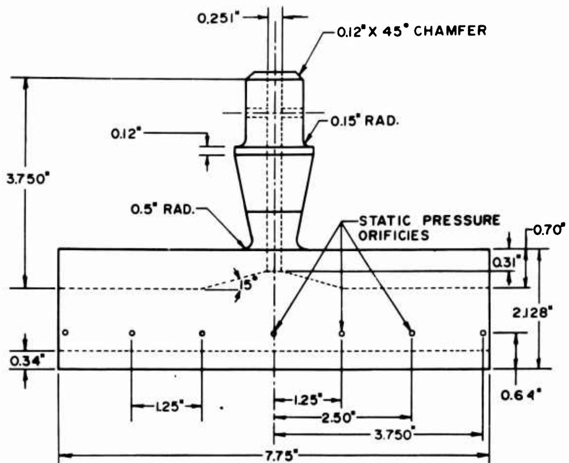
A. WEDGE PLAN VIEW
