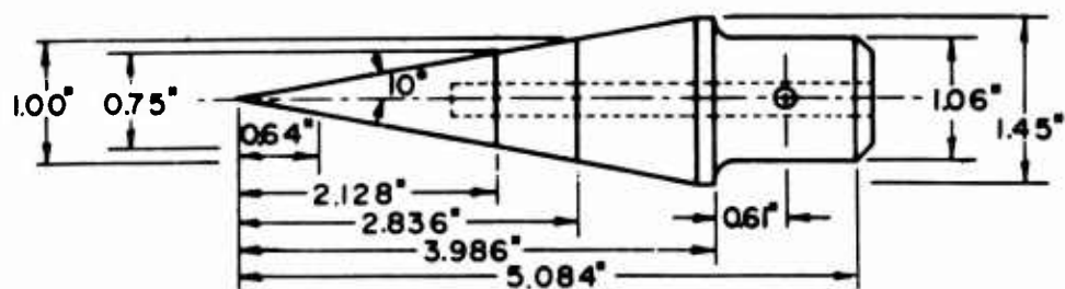
B. WEDGE SIDE VIEW
