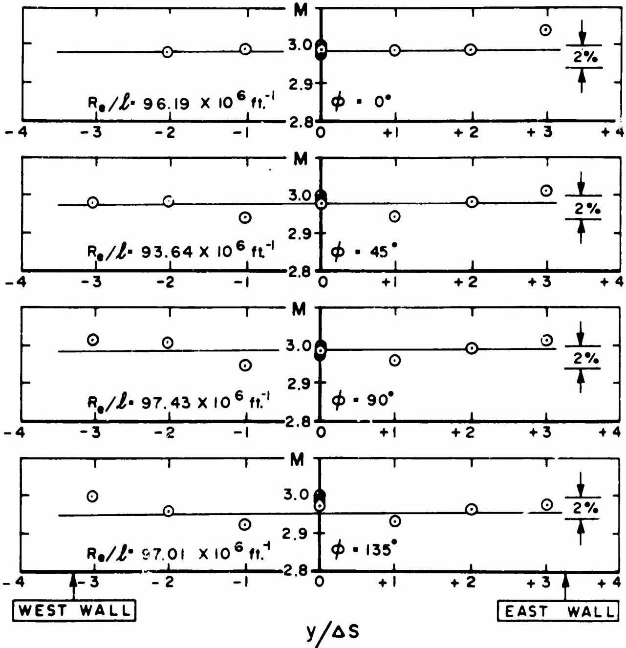
Figure 25e. Impact Mach Number versus y/\Delta s for x_p/x_r = +0.690 at p_0 = 523 \text{ psia} and T_0 = 486^\circ\text{R}
