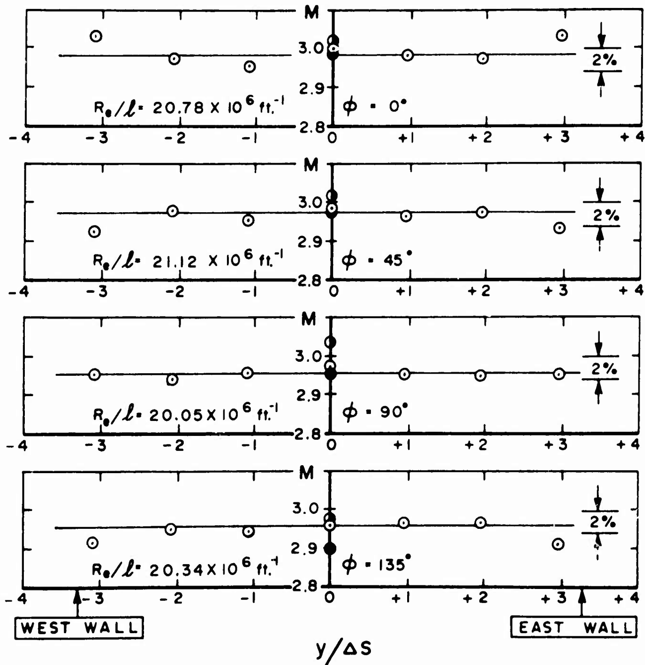
Figure 23d. Impact Mach Number versus y/\Delta s for x_p/x_r = +0.345 at p_0 = 108 \text{ psia} and T_0 = 477^\circ\text{R}
