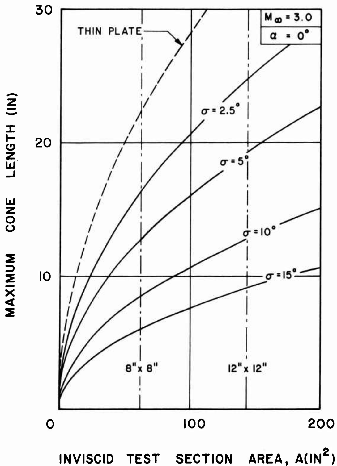
Figure A-9. Variation of Maximum Cone Length with Inviscid Test Section Size for Shock Reflection Limited Cases
