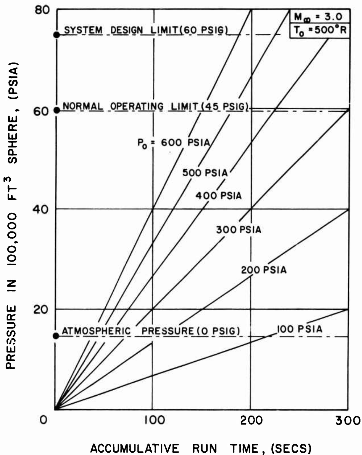
Figure 5. Rise of Sphere Pressure with Run Time for a Range of Stagnation Pressures
