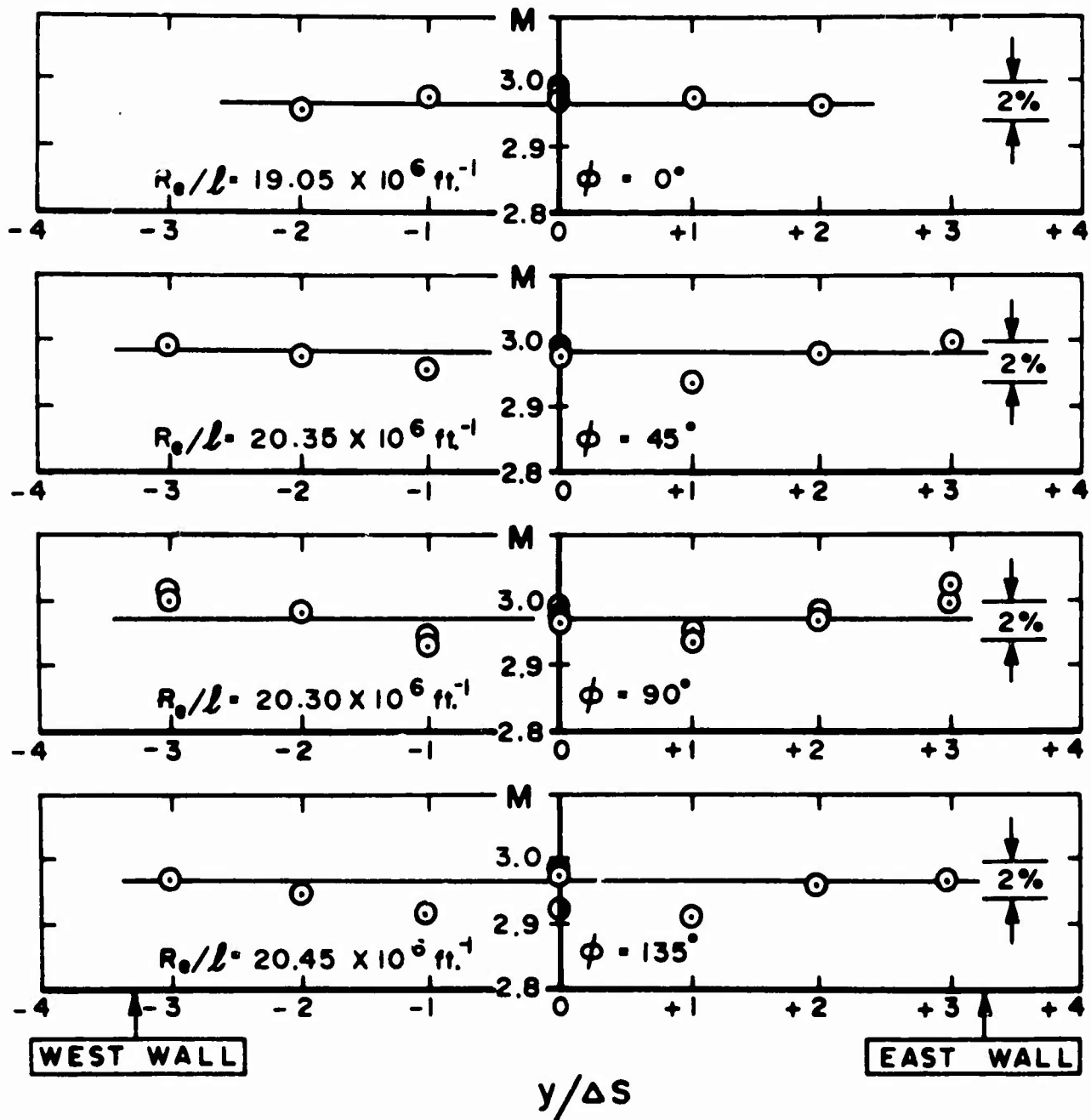
Figure 23e. Impact Mach Number versus y/\Delta s for x_p/x_r = +0.690 at p_0 = 103 \text{ psia} and T_0 = 472^\circ\text{R}
