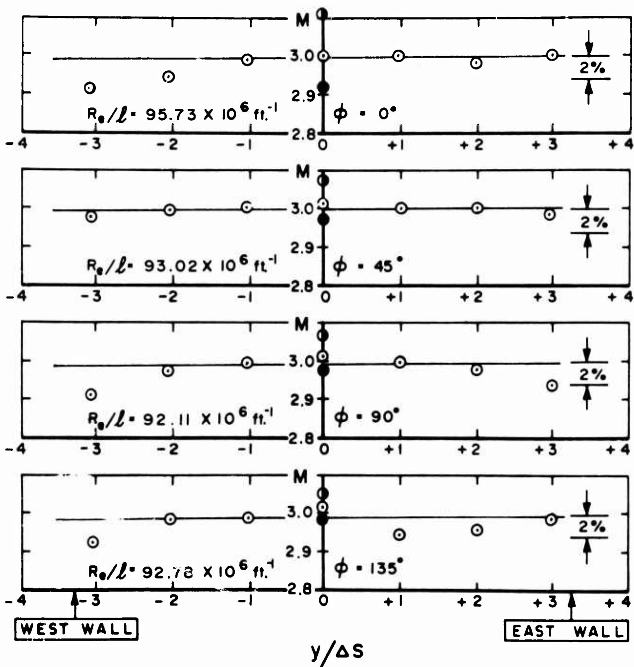
Figure 25c. Impact Mach Number versus y/\Delta s for x_p/x_r = 0 at p_0 = 532 psia and T_0 = 499^\circ\text{R}
