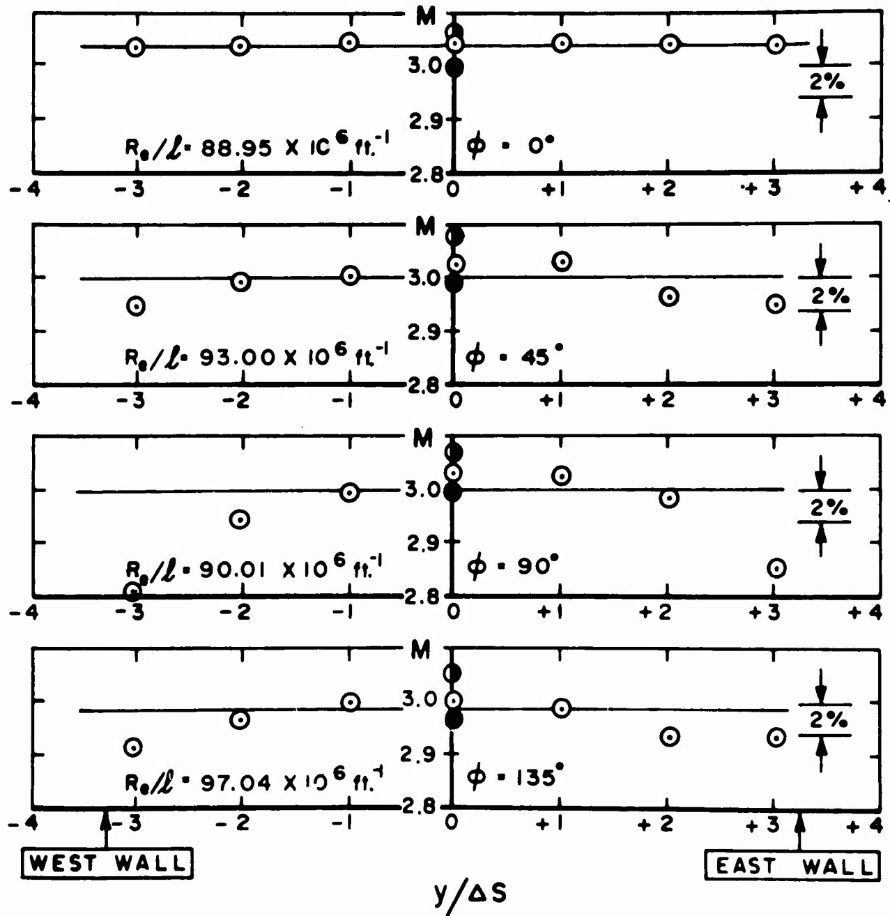
Figure 25b. Impact Mach Number versus y/\Delta s for x_p/x_r = 0.345 at p_0 = 520 \text{ psia} and T_0 = 491^\circ\text{R}
