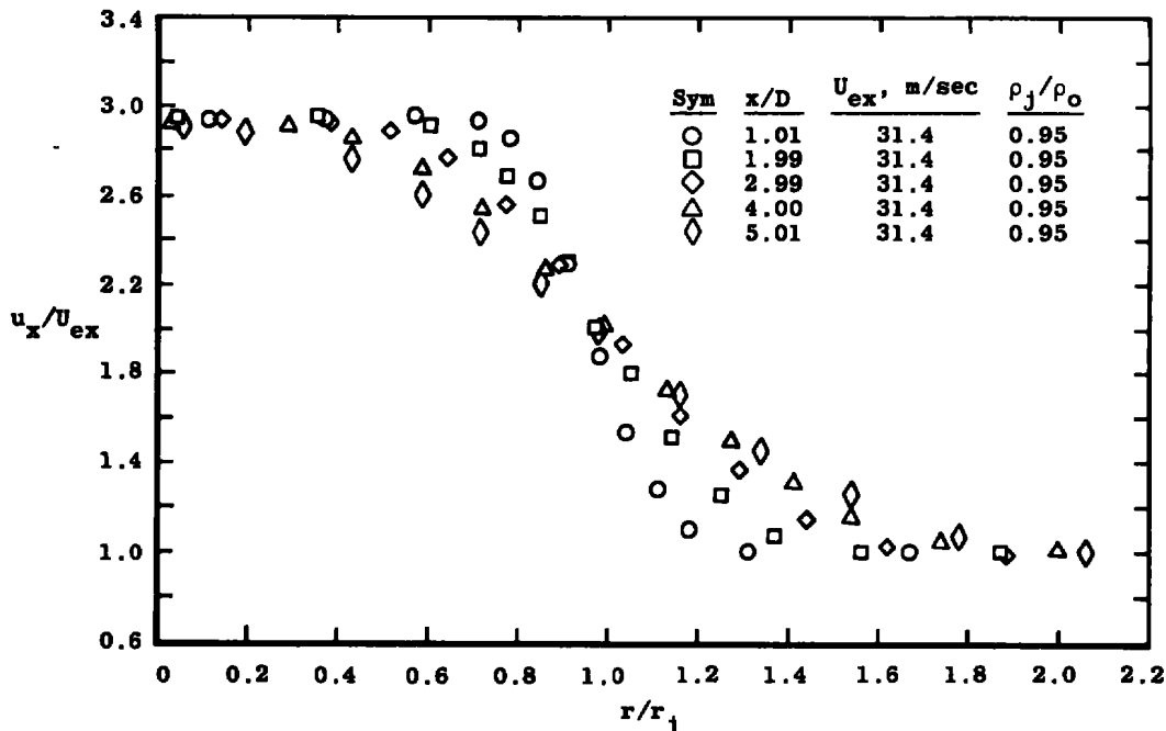
Figure 8. Mean velocity profiles, 3:1 velocity ratio, untripped.
