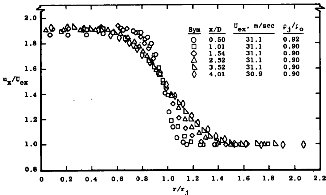
Figure 9. Mean velocity profiles, 2:1 velocity ratio, untripped.
