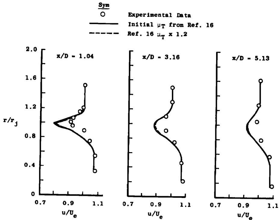
Figure 49. Effect of initial condition on three-equation model prediction, 1:1 velocity ratio, tripped.
