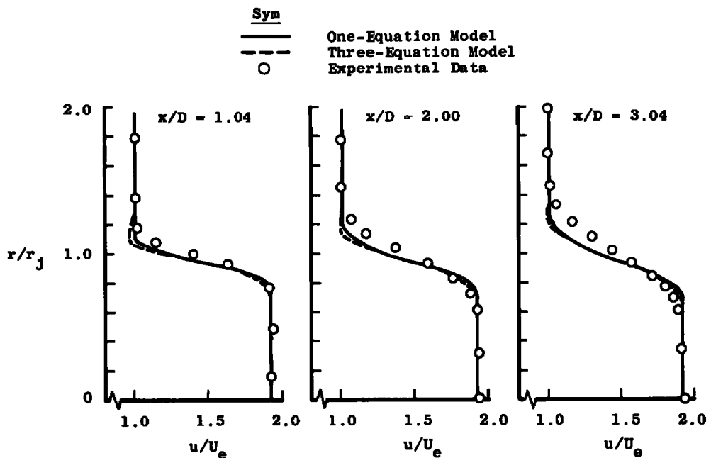
Figure 36. Comparison of predicted and experimental velocity profiles, 2:1 velocity ratio, untripped.
