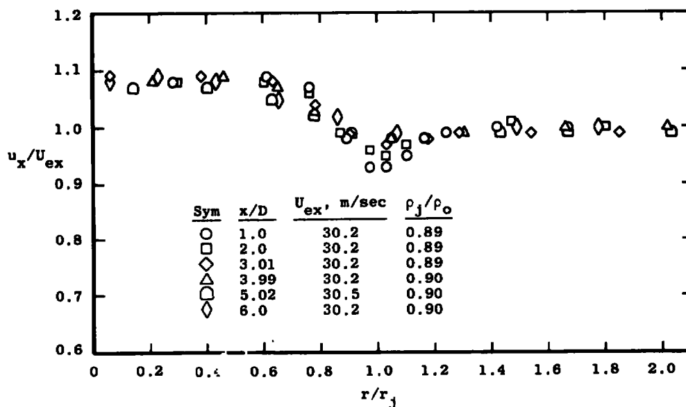
Figure 10. Mean velocity profiles, 1:1 velocity ratio, untripped.
