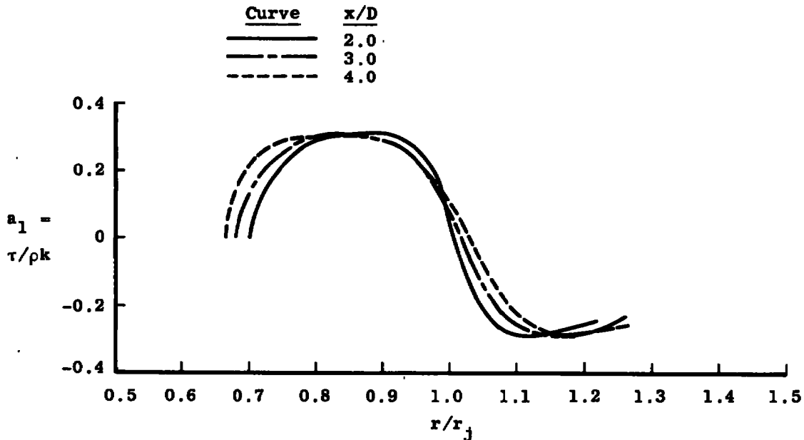
Figure 42. Implied distribution of a_1 , three-equation model, 1:1 velocity ratio, untripped.
