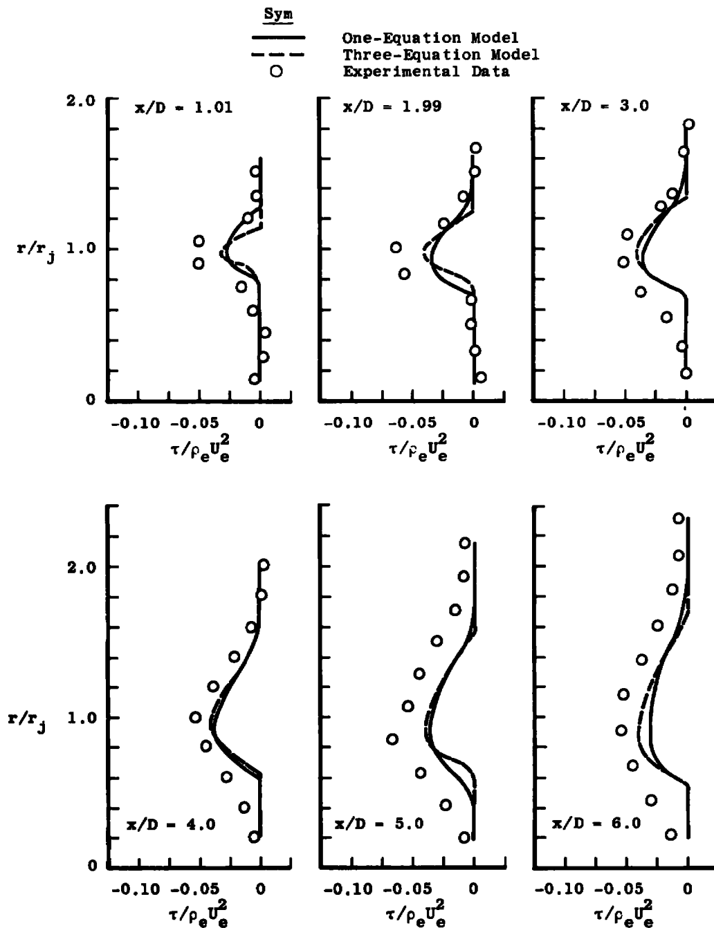
Figure 33. Comparison of predicted and experimental shear stress profiles, 3:1 velocity ratio, untripped.
