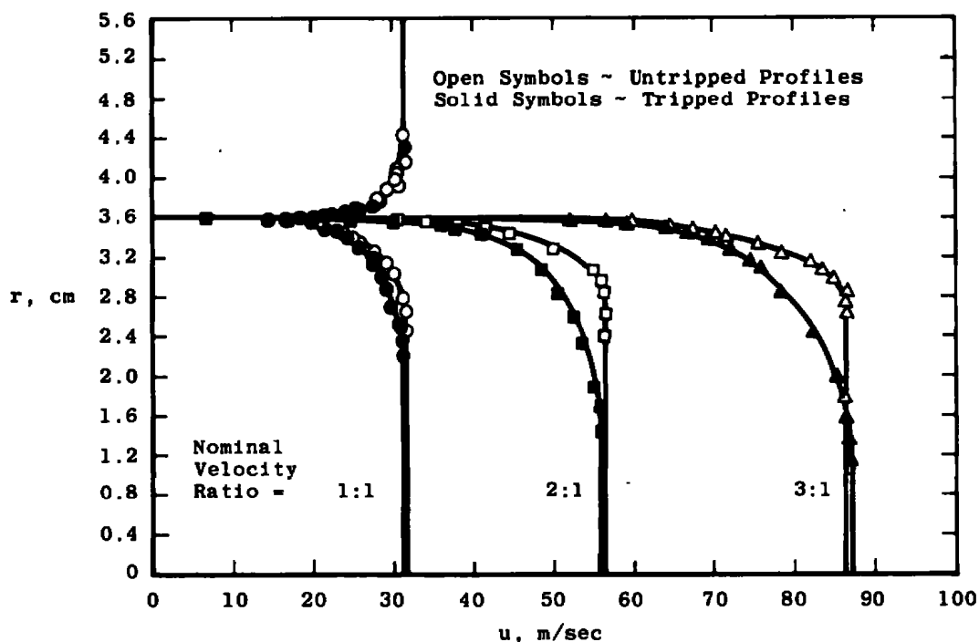
Figure 4. Initial boundary-layer profiles at nozzle exit.
