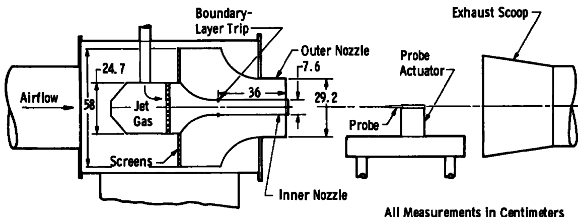
Figure 2. Schematic diagram of the free-jet-mixing test cell.
