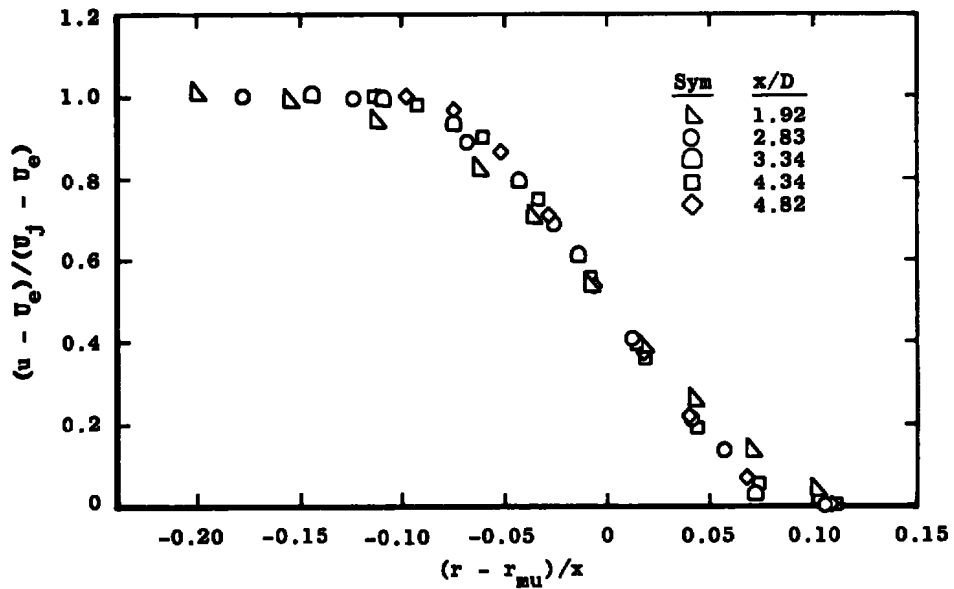
Figure 15. Velocity profiles plotted in two-dimensional shear layer similarity coordinates, 3:1 velocity ratio, tripped.
