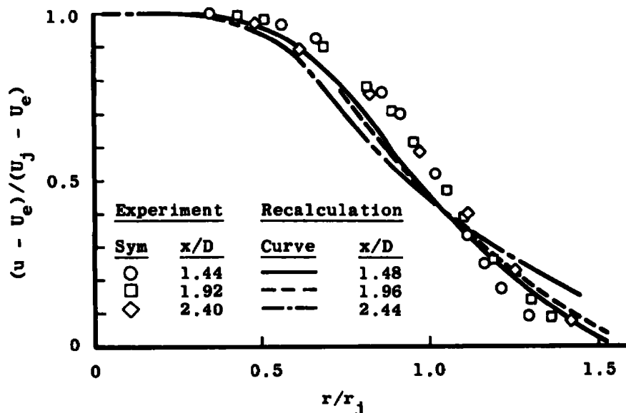
Figure 26. Results of data recalculation, 3:1 velocity ratio, tripped boundary-layer case.
