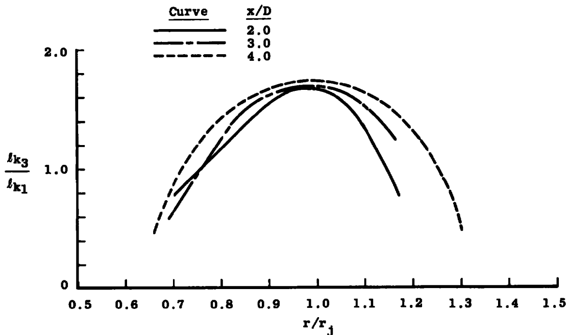
Figure 44. Implied distribution of turbulence length scale, 2:1 velocity ratio, untripped.
