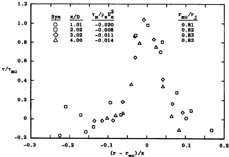
Figure 25. Turbulent shear stress in two-dimensional shear layer similarity coordinates, 2:1 velocity ratio, untripped.
