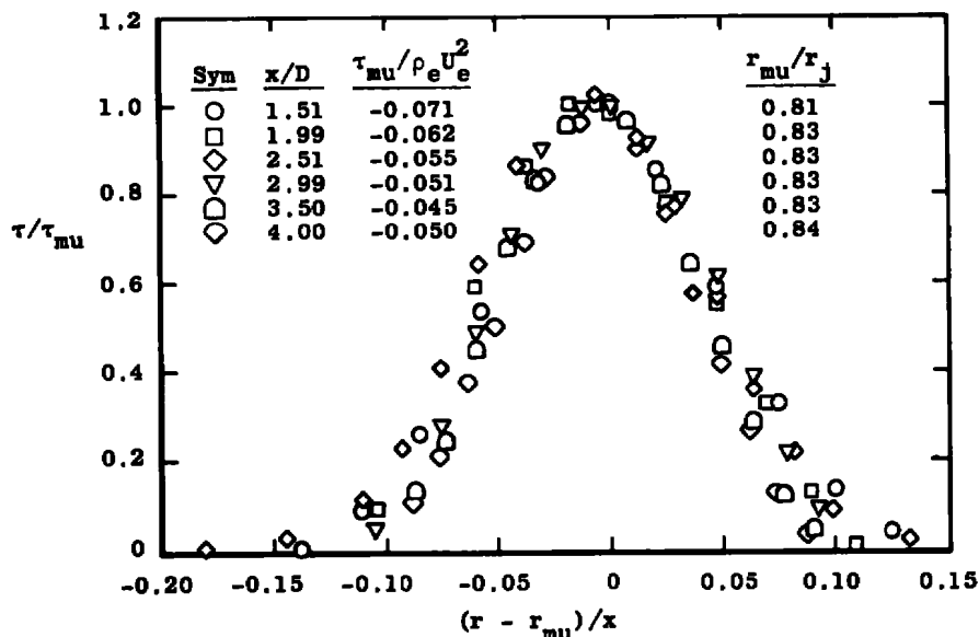
Figure 24. Turbulent shear stress in two-dimensional shear layer similarity coordinates, 3:1 velocity ratio, untripped.
