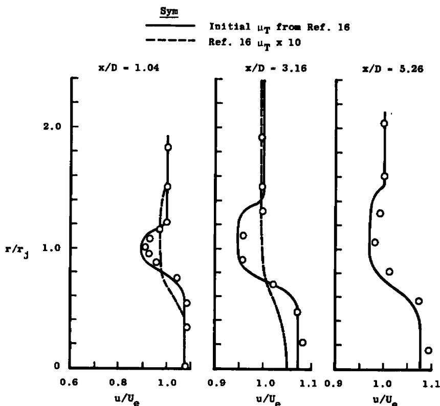
Figure 51. Effect of alteration of initial eddy viscosity profile, one-equation model, 1:1 velocity ratio, tripped.
