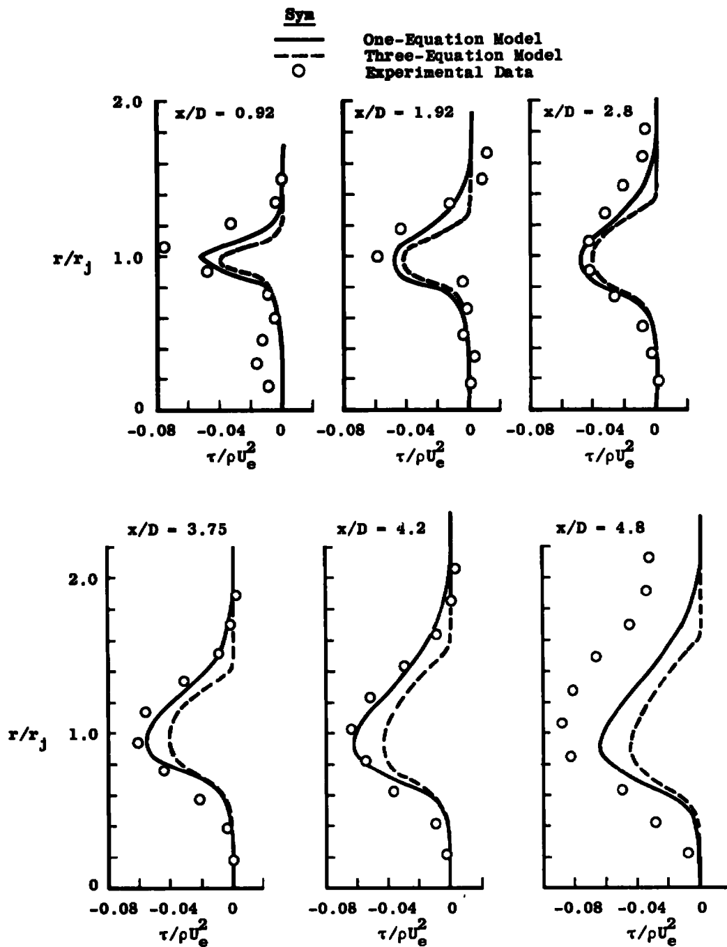
Figure 31. Comparison of predicted and measured shear stress profiles, 3:1 velocity ratio, tripped.
