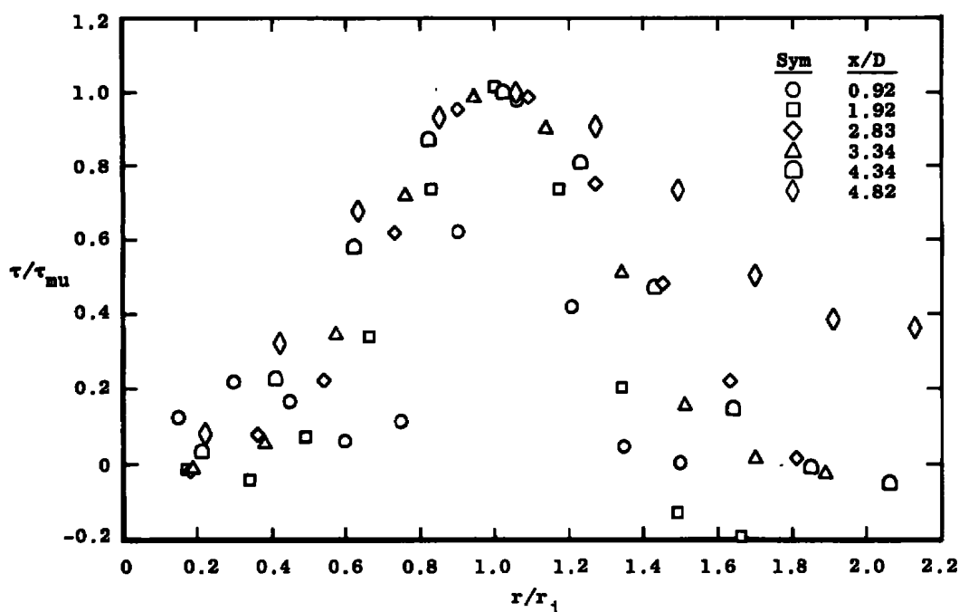
Figure 19. Radial distribution of shear stress, 3:1 velocity ratio, tripped.
