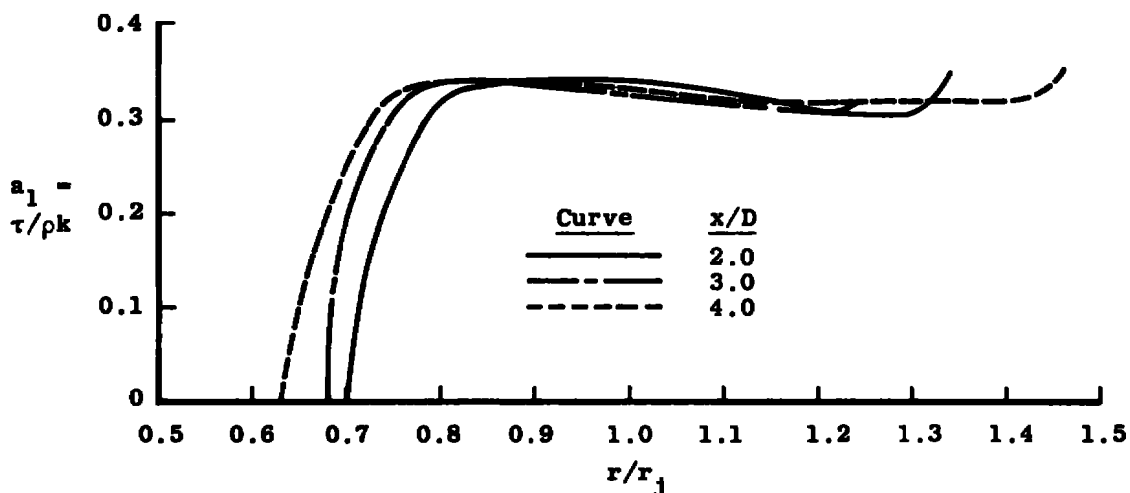
Figure 40. Implied distribution of a_1 , three-equation model, 3:1 velocity ratio, untripped.
