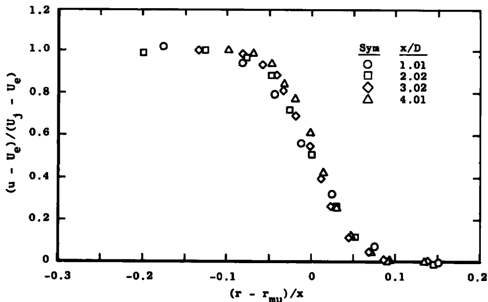
Figure 18. Velocity profiles plotted in two-dimensional shear layer similarity coordinates, 2:1 velocity ratio, untripped.
