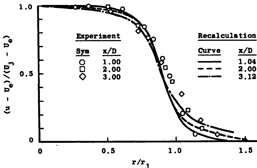
Figure 27. Results of data recalculation, 2:1 velocity ratio, tripped boundary-layer case.
