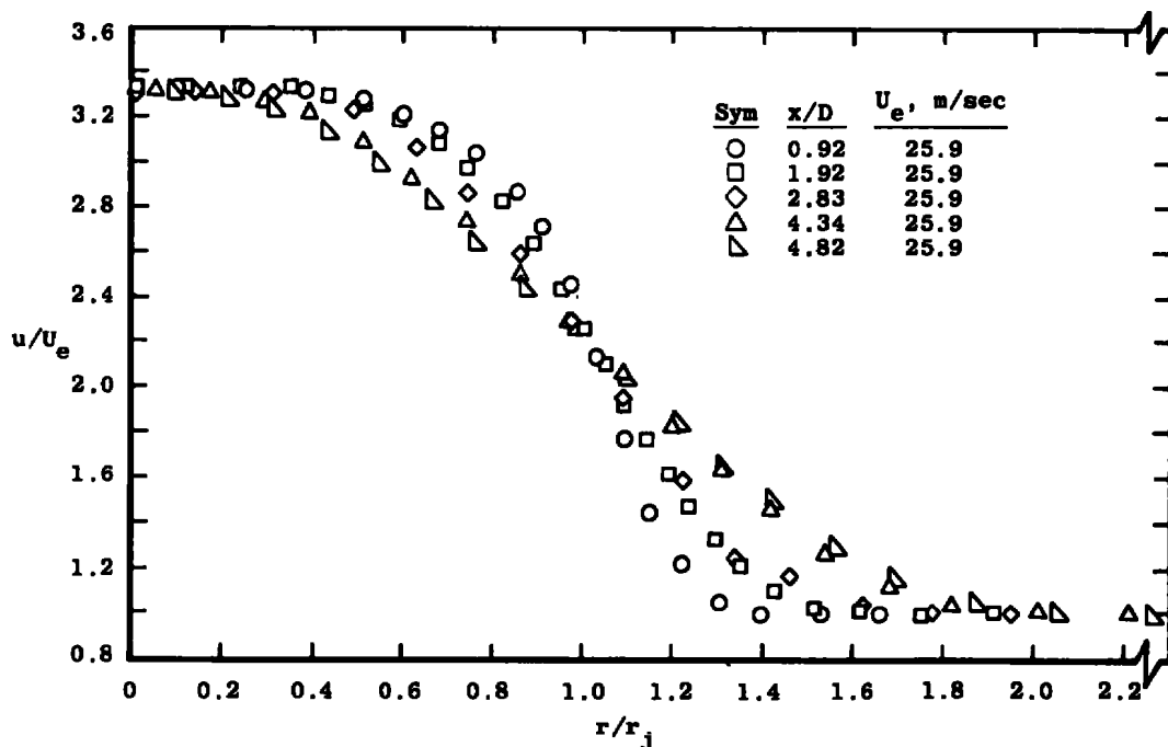
Figure 11. Mean velocity profiles, 3:1 velocity ratio, tripped, after edge velocity adjustment.
