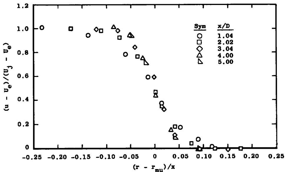
Figure 16. Velocity profiles plotted in two-dimensional shear layer similarity coordinates, 2:1 velocity ratio, tripped.
