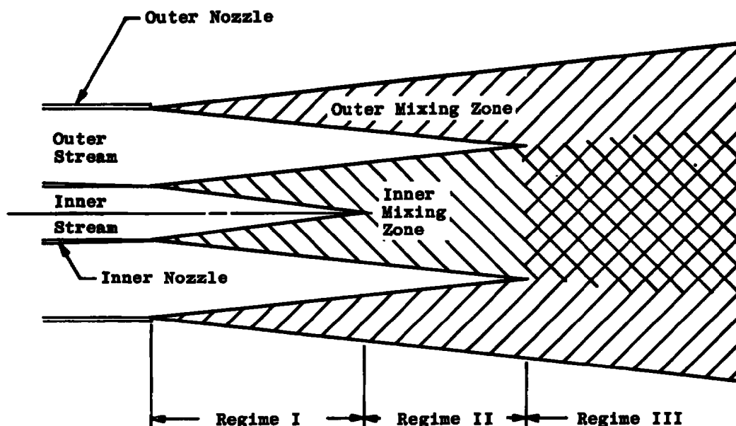
Figure 1. Mixing flow field.
