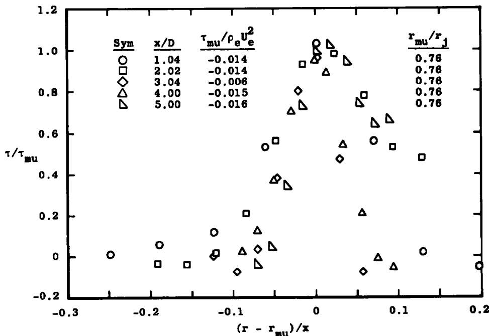
Figure 23. Turbulent shear stress in two-dimensional shear layer similarity coordinates, 2:1 velocity ratio, tripped.
