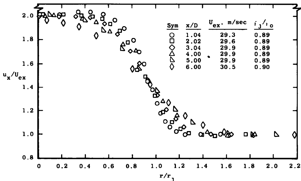
Figure 6. Mean velocity profiles, 2:1 velocity ratio, tripped.
