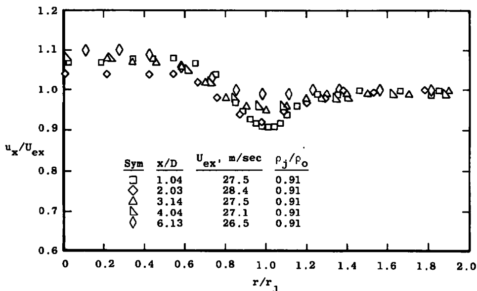
Figure 7. Mean velocity profiles, 1:1 velocity ratio, tripped.
