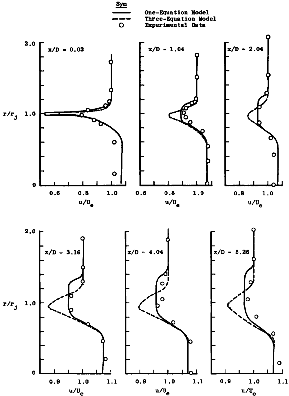
Figure 38. Comparison of prediction with experiment, 1:1 velocity ratio, tripped initial boundary layers.
