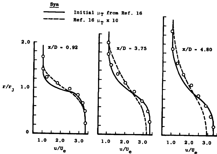
Figure 50. Effect of alteration of initial eddy viscosity profile, one-equation model, 3:1 velocity ratio, tripped.
