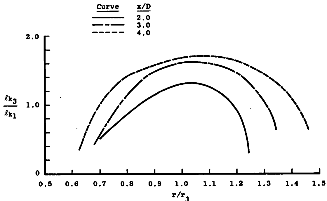
Figure 43. Implied distribution of turbulence length scale, 3:1 velocity ratio, untripped.
