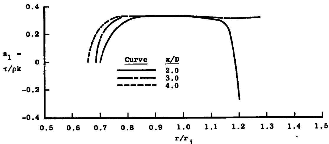
Figure 41. Implied distribution of a_1 , three-equation model, 2:1 velocity ratio, untripped.
