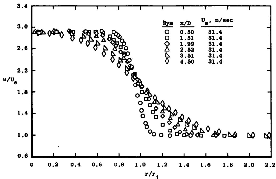
Figure 13. Mean velocity profiles, 3:1 velocity ratio, untripped, after edge velocity adjustment.
