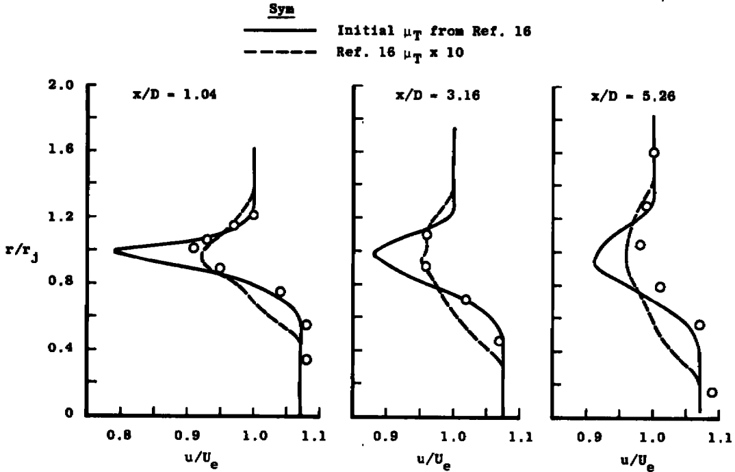
Figure 53. Effect of alteration of initial eddy viscosity profile, three-equation model, 1:1 velocity ratio, tripped.
