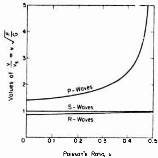
c. Relation between Poisson's ratio, \nu , and velocities of propagation of compression (P), shear (S), and Rayleigh (R) waves in a semi-infinite elastic medium
