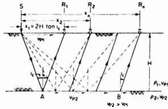
a. Direct and head wave paths (After Richart et al., 1970)
