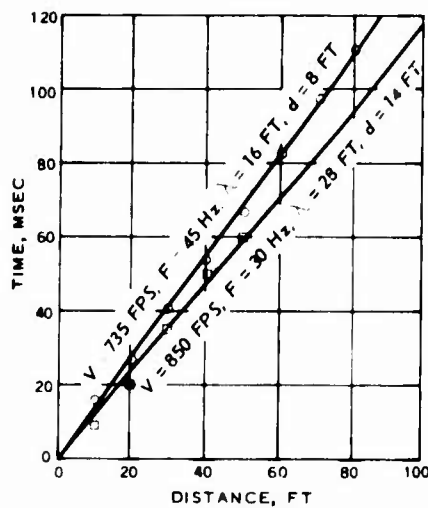
d. Rayleigh wave velocities from surface refraction seismic tests
