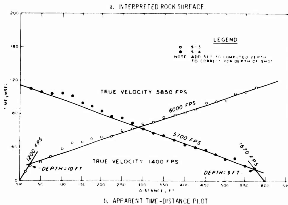
FIG. 4.--TIME-DELAY INTERPRETATION OF REFRACTION SEISMIC SURVEY
