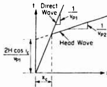
b. Apparent time-distance curves (After Richart et al., 1970)
