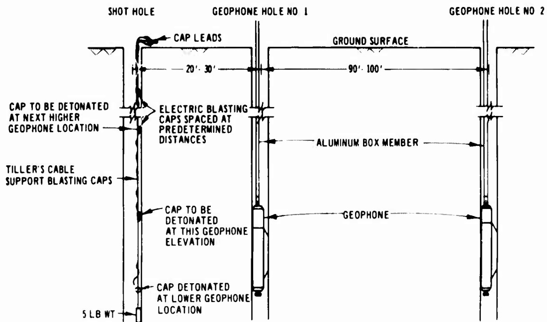
a. TYPICAL CROSSHOLE TEST LAYOUT
