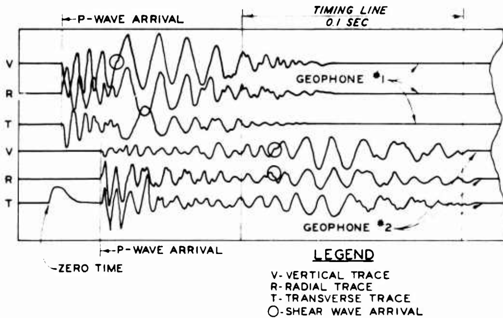
b. SAMPLE OSCILLOGRAPH RECORD FOR CROSSHOLE TESTS
