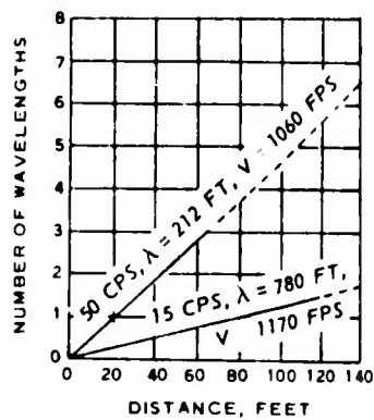
b. Number of waves versus distance plot
