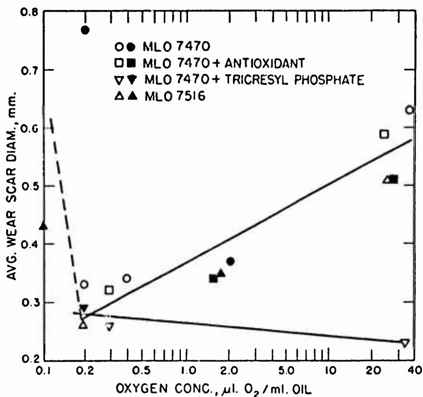
Figure 99. EFFECT OF DISSOLVED OXYGEN ON WEAR BEHAVIOR
