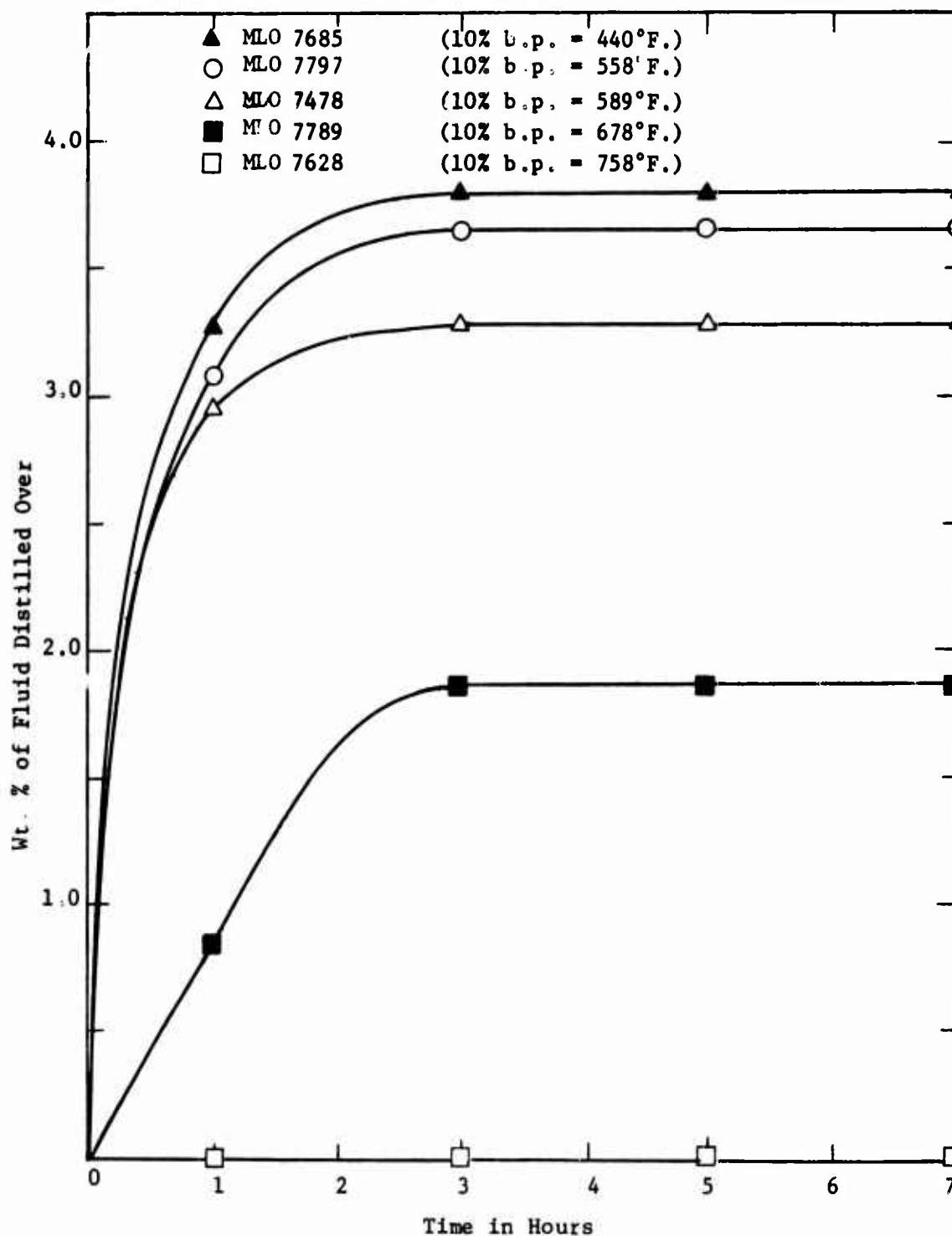
Figure 15. Volatility of Test Fluids
