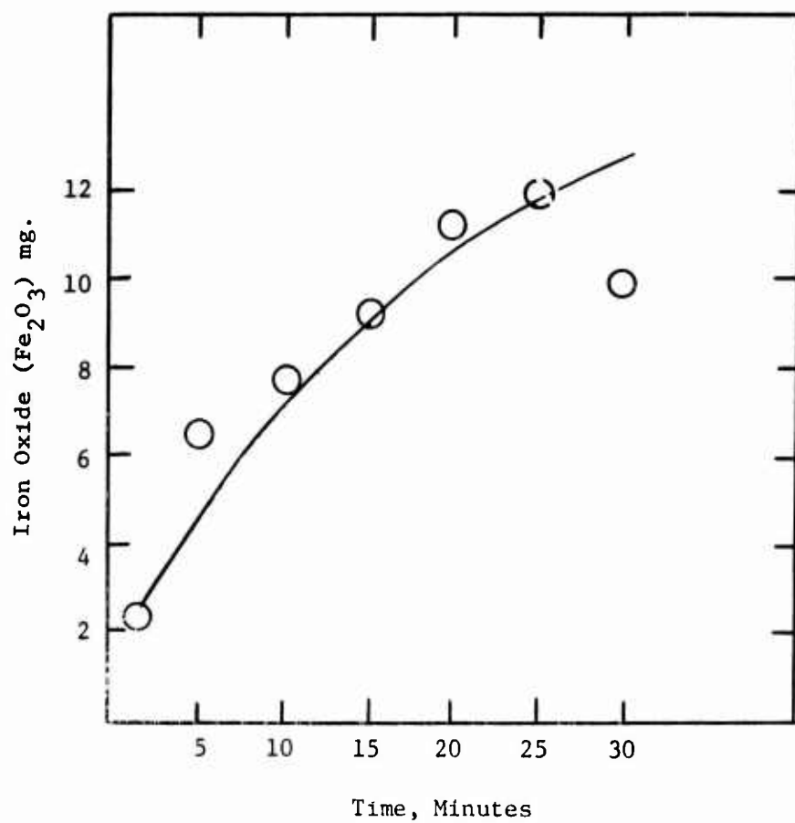
Figure 75. RATE OF DISSOLUTION OF IRON OXIDE ( \text{Fe}_2\text{O}_3 ) IN ACRIDINE-INHIBITED HYDROCHLORIC ACID SOLUTION
