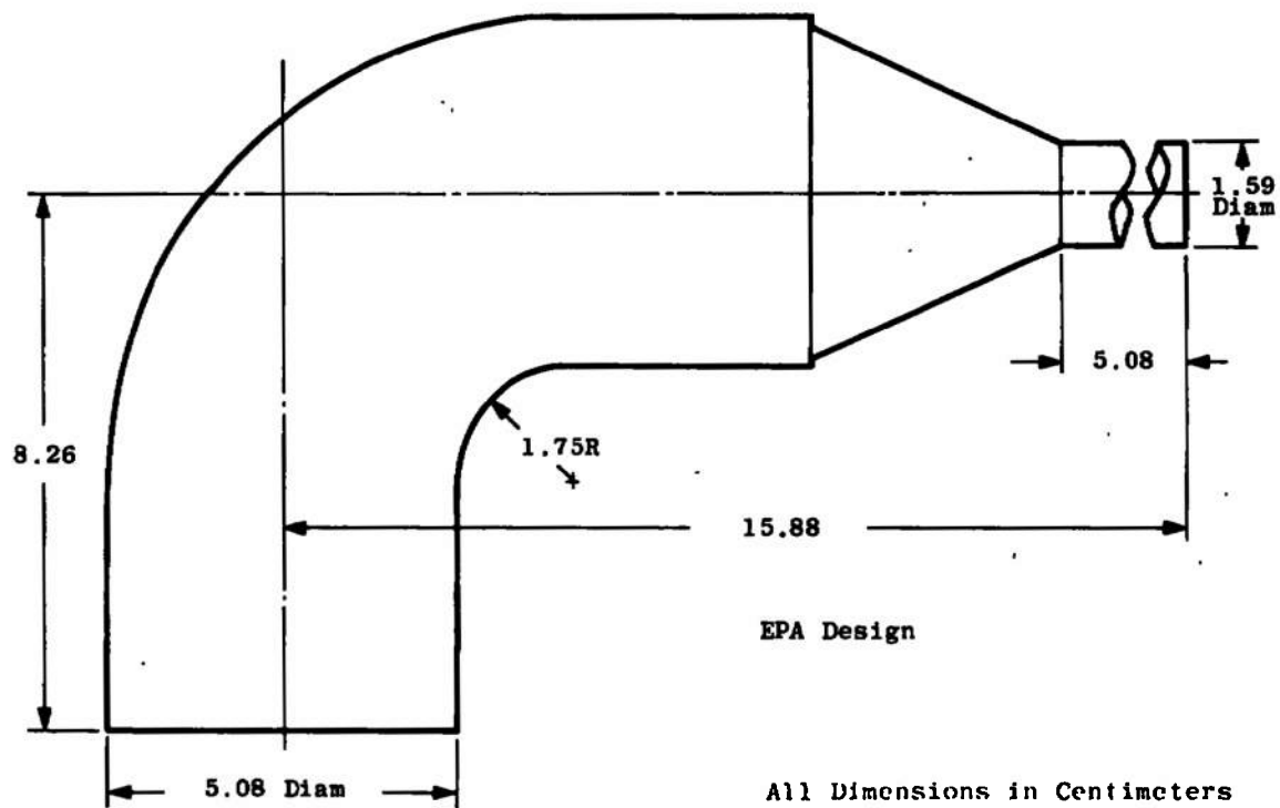
Figure 13. 5.08-cm sampling probe (square-edge).
