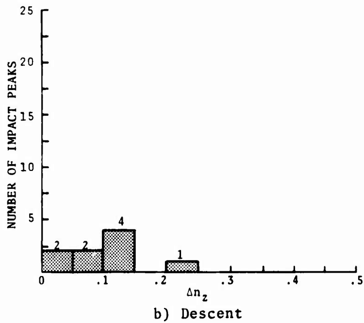
Figure 23. UH-1H Utility Landing Impact Peaks.
