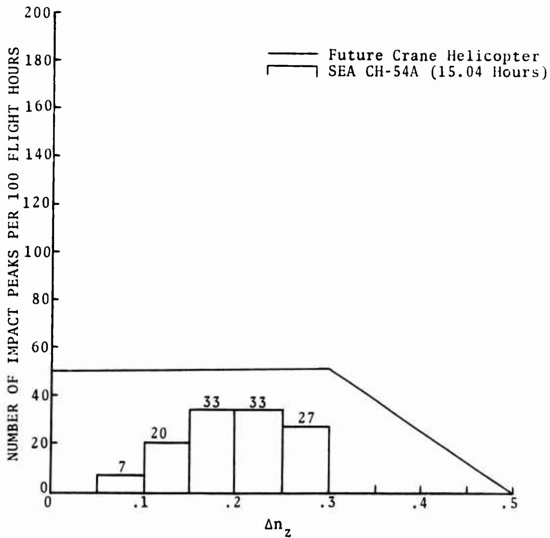
Figure 34. Landing Impact Peak Distribution of the Operational and Future Mission Profiles for the Crane Helicopter.
