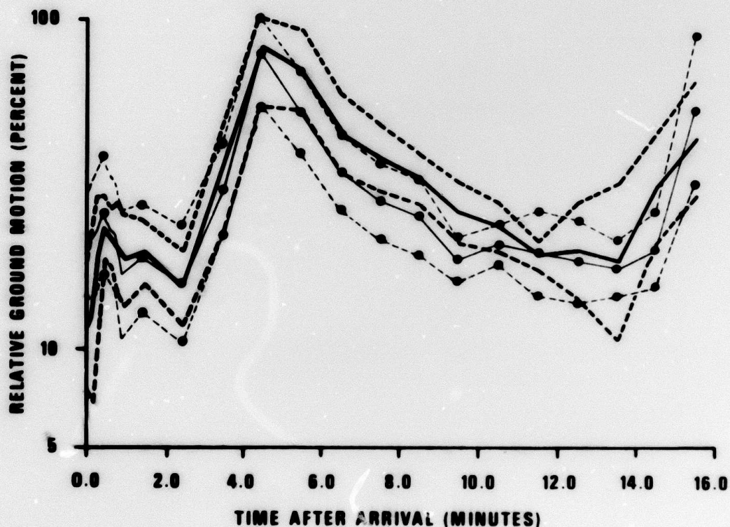
Figure AI-2. Comparison of large-event and small-event coda averages, 105-110°.
