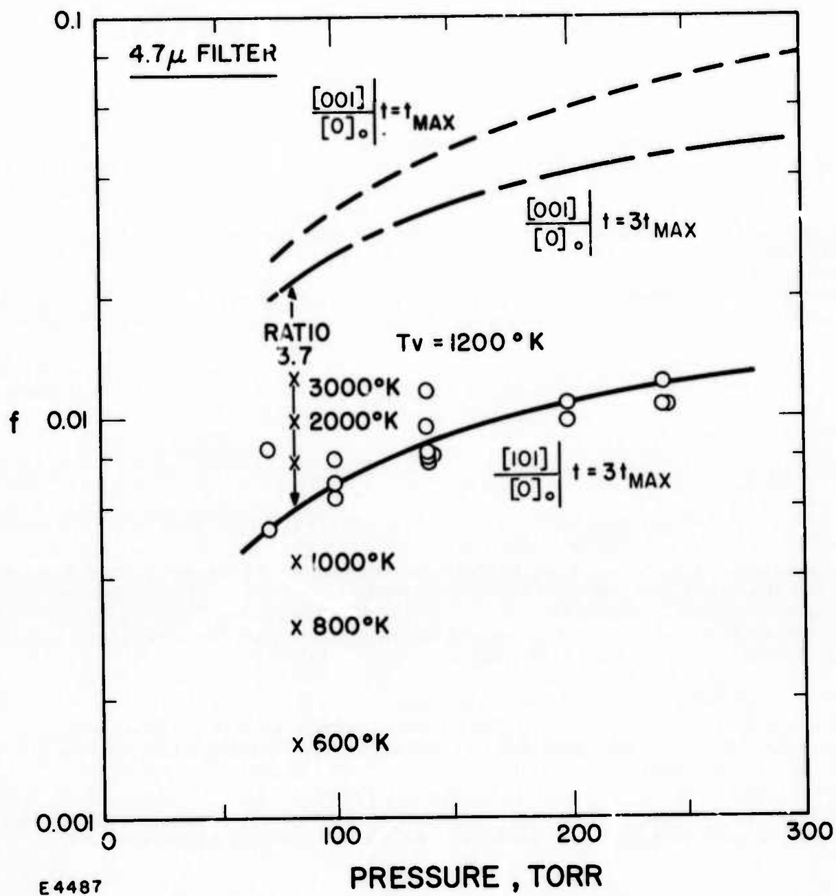
Fig. 5 Reduced data for [101]/[O]_e at t = 3t_{max} are shown vs total pressure. Solid line is our fit to this data. Dashed line represents our earlier data for [001]/[O]_e at t = t_{max} , and broken line is this earlier data theoretically scaled to t = 3t_{max} . Ratio of broken to solid line implies a T_v \approx 1200^\circ K .
