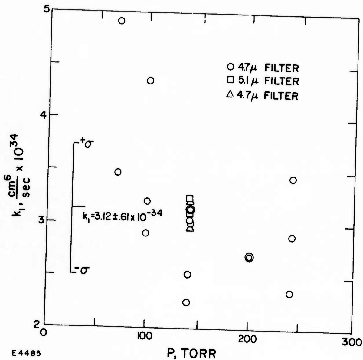
Fig. 3 Recombination Rate Data vs Total Pressure for \text{O} + \text{O}_2 + \text{O}_2 \rightarrow \text{O}_3 + \text{O}_2 Obtained from Data such as Shown in Figs. 2 and 6 and Using the 4.7 and 5.1 \mu Filters in Series
