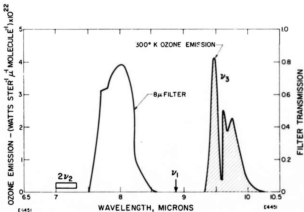
Fig. 7 Spectral Transmission of 8\mu Filter used to Look for \nu_1 and \nu_3 Vibration-Rotation Transitions of the ^3B_2 State. Their predicted positions are indicated. A 300^\circ\text{K} emission spectrum due to the ground state \nu_3 -band is also shown for comparison. The \nu_1 band has a peak value of 2.5 \times 10^{-24} watts ster ^{-1} \mu^{-1} molecule ^{-1} at the location indicated. The location of the 2\nu_2 band is also shown.
