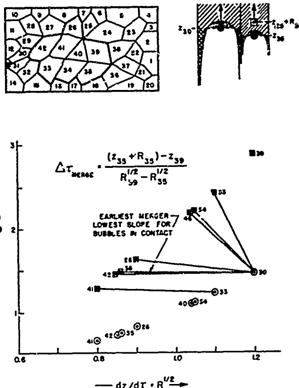
Fig. 3. Factors governing bubble merger in idealized model. Upper left: Representative bubble pattern as viewed from above. The cross sectional area associated with one bubble in this diagram is identified with \pi R^2 to define the effective radius R . Upper right: Bubble or finger No. 39 is idealized as engulfing finger No. 35 as soon as the effective height z_{39} of the larger one exceeds the effective height of the smaller one by the radius of the smaller one; that is, as soon as z_{39} (point \square ) comes to equality with z_{35} + R_{35} (point \square ). The arrows recall that the rate of rise of the larger bubble is greater than the rate of rise of the smaller finger, as is required for capture of the smaller one: dz/dt = 0.48 (gR)^{1/2} . Instead of the true time t it is convenient to use the "reduced time", \tau = 0.48 g^{1/2} t , so that the rate of rise becomes dz/d\tau = R . Lower diagram: Graphical procedure to determine which pair of bubbles merge first. For simplicity, attention is limited to the system of eight fingers outlined by a heavy line in the upper left hand diagram. The calculated value of the reduced time interval \Delta\tau required for No. 39 to capture No. 35 is determined by the slope (with sign reversed) of the designated line in the diagram. The line from No. 39 to No. 42 is irrelevant because it corresponds to two bubbles which are not in contact. For fingers in contact, the line with the lowest slope corresponds to the earliest merger. A new diagram of this type was constructed for each successive stage in the process of bubble merger in the process of working out the illustrative numbers in Table V.
