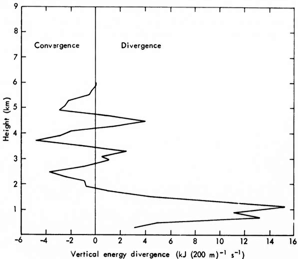
Fig. 24—Average vertical divergence per slab of static energy (KJ (200 m) -1 s -1 ), Cloud B
