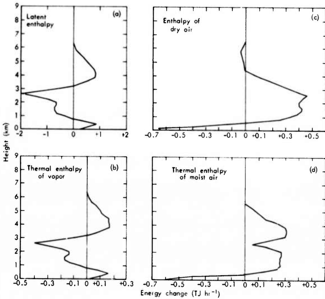
Fig. 8—Change from 0 to 60 min of energy summed by slabs (TJ hr -1 ), Cloud A
