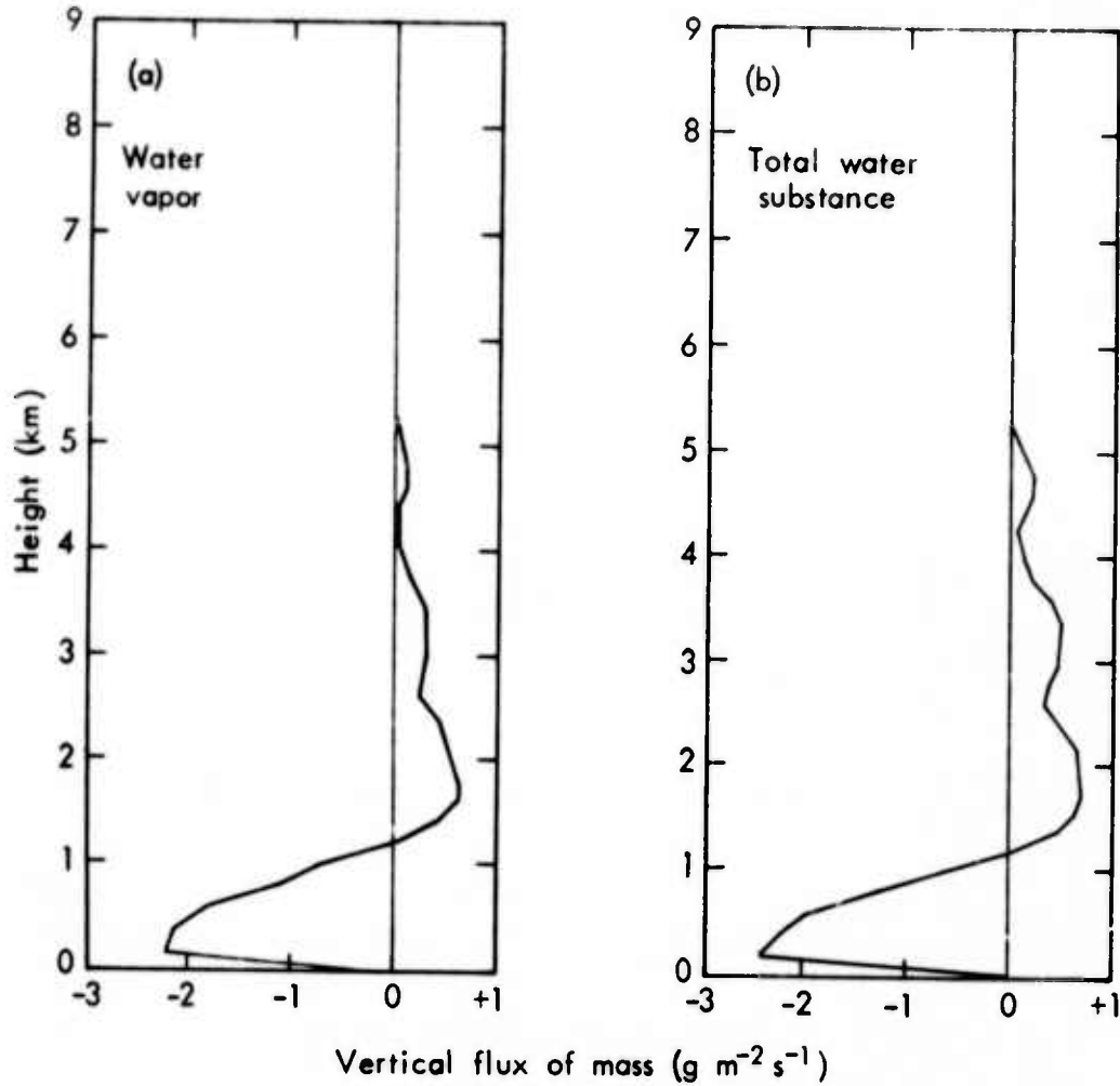
Fig. 23—Average vertical flux summed by slabs (g m -2 s -1 ), Cloud B
