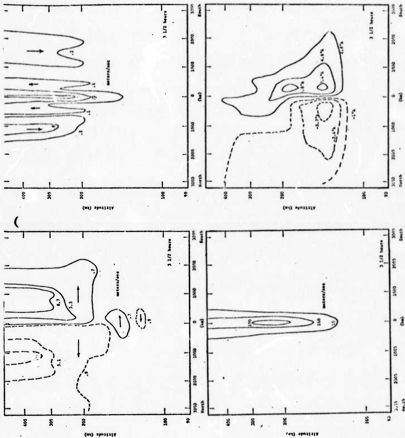
Figure 7. Wind profiles generated by auroral zone electric field.
