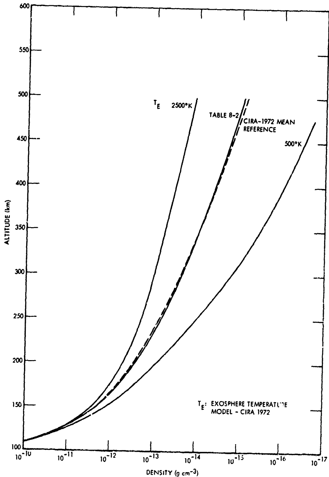
Figure 8-2. Density versus altitude for extremes of CIRA 1972 atmospheric models and for the CIRA 1972 mean and CIRA 1965 Model 5, 8 hour.
