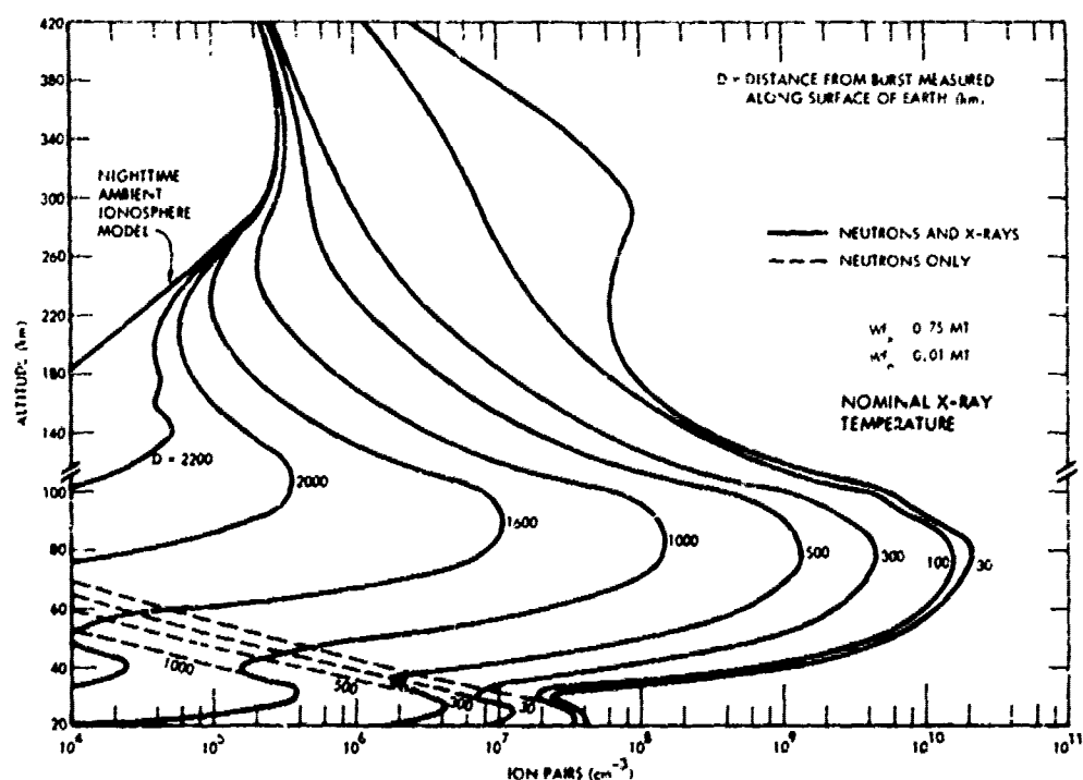
Figure 2-16. Ion-pair density at t = 0 due to X-rays and neutrons, burst at 300 km.
