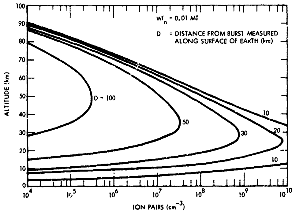
Figure 2-18. Ion-pair density at t = 0 due to neutrons, burst at 20 km.
