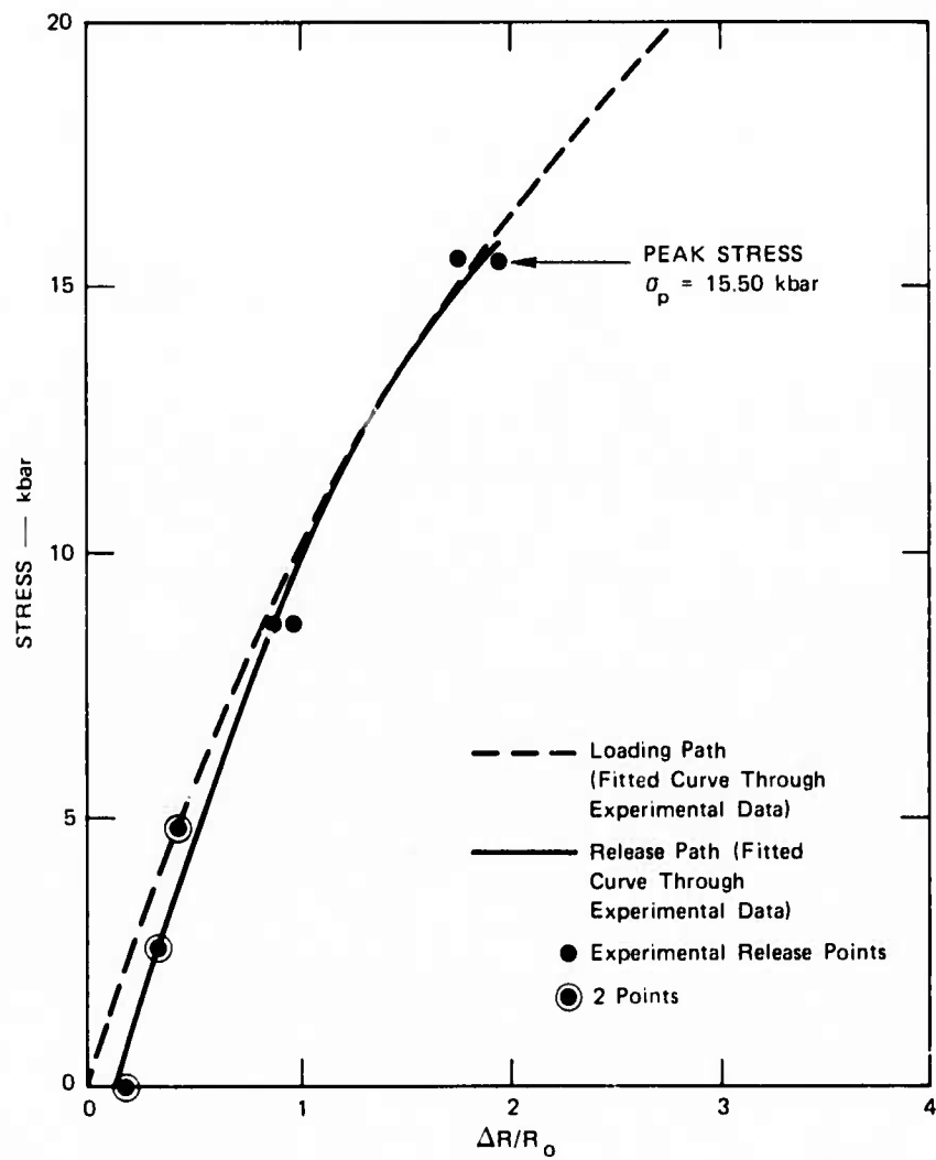
FIGURE 28 LOADING AND RELEASE PATHS, SHOT S18
