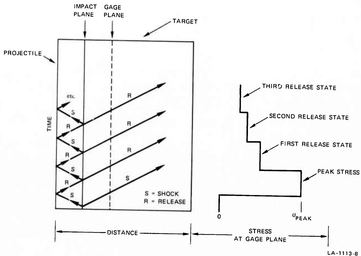
FIGURE 7 SCHEMATIC DIAGRAM OF WAVE BEHAVIOR IN STEP-RELEASE EXPERIMENT AND EXPECTED GAGE RECORD
