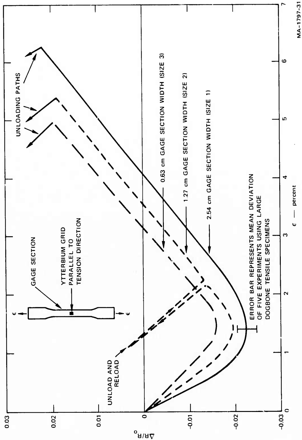
FIGURE 47 FRACTIONAL CHANGE IN RESISTANCE VERSUS TENSILE STRAIN
