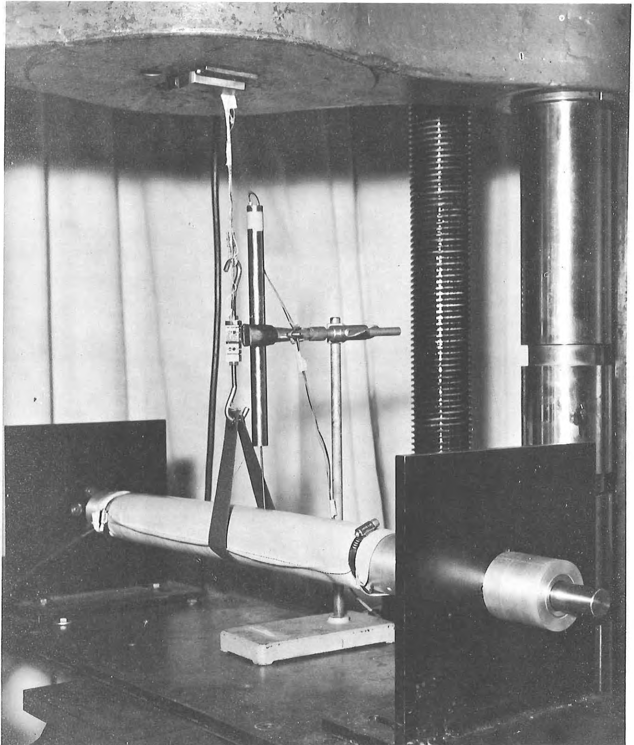
Figure 3. Beam Bending Test Apparatus
