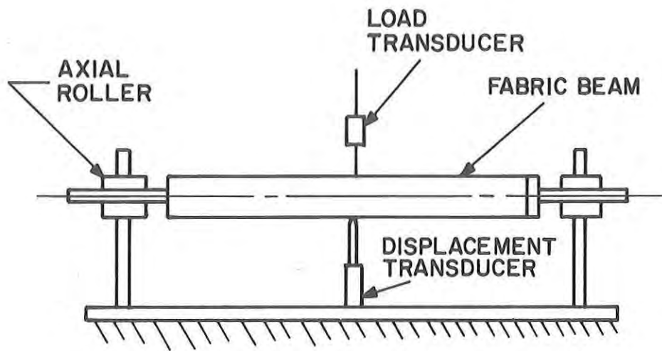
Figure 2. Schematic Diagram of Experimental Apparatus
