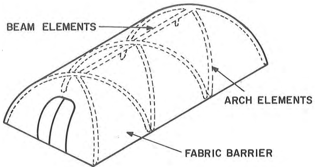
Figure 1. Tent Concept Using Pressure Stabilized Structural Elements
