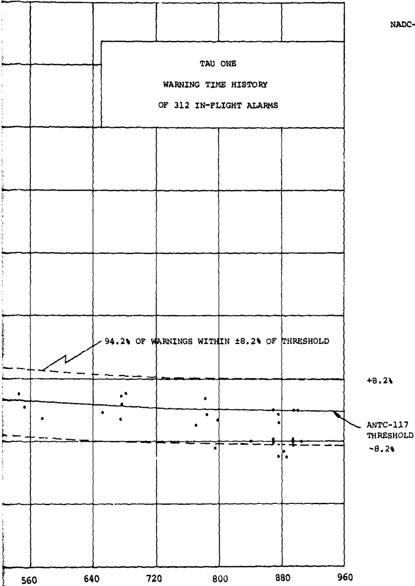
Figure VII-12. Warning Time History of 312 Tau One Alarms.
