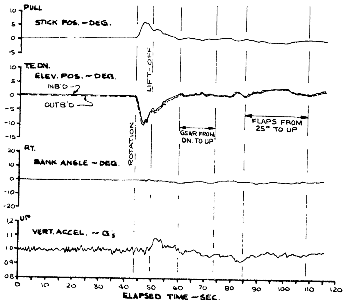
FIGURE NO. 1C(3.2.3.3) TAKE-OFF ASSESSMENT
