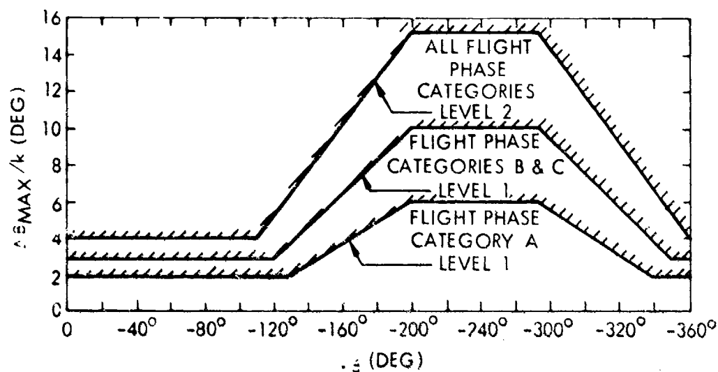
Figure 6. Sideslip Excursion Limitations
