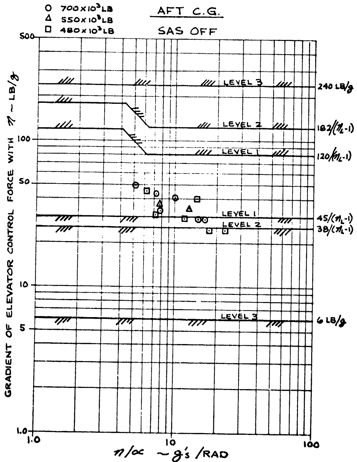
FIGURE NO.2(3.22.2.1) ELEVATOR CONTROL FORCE GRADIENT SUMMARY
