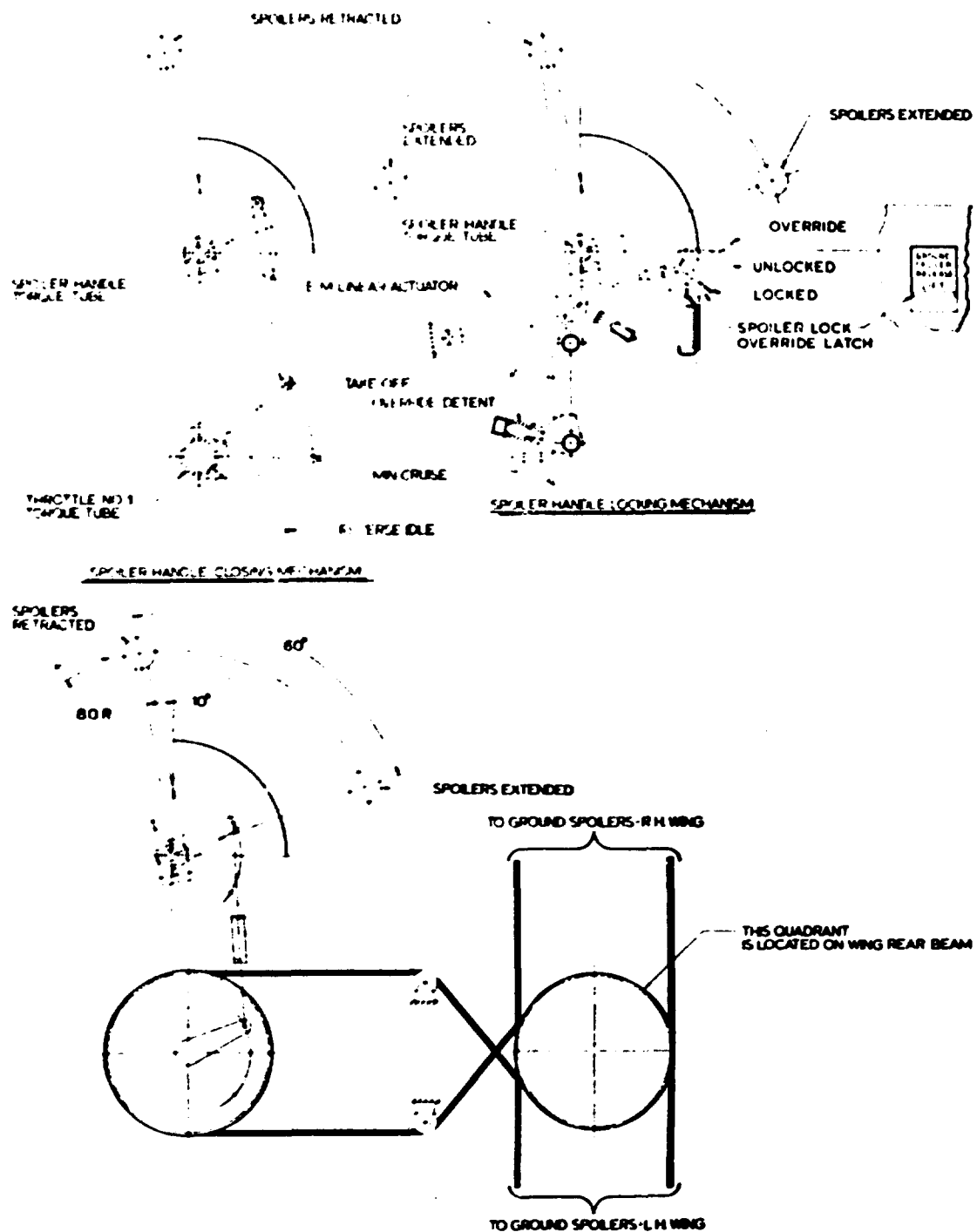
Figure 14(2.0). Ground Spoiler Control System
