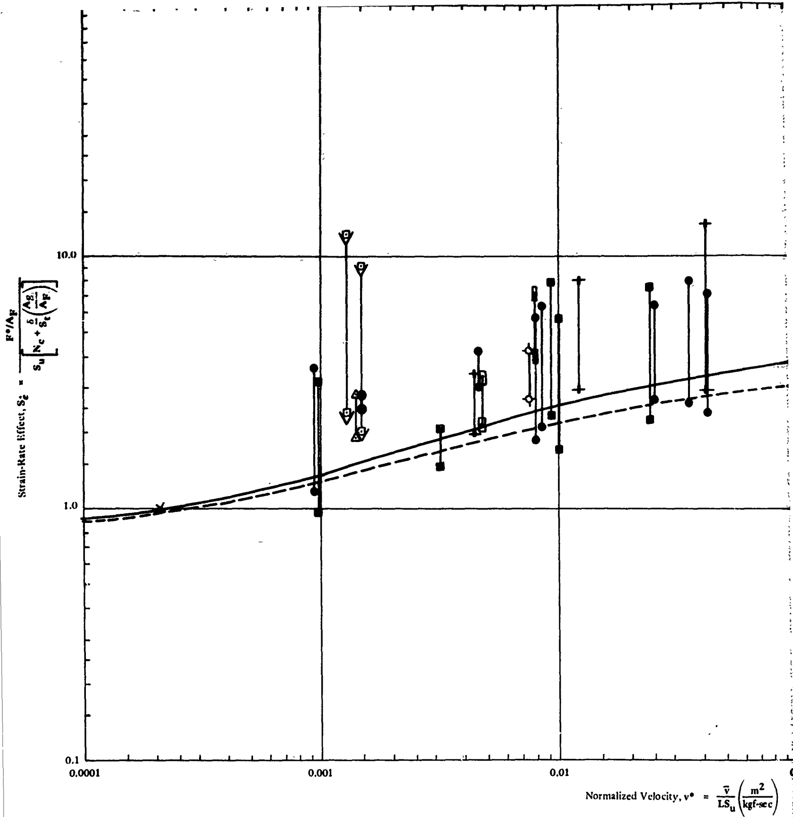
Figure 23. Strain-rate effect versus normalized velocity for silt and clay
