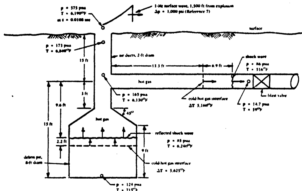
Figure 12. Typical computed results—Lagrange code, 0.0108 second after arrival of shock wave from 1-Mt nuclear explosion.
