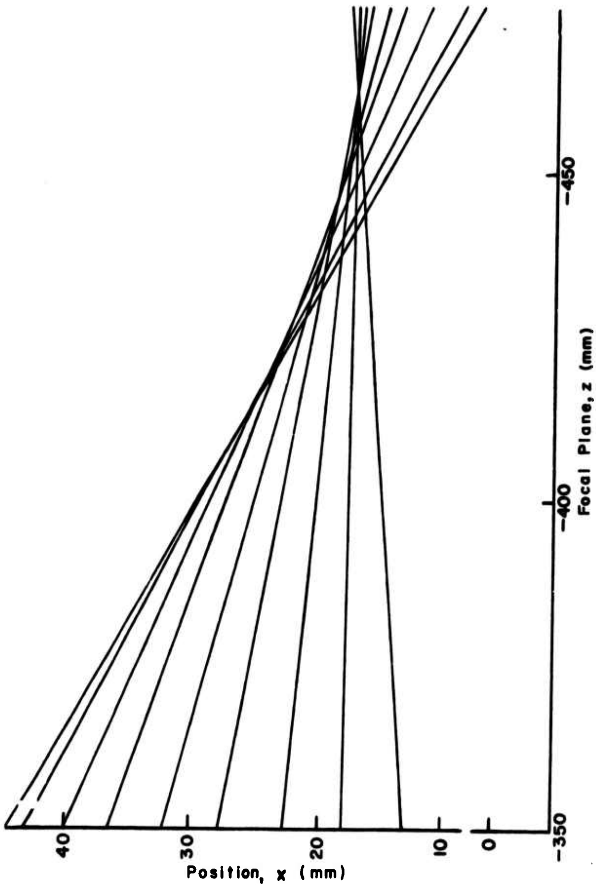
Figure 29. Theoretical Meridional Ray Fan Graph for Lens C at \lambda = 568.2 \text{ nm}
