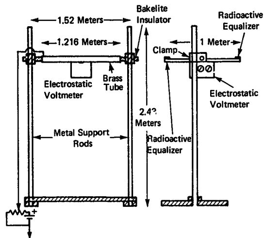
Fig. 7 Support Stand for Electrostatic Voltmeter
