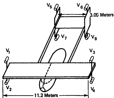
Fig. 8 Position of Atmospheric Potential Field Sensors on Cessna 337 Airplane
