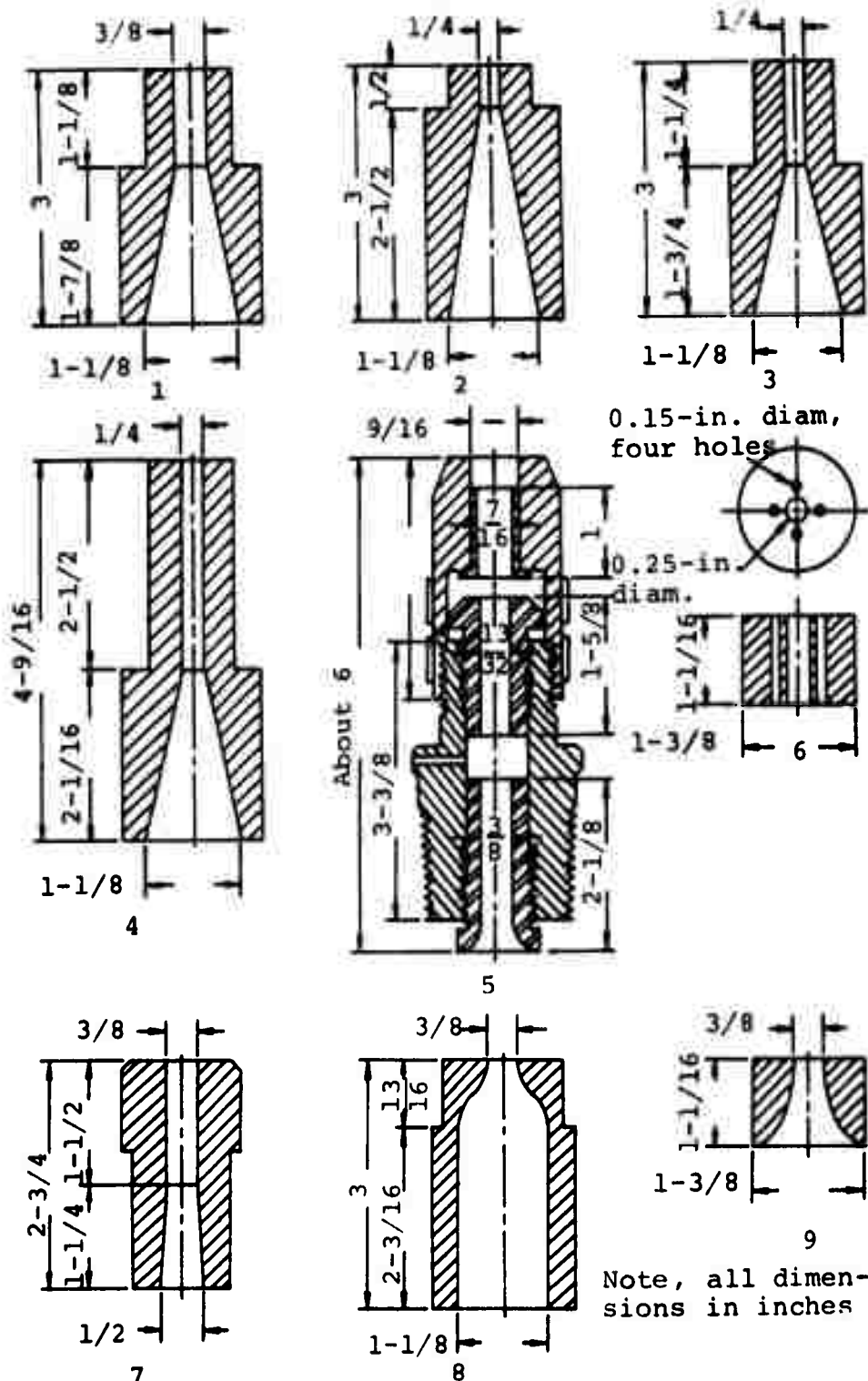
Figure 71. Various types of nozzles used by the U.S. Bureau of Mines (after Ref. 47).
