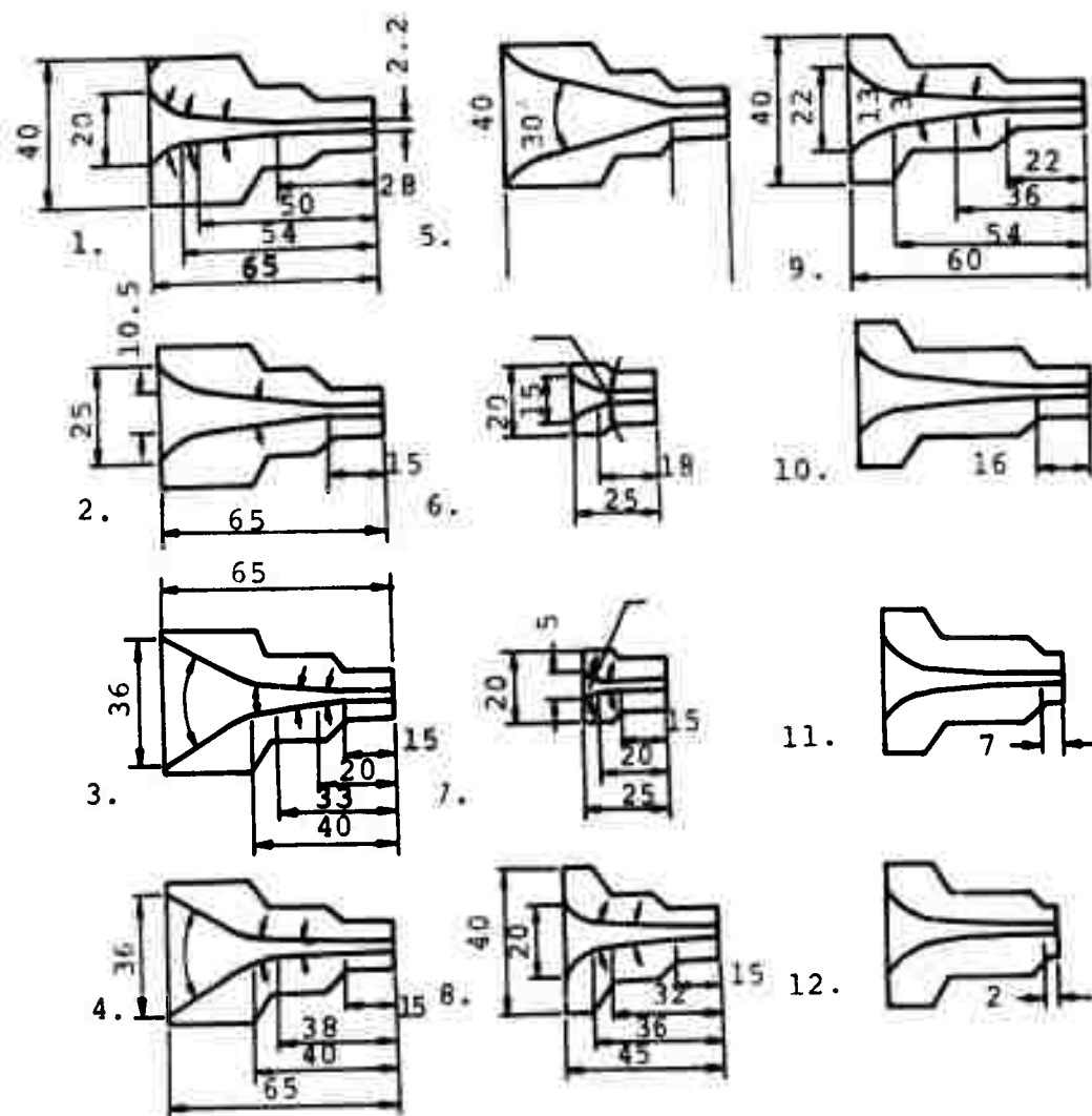
Figure 61. Profiles of experimental nozzles (after Ref. 42).
