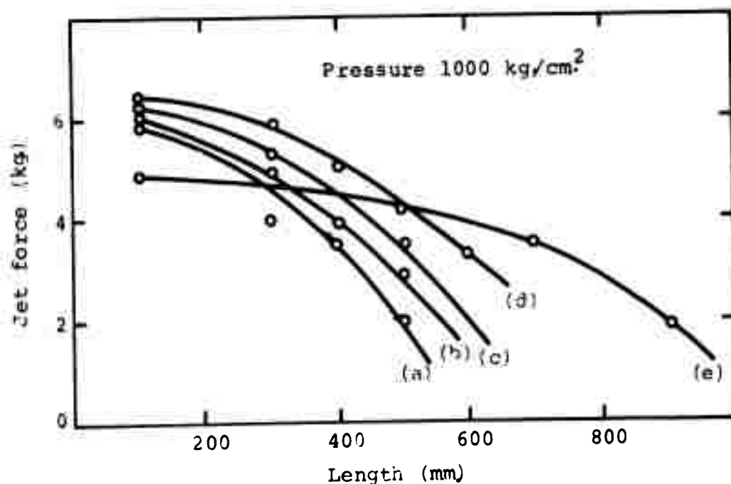
Figure 94(a). Jet force variation with standoff distance (after Ref. 40).
