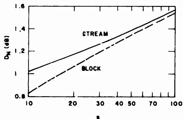
Fig. 7 — Degradation of word error rate as a function of n for a noncoherent system with P_w = 10^{-4} and k = 10 .
