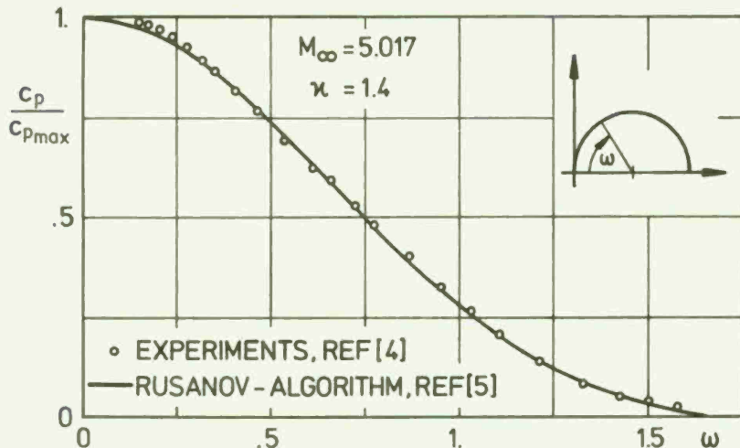
Fig. 1 Surface pressure distribution on a sphere
