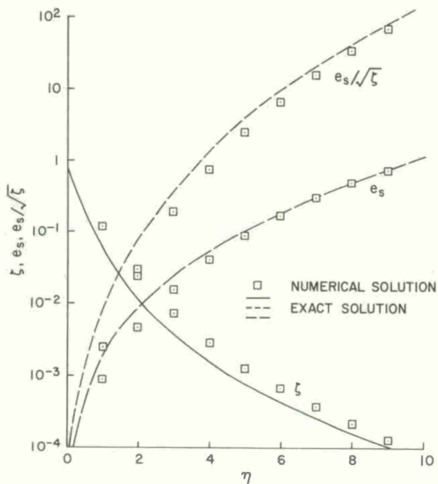
Fig. 5 Simplified turbulence model (basic method).
