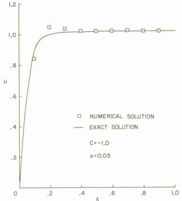
Fig. 3 Linear viscous equation (basic method).
