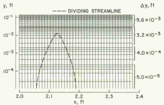
Fig. 18 Computational mesh.
