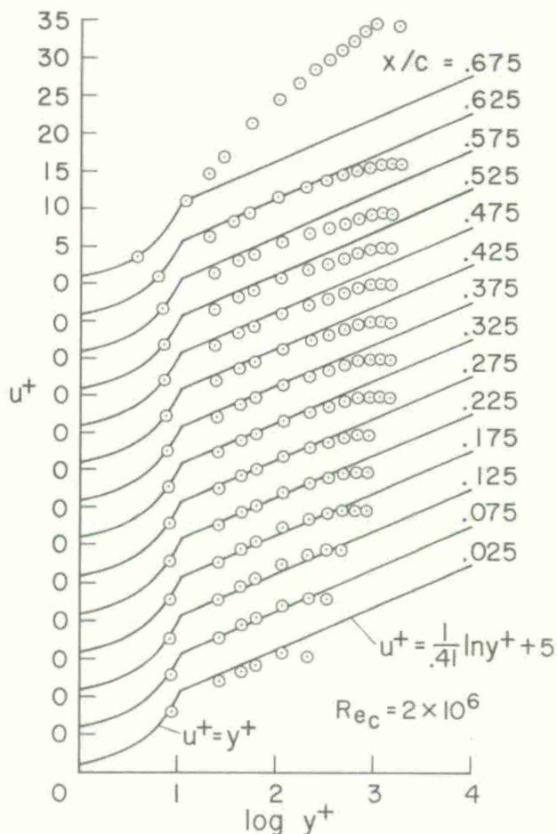
Fig. 12 Velocity profiles ahead of shock.
