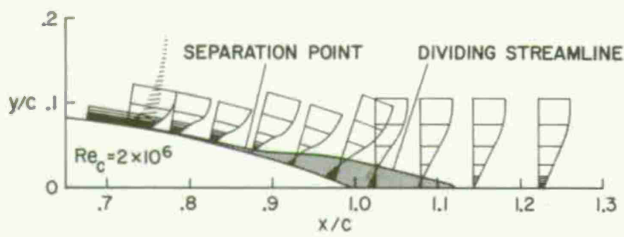
Fig. 13 Separation velocity profiles on 18-percent circular arc ( M_\infty = 0.775 ).
