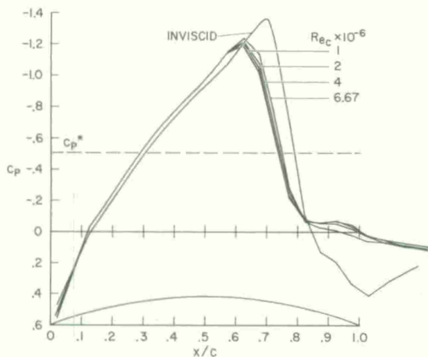
Fig. 9 Pressure distribution over 18-percent circular arc ( M_\infty = 0.775 ).
