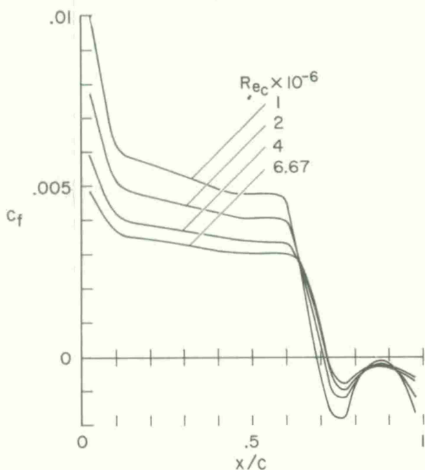
Fig. 10 Skin-friction distribution over 18-percent circular arc ( M_\infty = 0.775 ).
