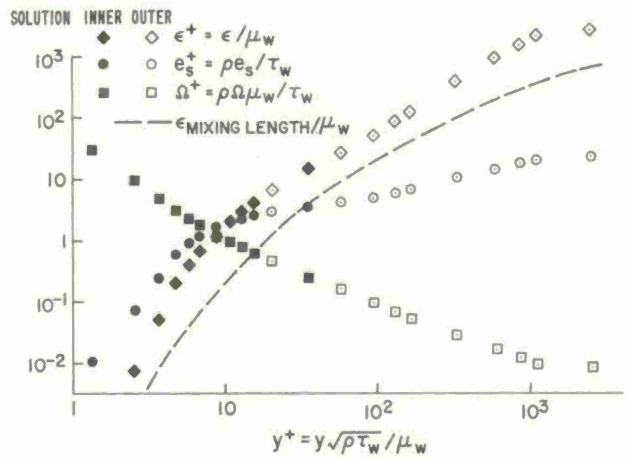
Fig. 29 Turbulence model variations aft of reattachment.
