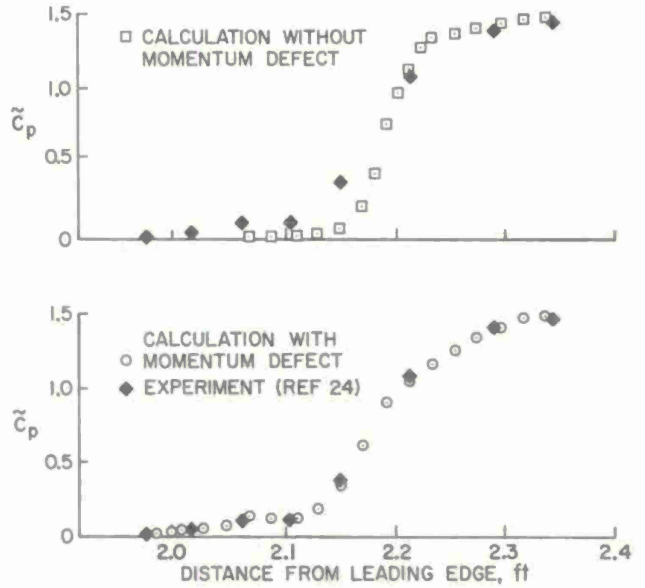
Fig. 24 Pressure distributions.
