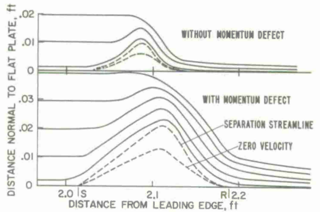
Fig. 25 Computed streamlines.
