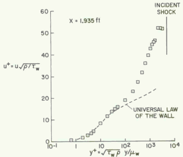
Fig. 19 Velocity profile ahead of interaction.
