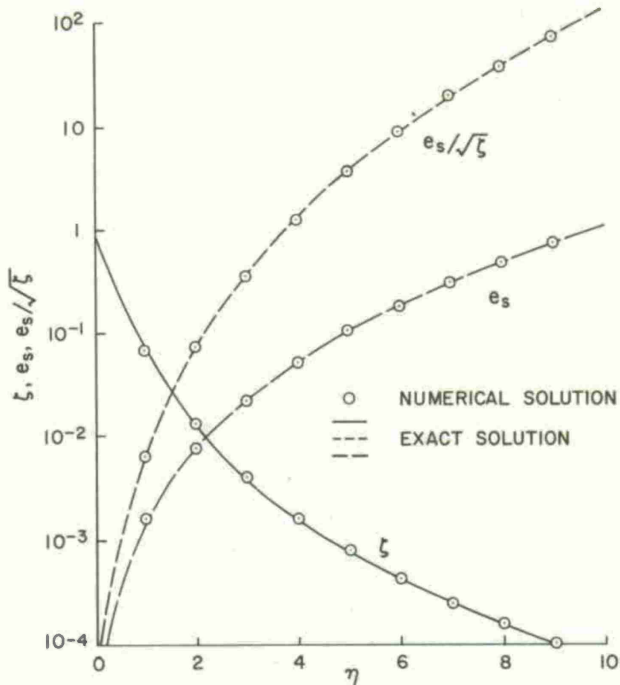
Fig. 6 Simplified turbulence model (exponential accuracy).
