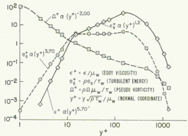
Fig. 20 Turbulence model variations ahead of interaction.
