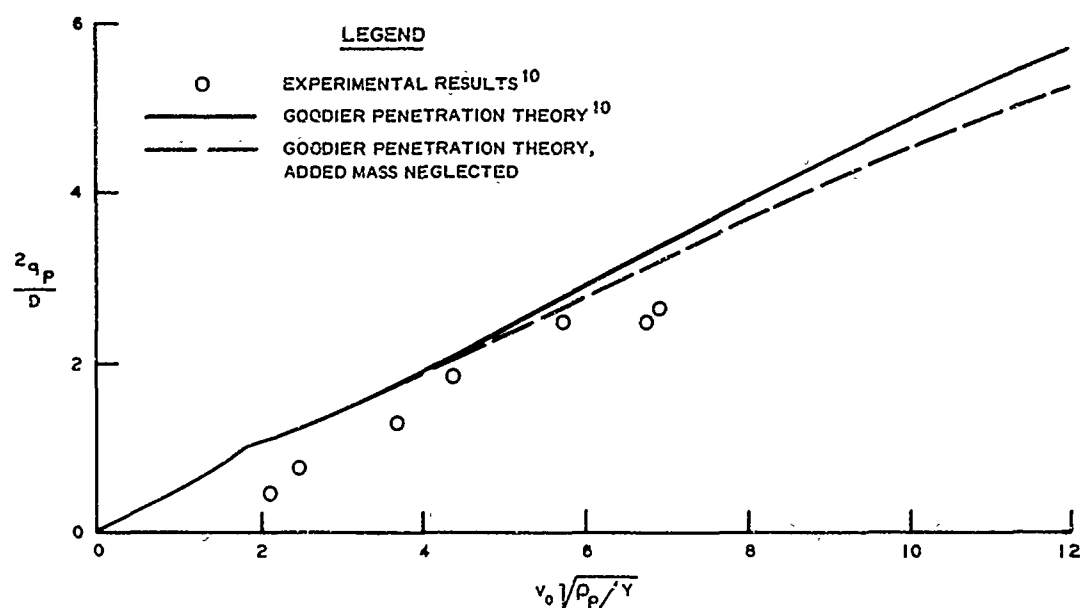
Figure C1. Penetration of aluminum target (AL 2024 T3) by lead spheres, R_a = 0.16
