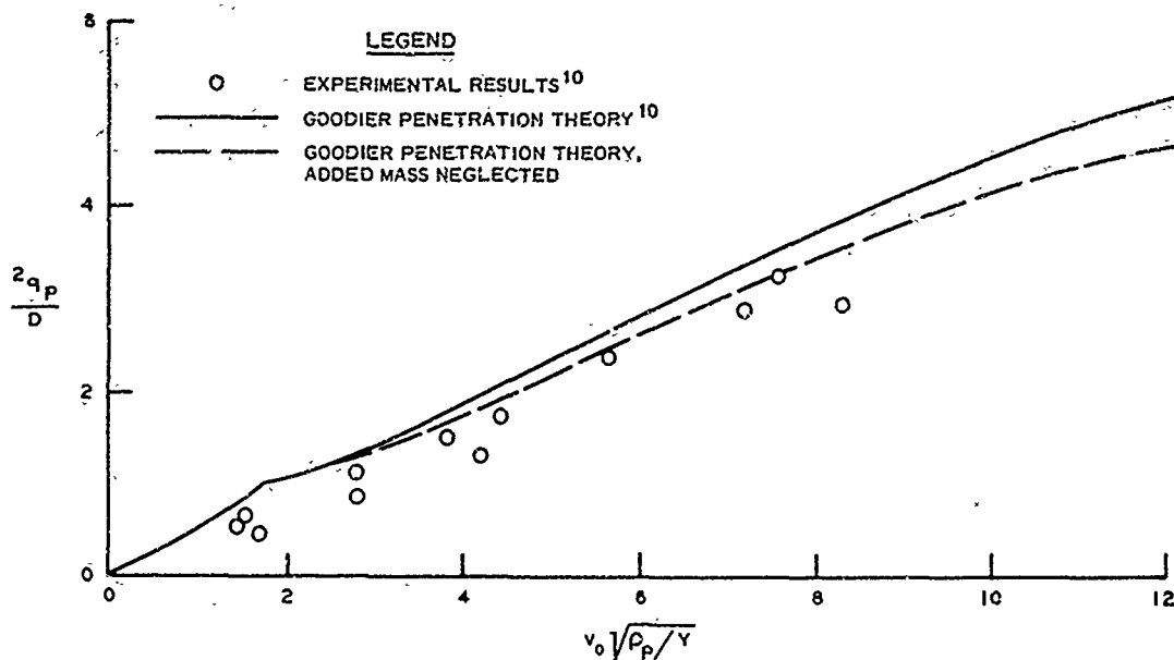
Figure C3. Penetration of aluminum target (AL 2024 T3) by steel spheres, R_a = 0.25
