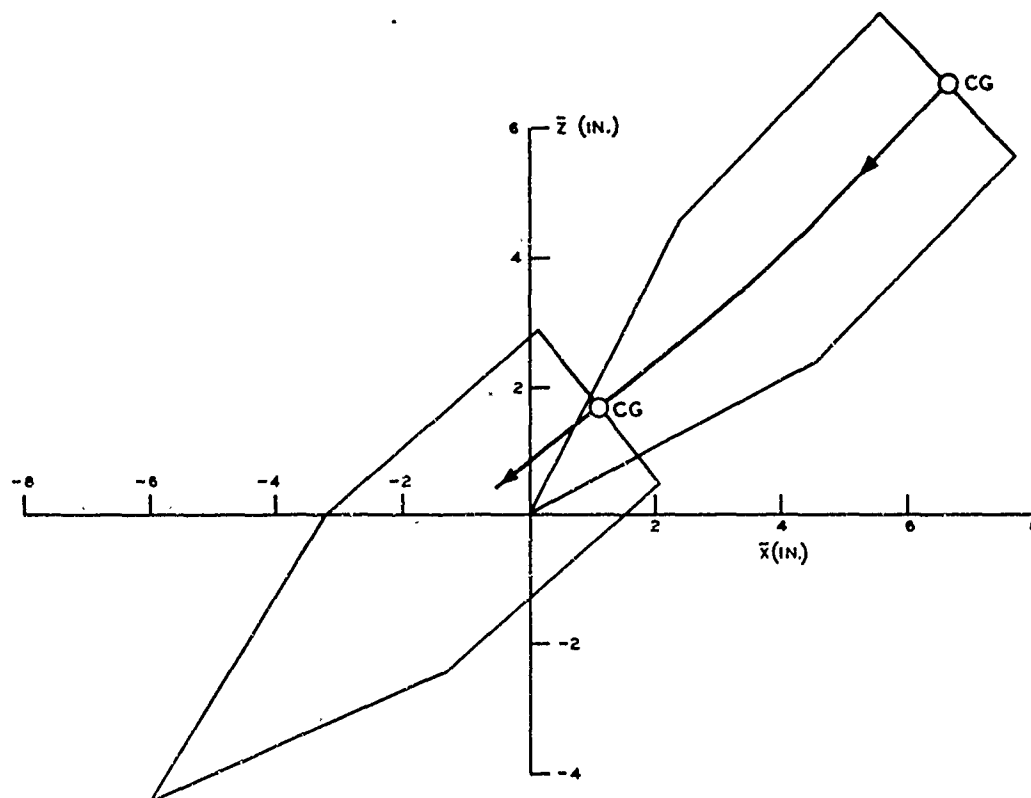
Figure 28. Oblique impact of TDV against hard earth for \omega_o = 45 \text{ deg} and v_o = 600 \text{ fps}
