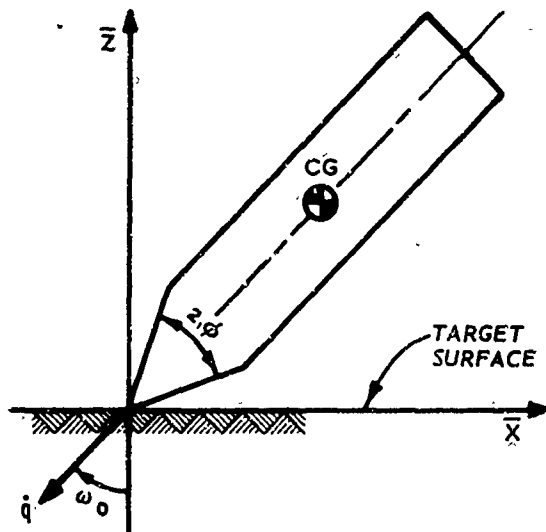
Figure 8. Oblique impact of a projectile with a conical nose
