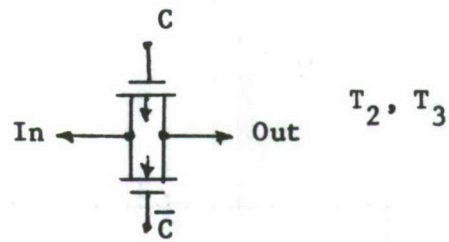
Figure 8. CMOS Inverter
