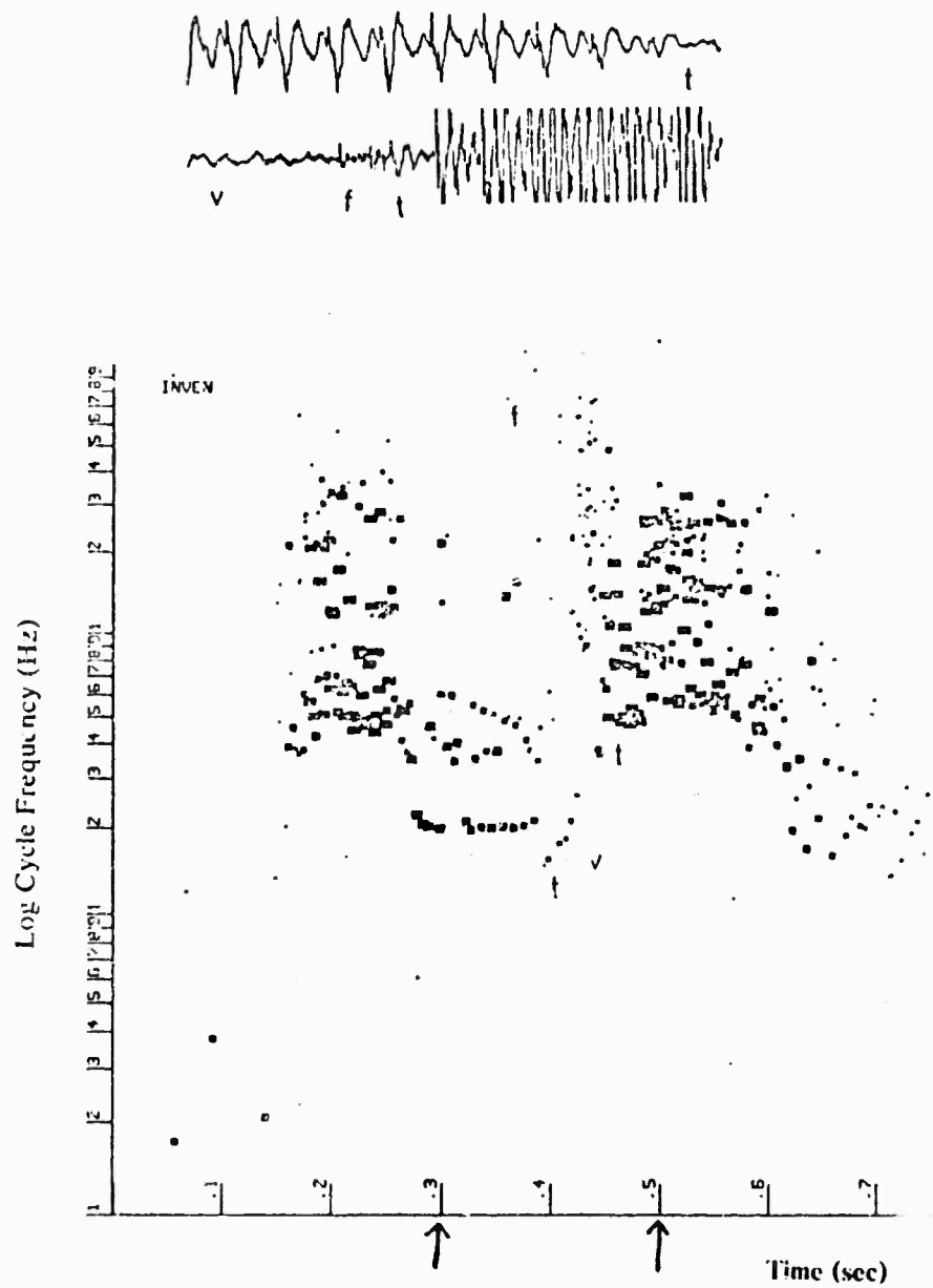
Figure 3: \text{invent}(\sigma, EH)
