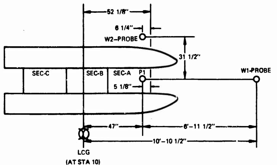
RIGID CROSS-STRUCTURE MODEL (1/4" scale):
