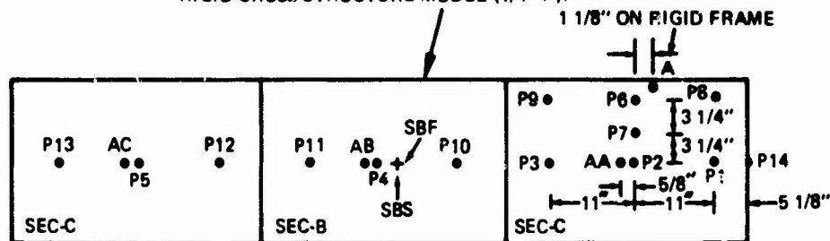
RIGID CROSS-STRUCTURE MODEL (1/4" scale):
