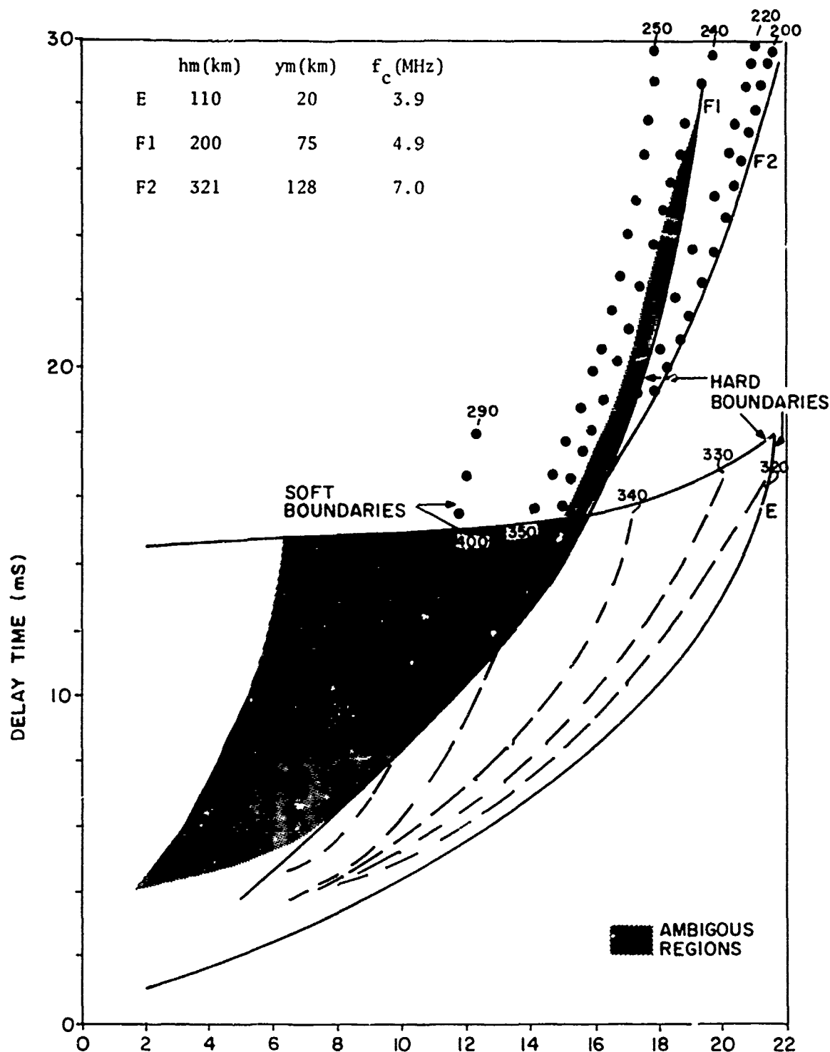
Figure 2-8. Ambiguous Regions Established by Hard and Soft Mode Boundaries Antennas with little gain near the horizon will produce a soft boundary at, for example, the longer time delay boundary of the E layer mode-observable region. This effect was not considered in making this diagram, so this boundary is indicated to be a hard one.
